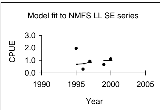
Figure 43. WinBUGS SSSPM fits to the individual CPUE series of the baseline scenario for sandbar shark.
