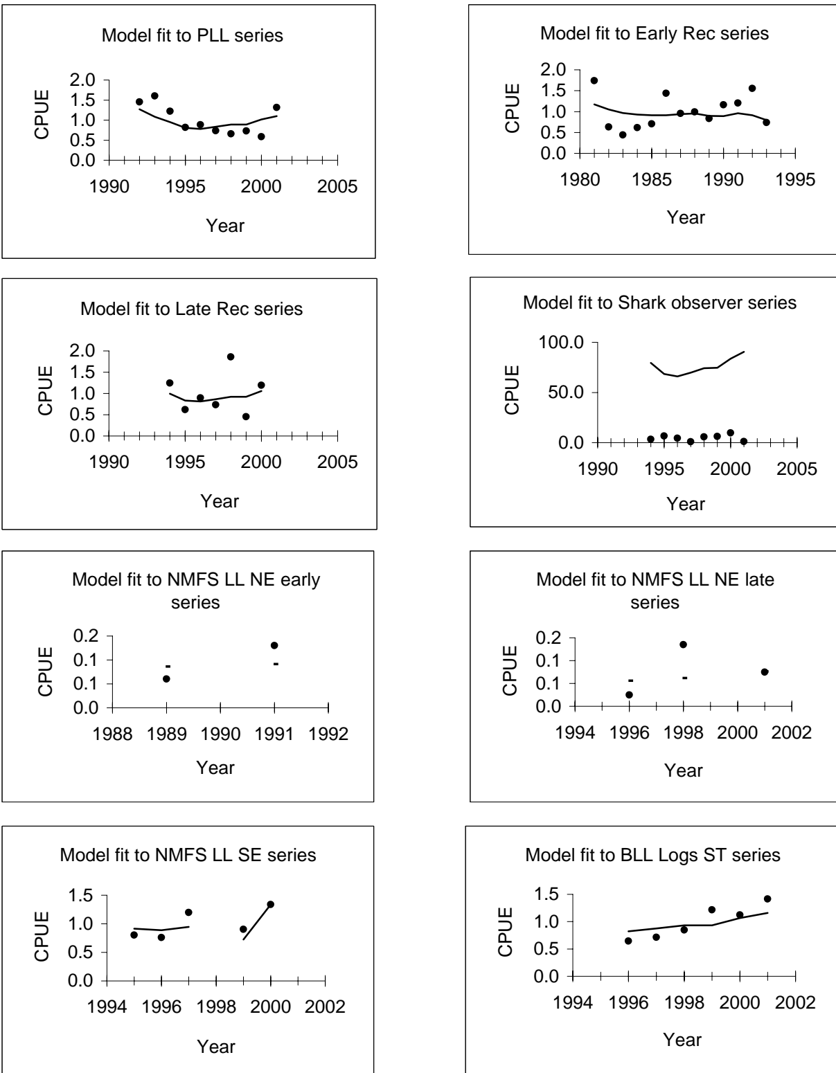
Figure 37. WinBUGS SSLRSG model fits to the individual CPUE series of the updated scenario for blacktip shark.
