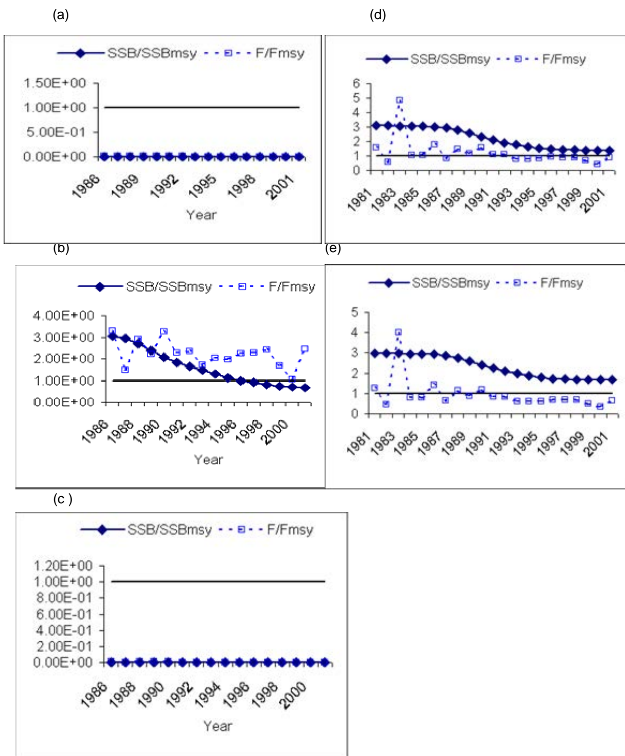
Figure 56. Trajectory of B/B_{msy} and F/F_{msy} for all Sandbar Updated ASPM models using (a) all indices, (b) fishery-dependent indices, or (c) fishery-independent indices; and for Sandbar Baseline models using (d) all indices or (e) fishery-independent indices.
