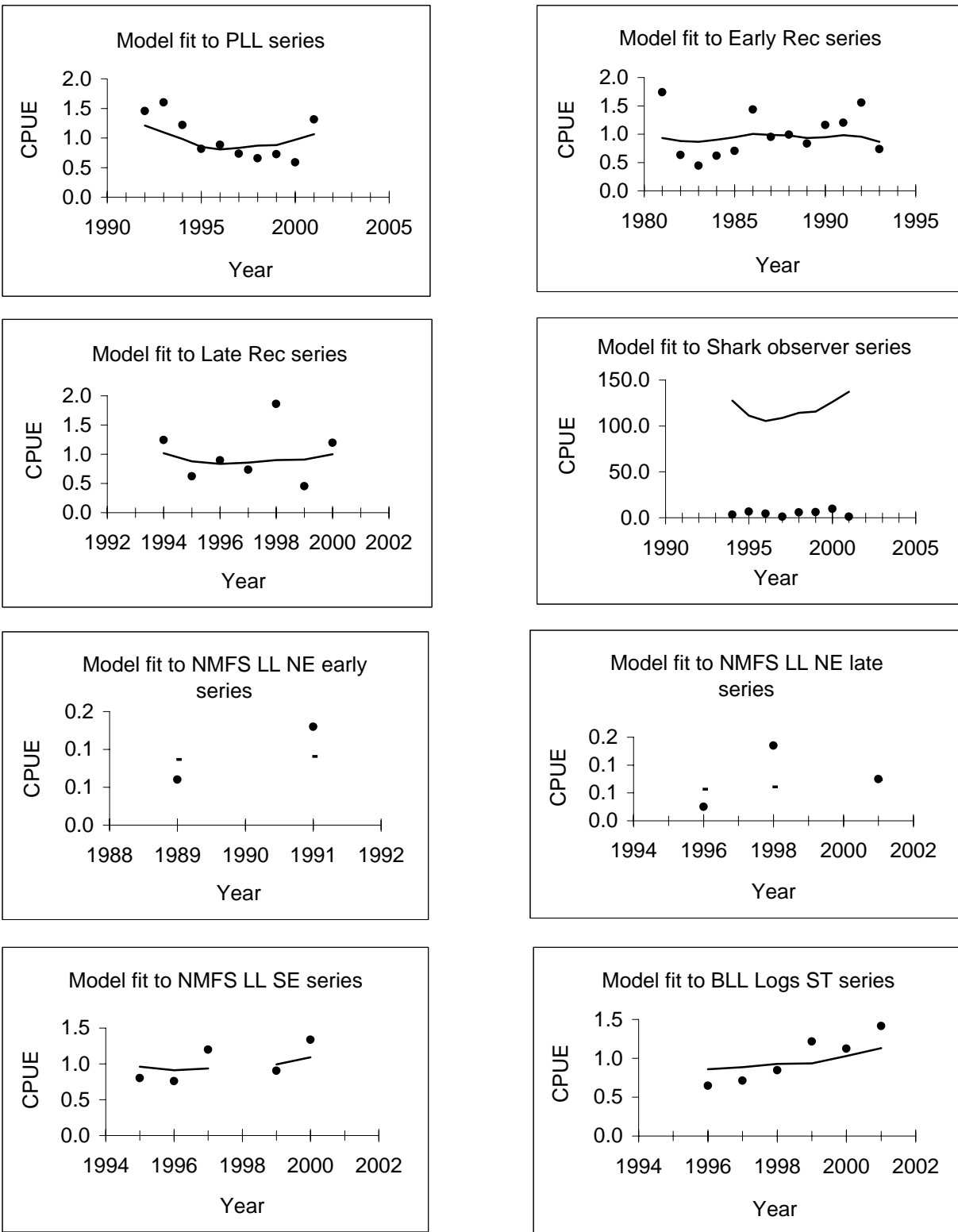
Figure 47. WinBUGS SSSPM fits to the individual CPUE series of the baseline scenario for blacktip shark.
