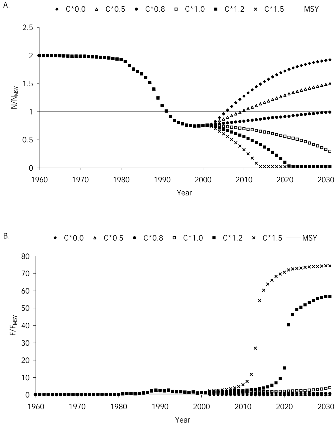
Figure 25. Estimated relative abundance (A) and fishing mortality rate (B) trajectories and projections (from 2001 to 2031) for alternative total allowable catch (TAC) harvesting policies (0 catch, 50%, 80%, 100%, 120%, and 150% of the 2000 catch) for the large coastal shark complex under the alternative catch scenario. Values shown are medians; the horizontal line at 1 denotes the MSY (MSC) level.
