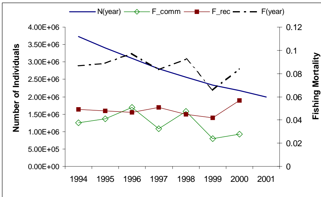
Figure 54. Annual estimates of commercial fishing mortality ( F_{comm} ), recreational fishing mortality ( F_{rec} ), annual fishing mortality ( F(year) ), and population size ( N(year) ) for Blacktip shark MLE models. (a) updated model; (b) baseline model.
