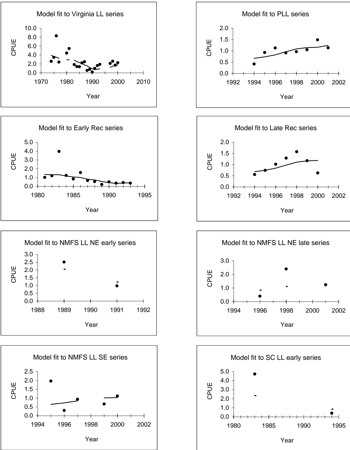
Figure 33. WinBUGS SSLRSG model fits to the individual CPUE series of the updated scenario for sandbar shark.
