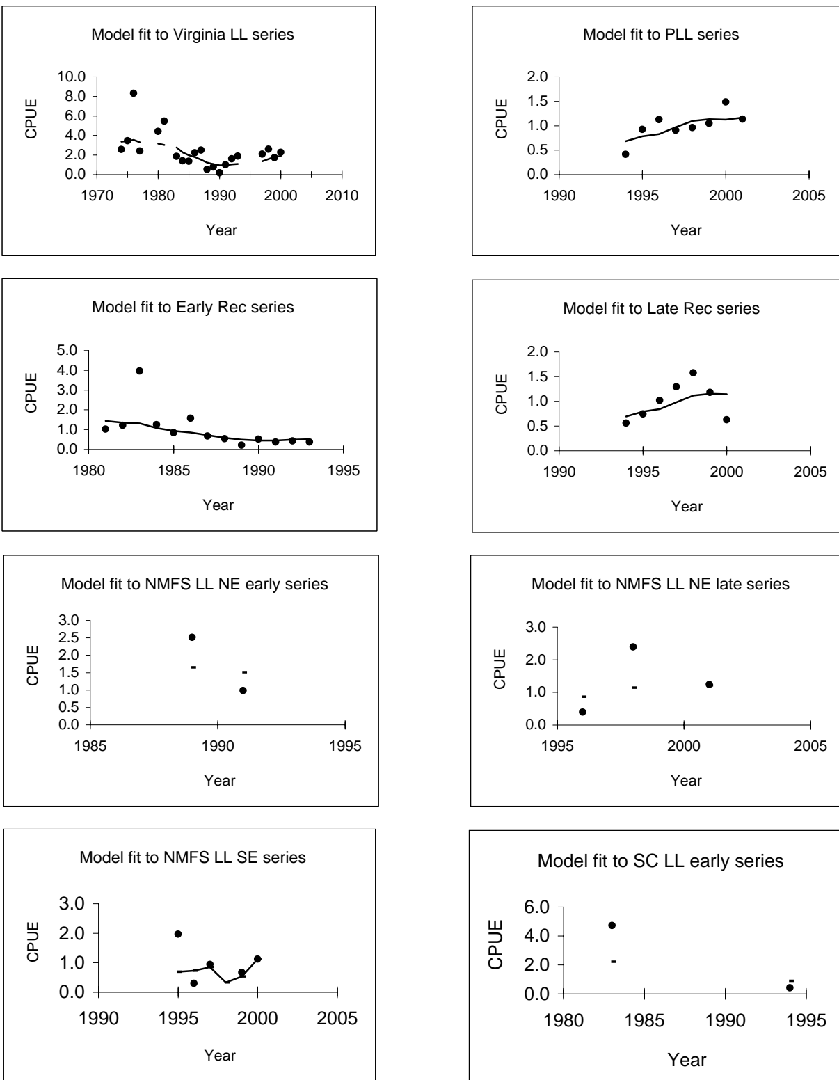
Figure 31. WinBUGS SSSPM fits to the individual CPUE series of the updated scenario for sandbar shark.
