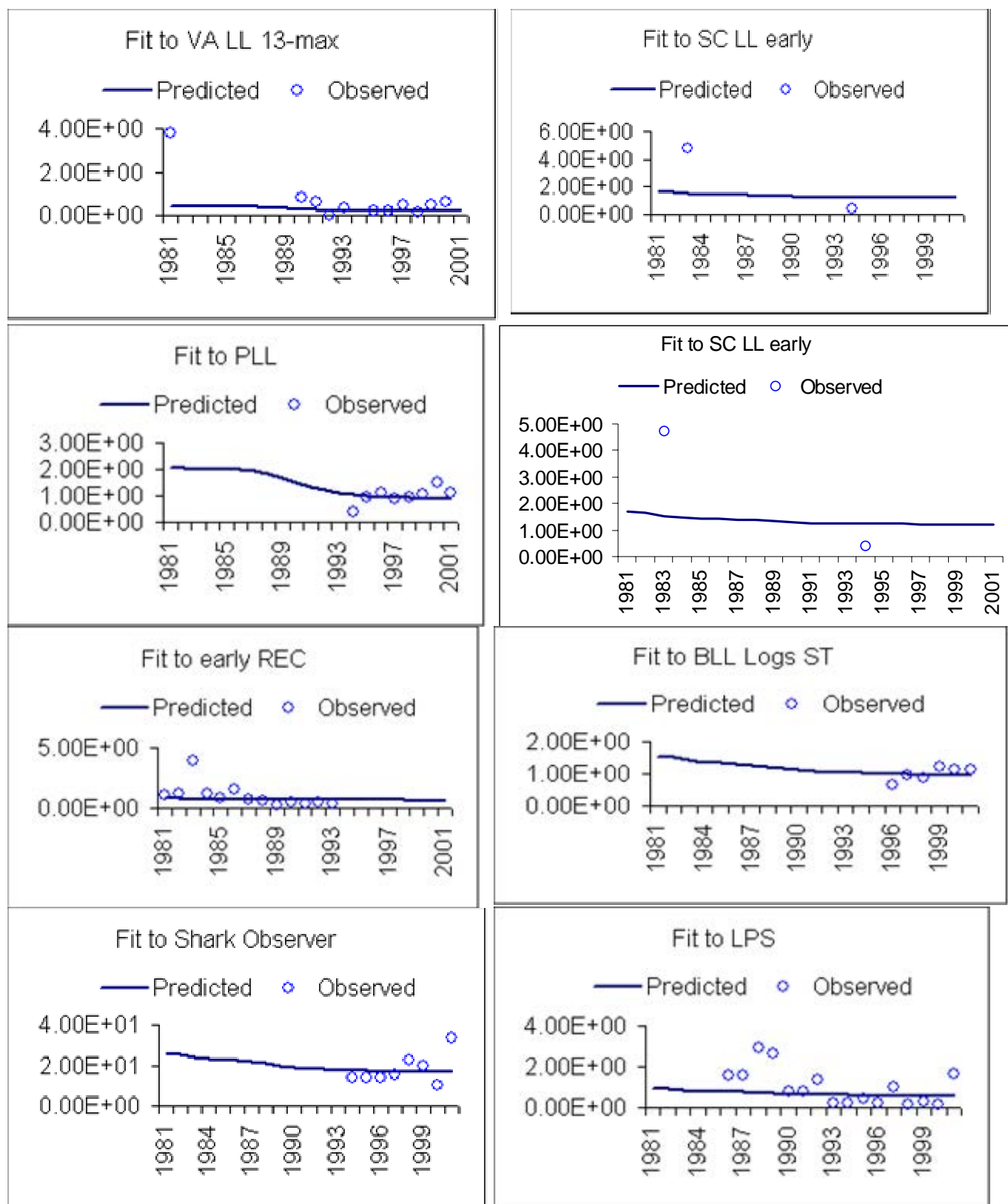
Figure 64. Fit to CPUE indices for Sandbar Baseline ASPM model using all indices.
