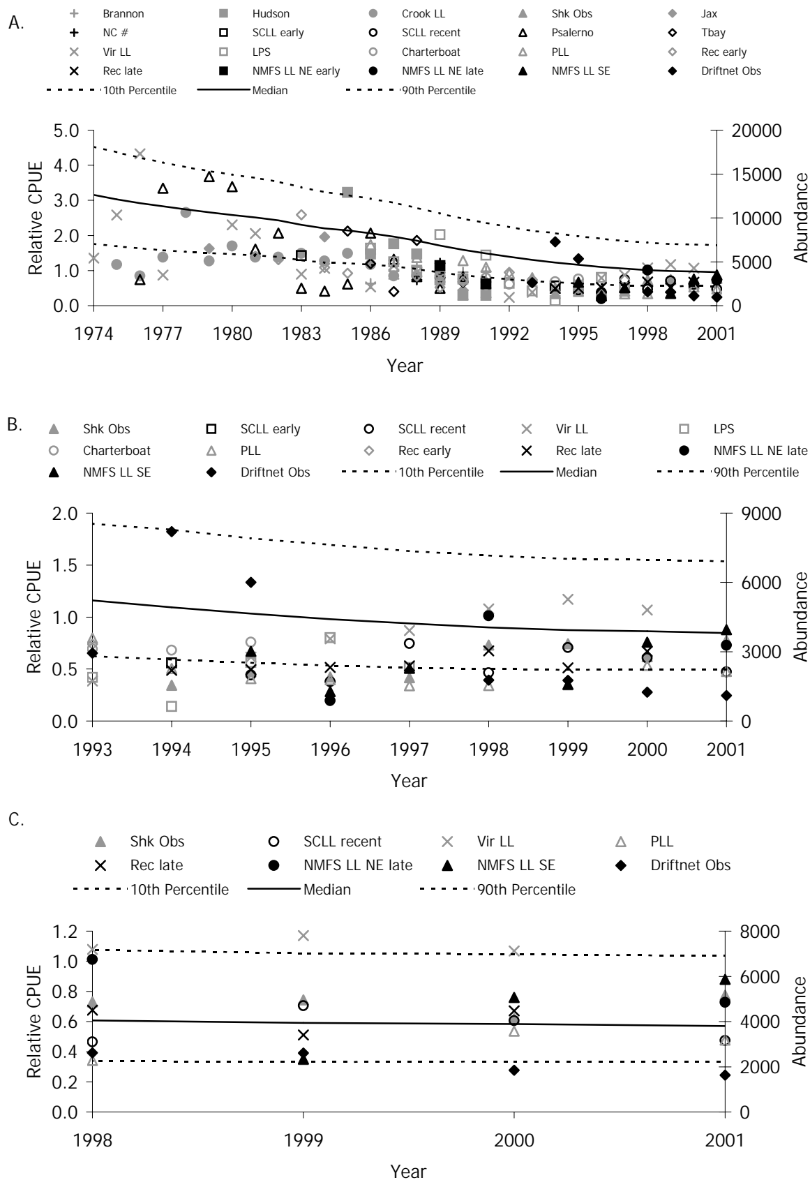
Figure 18. Abundance of the large coastal shark complex predicted by the surplus production model fitted to the catch and CPUE series for the baseline scenario. The series are scaled (divided by the catchability coefficient for each series and the overall mean for all series). A) 1974-2001, B) 1993-2001, C) 1998-2001.
