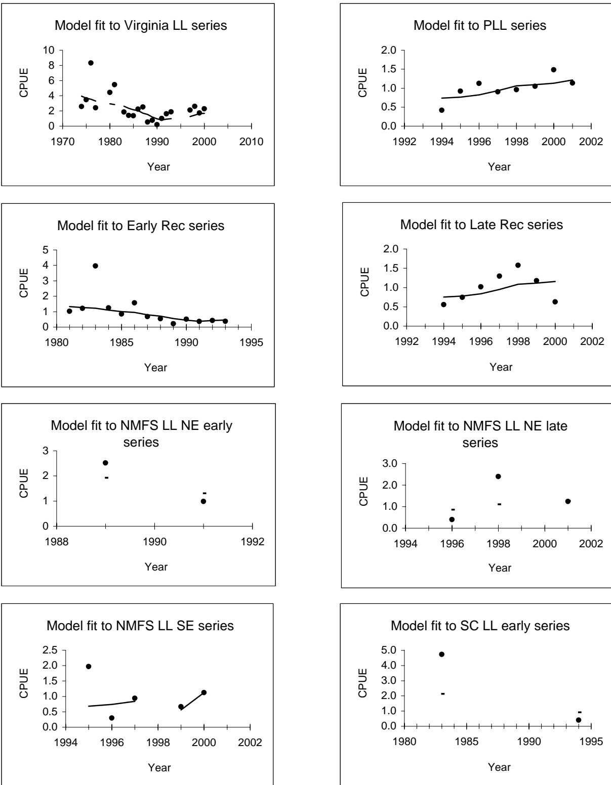
Figure 45. WinBUGS SSLRSG model fits to the individual CPUE series of the baseline scenario for sandbar shark.
