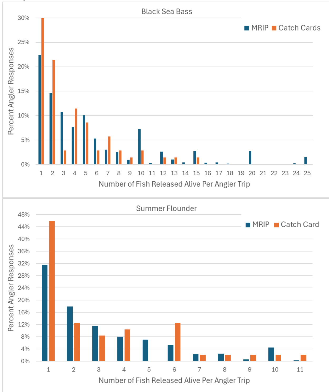
Figure 5. The number of fish anglers reported releasing alive from MRIP public intercept data as compared to the pilot catch cards for select species (Black Sea Bass, Summer Flounder, Scup, Spotted Seatrout, Striped Bass, and Red Drum). Data from all catch card pilot states in waves 3-5 were used in the analysis from the private/rental boat and shore modes and all areas. Note the different scales on the x- and y-axes.
