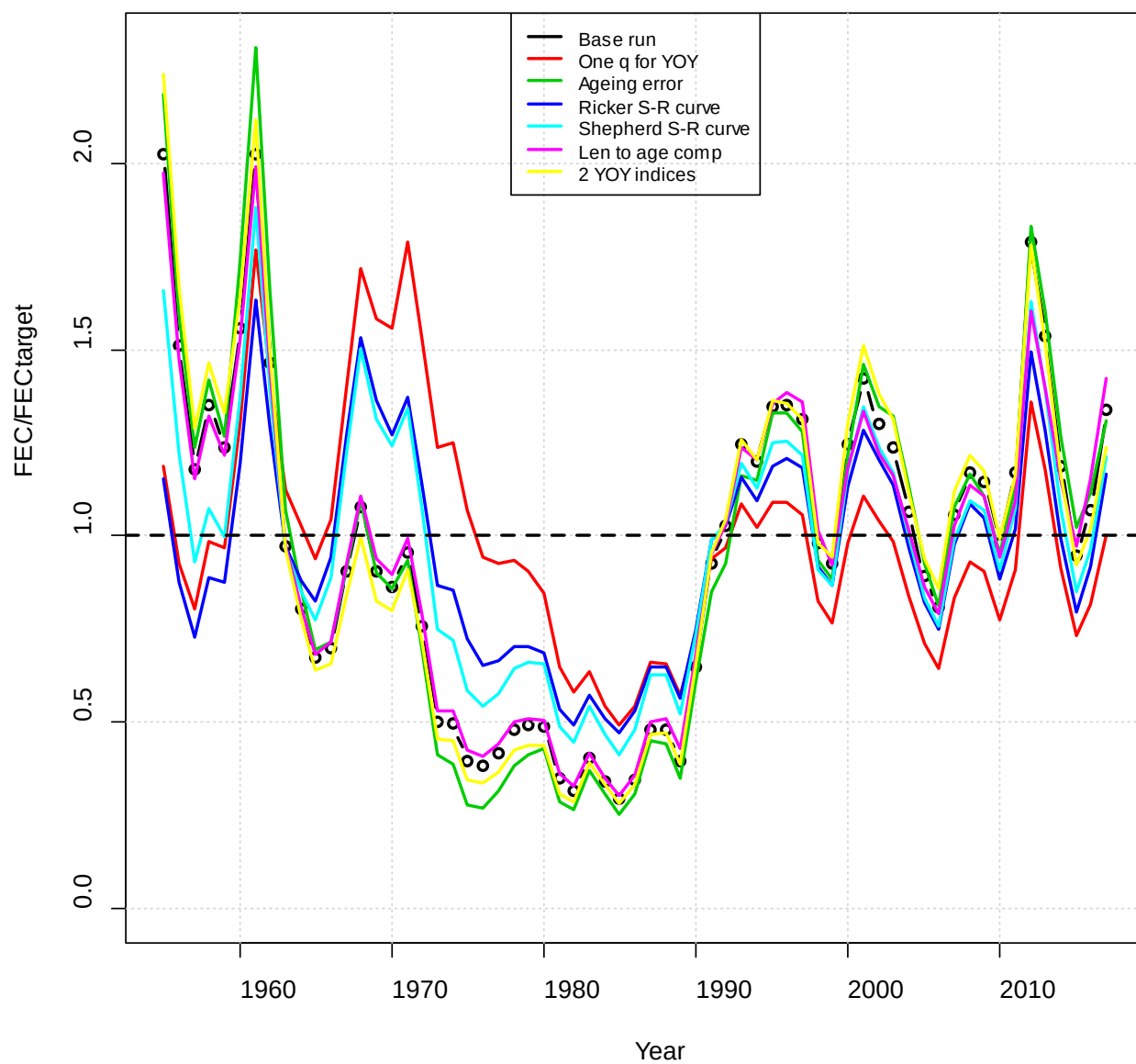
Figure 225. Fecundity divided by the target fecundity for the suite of sensitivity runs related to catchability, ageing error, and the stock-recruitment curve.
