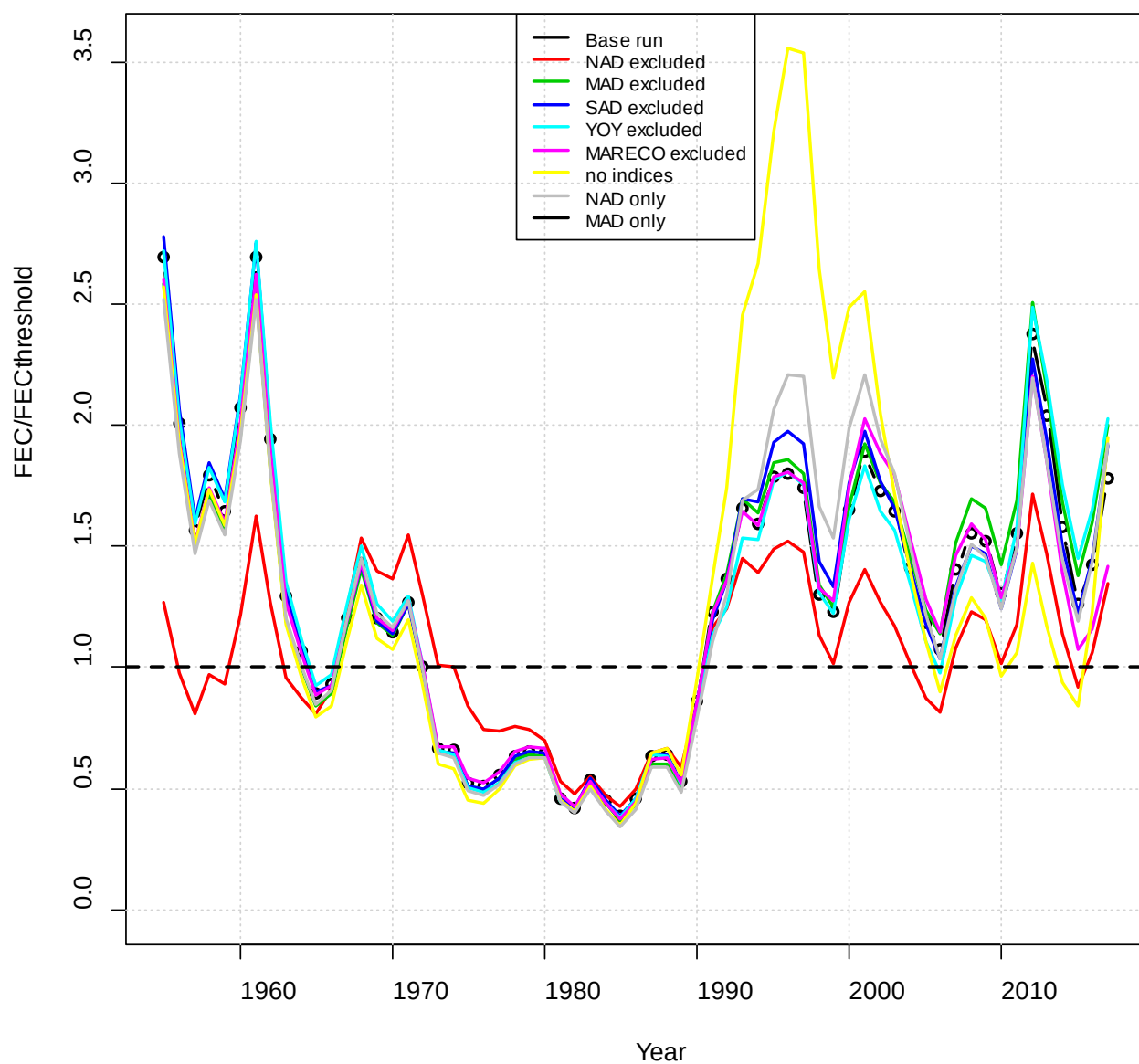
Figure 216. Fecundity divided by the threshold fecundity for the suite of sensitivity runs related to index choice.
