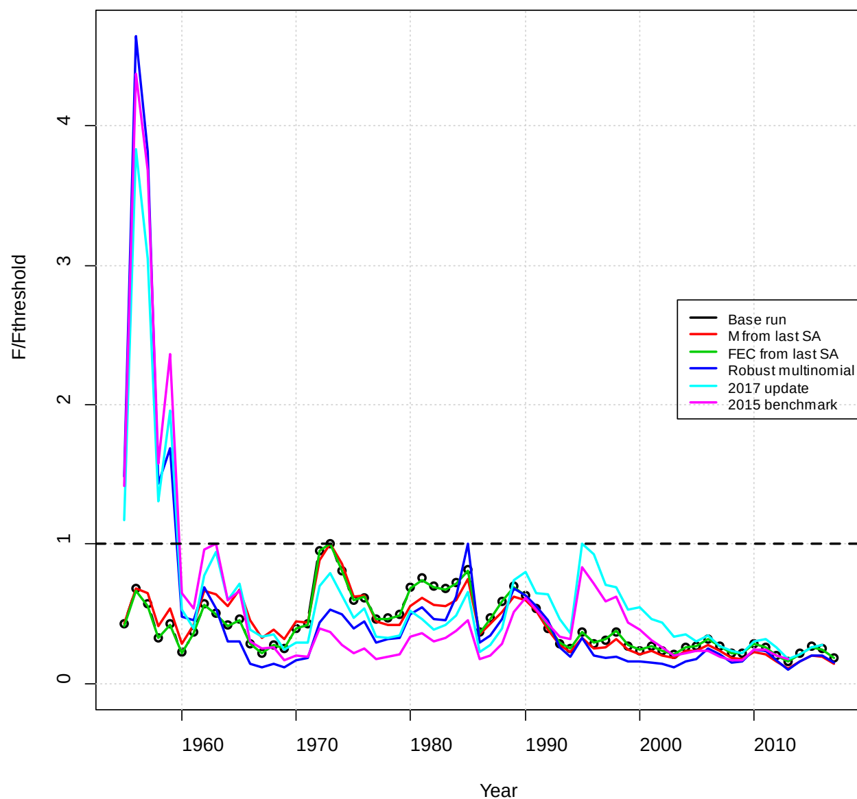
Figure 210. Fishing mortality rate divided by the threshold F for the suite of sensitivity runs related to continuity with the last update and benchmark assessments.
