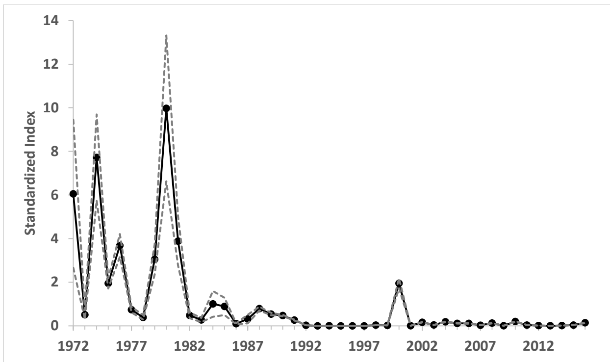
Figure 83. Standardized index of relative abundance of YOY Atlantic menhaden developed from Maryland Department of Natural Resources Coastal Bays Survey with 95% confidence intervals.
