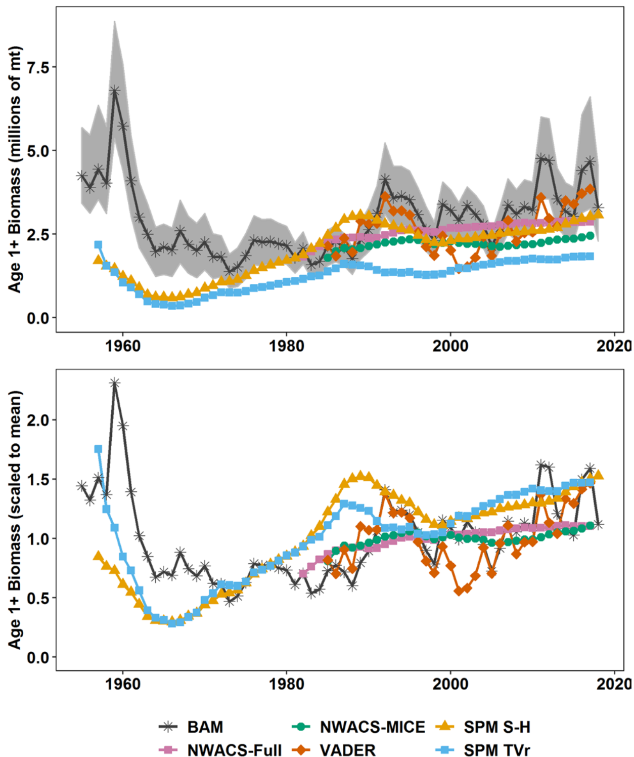
Figure 249. Estimates of age-1+ biomass from the BAM model and the ERP models on an absolute scale (top) and scaled to their time series mean (bottom). Shaded area around BAM estimates indicates 95% confidence interval from MCMC analysis, a minimum estimate of uncertainty.
