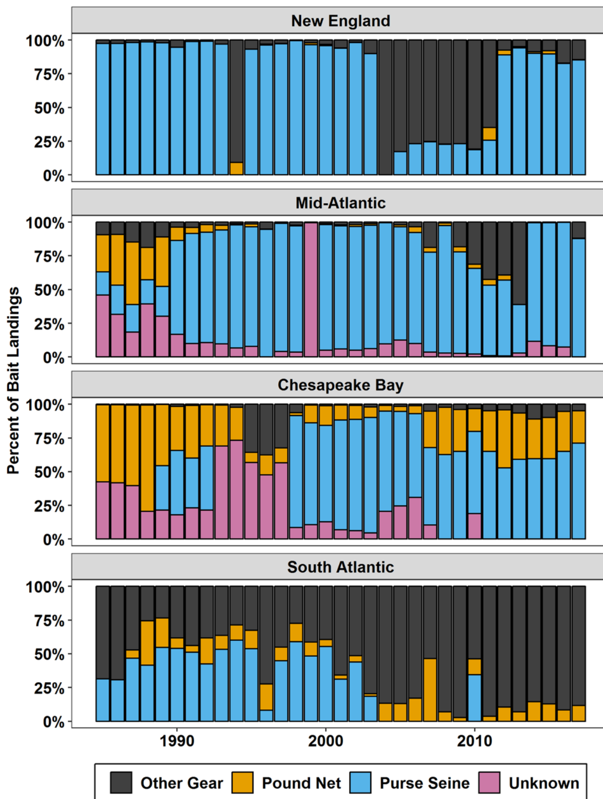
Figure 46. a. Percent of bait landings by major gear types for each region.
