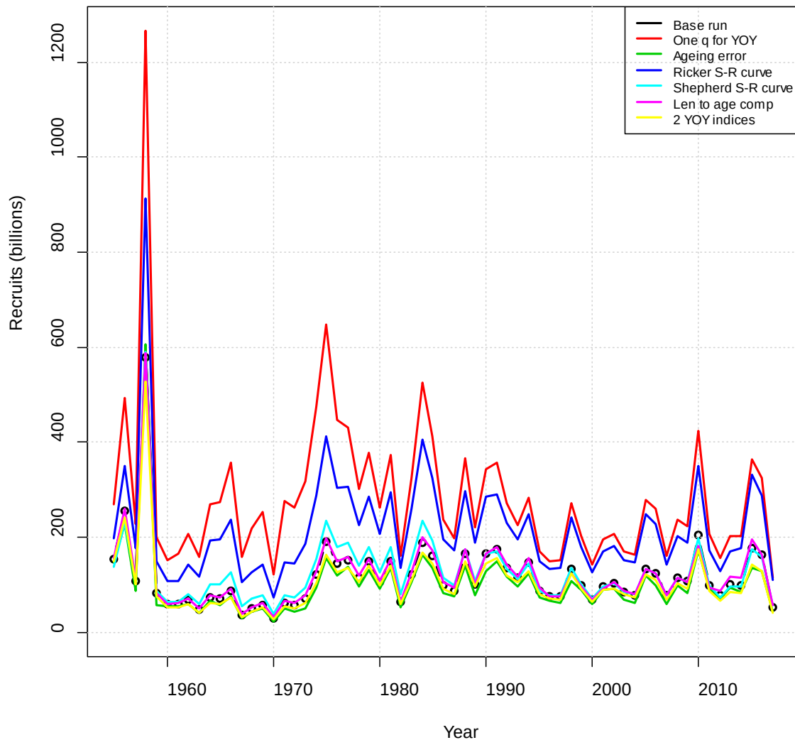
Figure 169. Recruitment in billions of fish for 1955-2017 for a suite of sensitivity runs that explored model structure related to ageing, catchability, the stock-recruitment curve, and data type.
