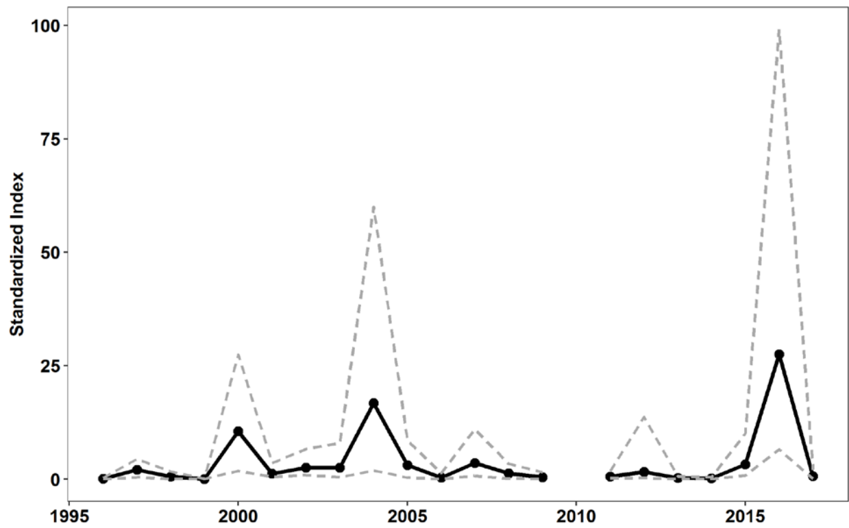
Figure 58. Standardized index of relative abundance of YOY Atlantic menhaden developed from the Connecticut Long Island Trawl Survey with 95% confidence intervals.
