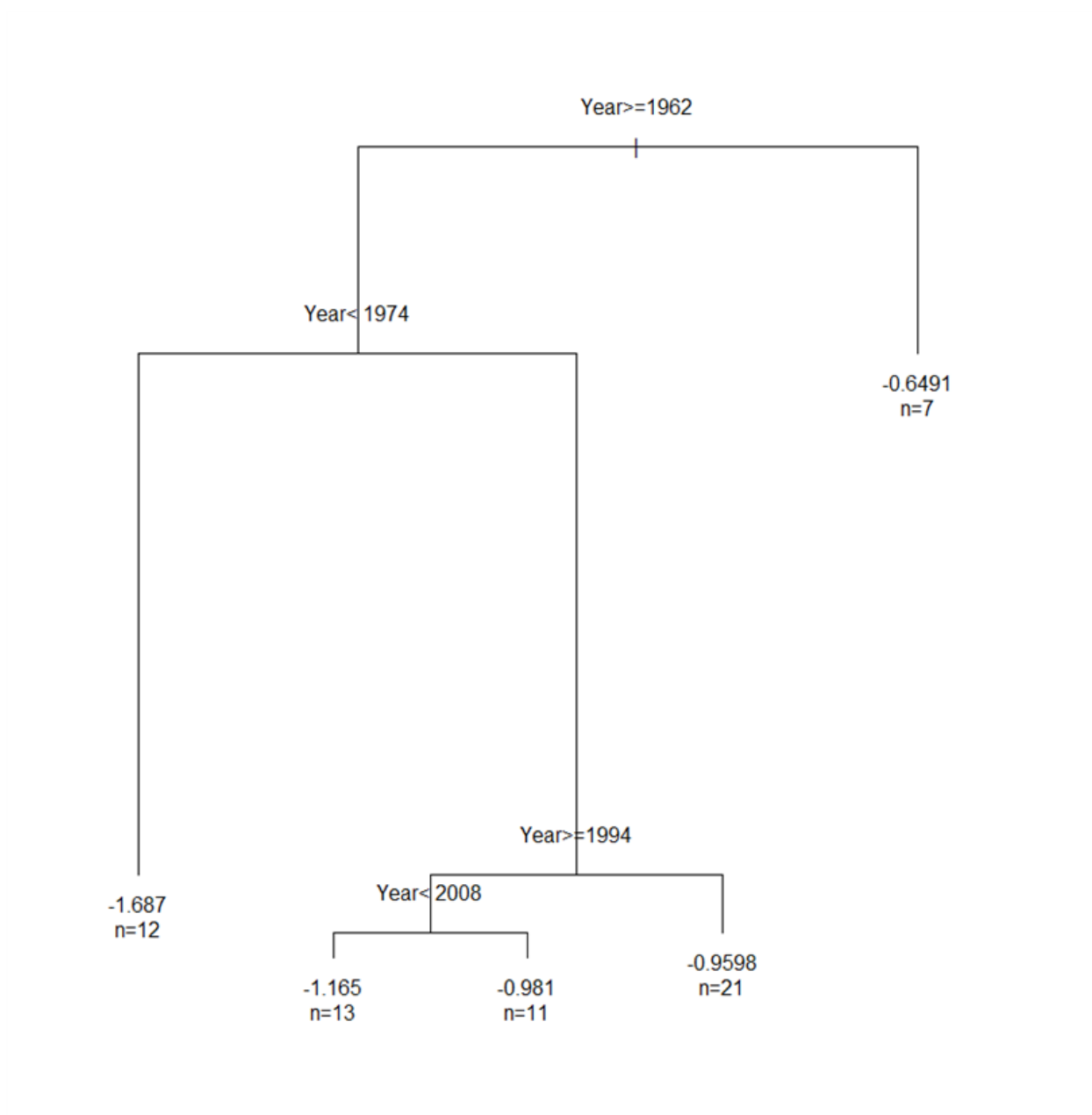
Figure 36. Tree produced by R package RPART to identify regimes for Atlantic menhaden productivity.
