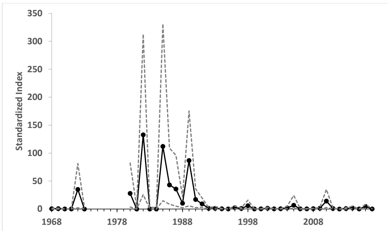
Figure 89. Standardized index of relative abundance of YOY Atlantic menhaden developed from the VIMS Juvenile Striped Bass Seine Survey with 95% confidence intervals.
