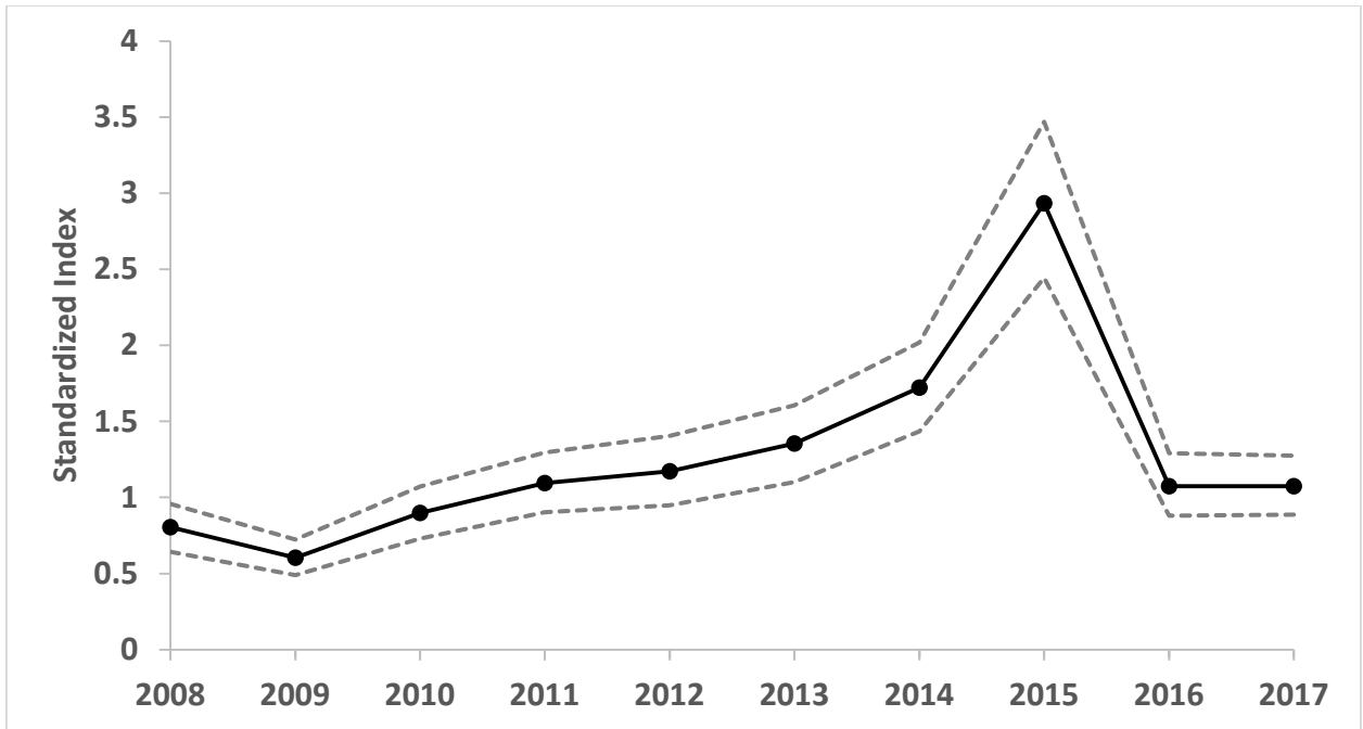
Figure 95. Standardized index of relative abundance of age 1+ Atlantic menhaden developed from the North Carolina Program 915 Pamlico Sound Independent Gill Net Survey. The grey ribbon is the 95% confidence interval.
