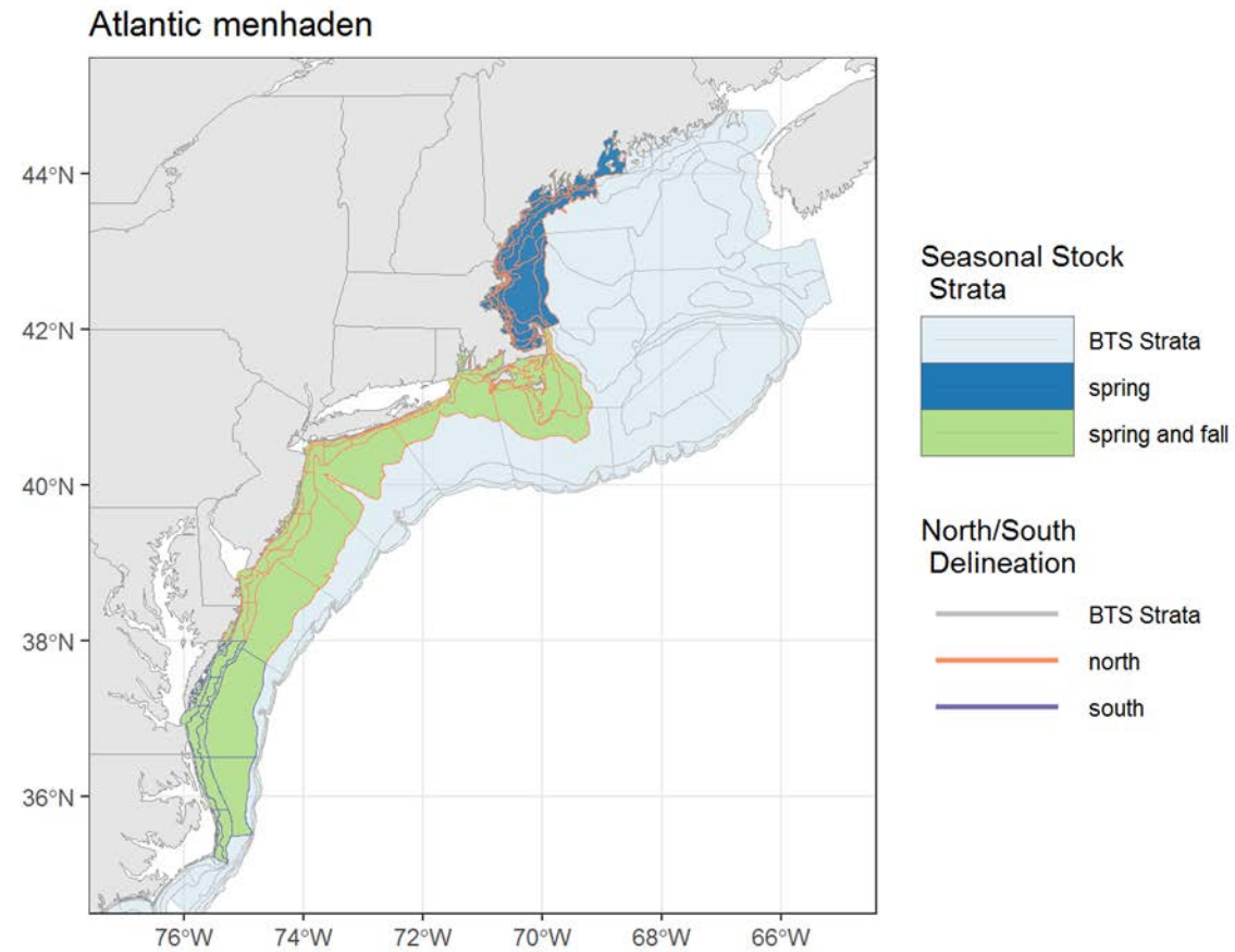
Figure 21. Map of Northeast Fisheries Science Center (NEFSC) bottom trawl survey (BTS) spring and fall strata selected for the Ecosystem Context analysis for Atlantic menhaden (source: NEFSC).
