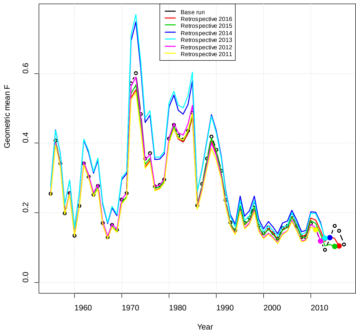
Figure 191. Geometric mean fishing mortality rate for ages-2 to -4 for 1955-2017 for the retrospective analysis going back until 2011 and the northern age comp fixed at a value similar to the recent time period.
