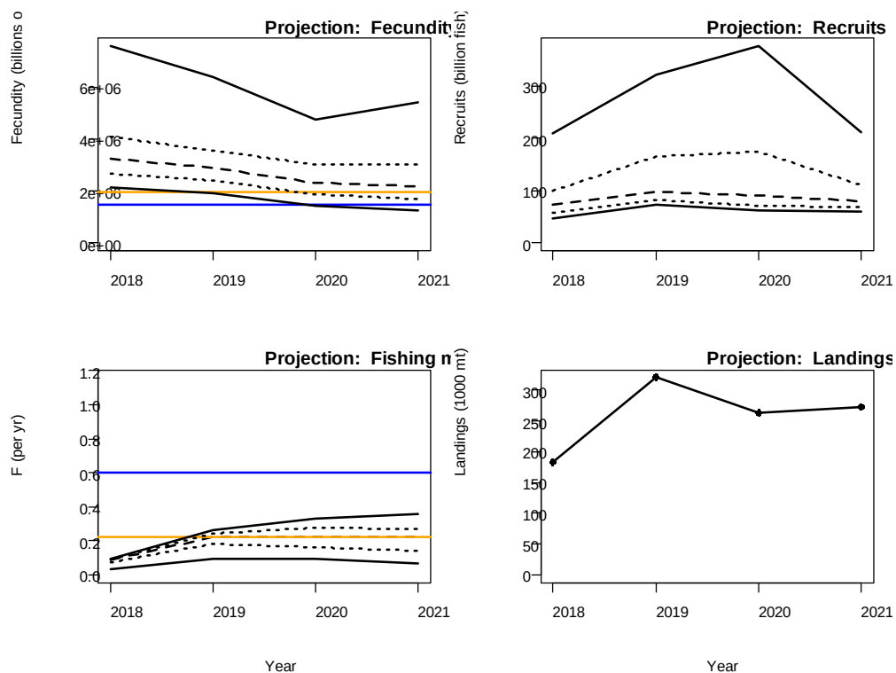
Figure 206. Fecundity, recruits, geometric mean fishing mortality rate, and landings for projections done to reach the F_{\text{TARGET}} during 2019-2021. The blue lines indicate the thresholds and the orange lines indicate the targets for the base run. The dashed black line is the 50 th percentile (median), the dotted black lines are the 25 th and 75 th percentiles, and the solid black lines are the 5 th and 95 th percentiles.
