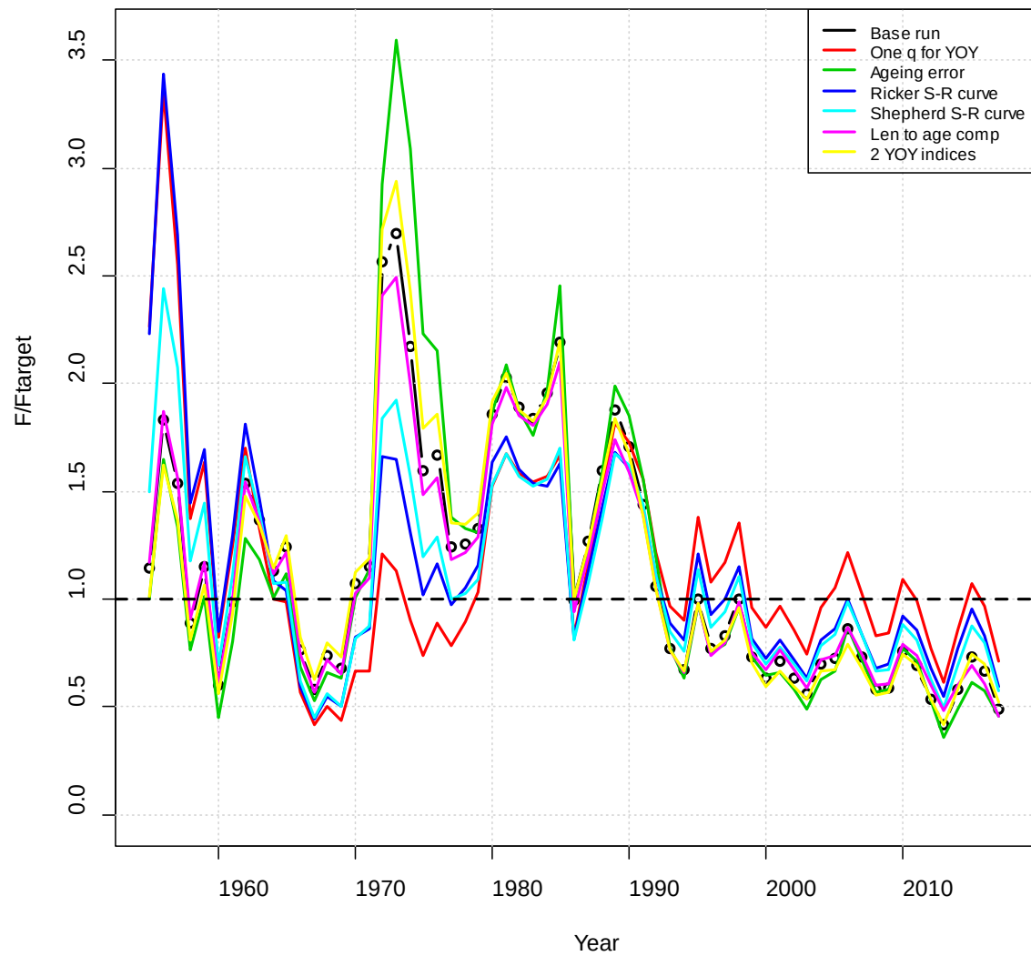
Figure 223. Fishing mortality rate divided by the target F for the suite of sensitivity runs related to catchability, ageing error, and the stock-recruitment curve.
