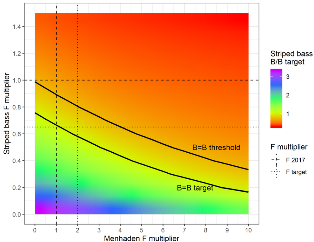
Figure 251. Striped bass age 6+ biomass ratio ( B/B_{\text{TARGET}} ) in the terminal year of the EwE projections as a function of fishing mortality on both Atlantic menhaden and striped bass. Fishing mortality for each species is increased or decreased relative to F in 2017 through the F multipliers, i.e., an F multiplier equal to 1 indicates fishing at F_{2017} . The solid black lines represent the contours where striped bass age 6+ biomass equals the striped bass biomass target or threshold.
