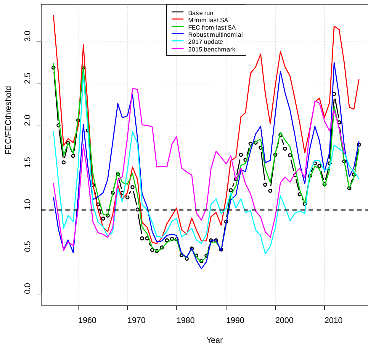
Figure 212. Fecundity divided by the threshold fecundity for the suite of sensitivity runs related to continuity with the last update and benchmark assessments.
