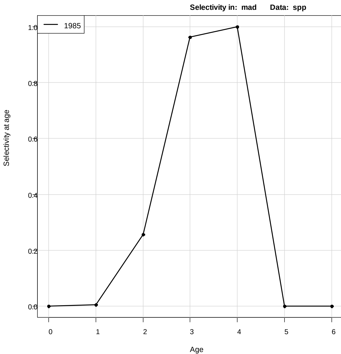
Figure 144. Selectivity-at-age for the MAD index for 1985-2017.
