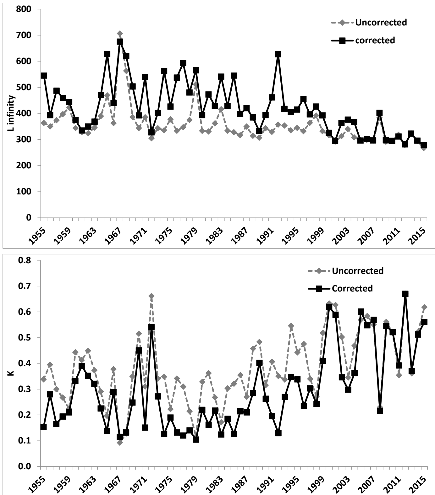
Figure 6. A comparison of the estimated annual, cohort-based von Bertalanffy growth coefficients L_{\infty} (top) and K (bottom) with and without the bias correction as detailed in Schueller et al. (2014).
