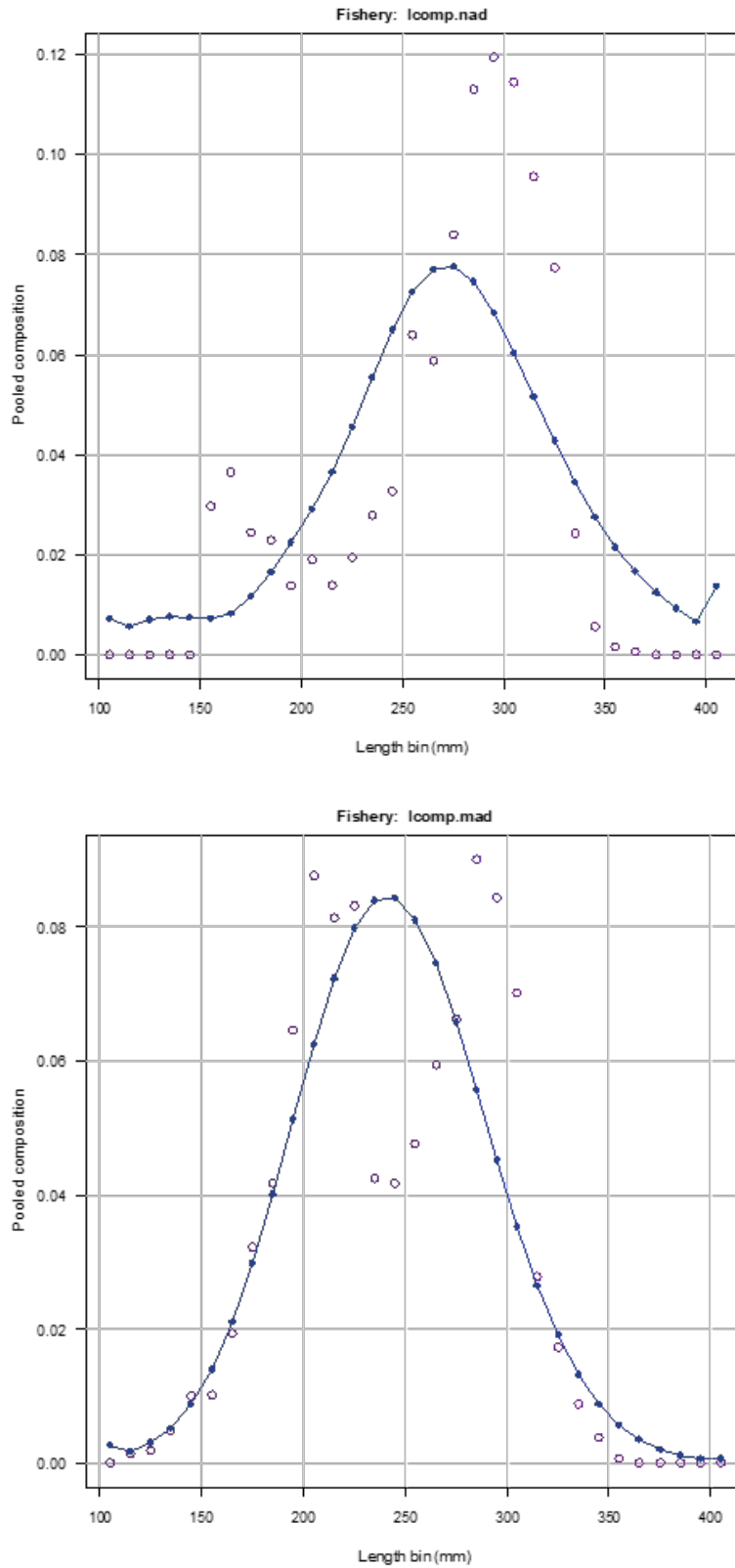
Figure 136. Pooled length compositions for the NAD (upper) and MAD (lower) indices. Pooling was done with no weighting.
