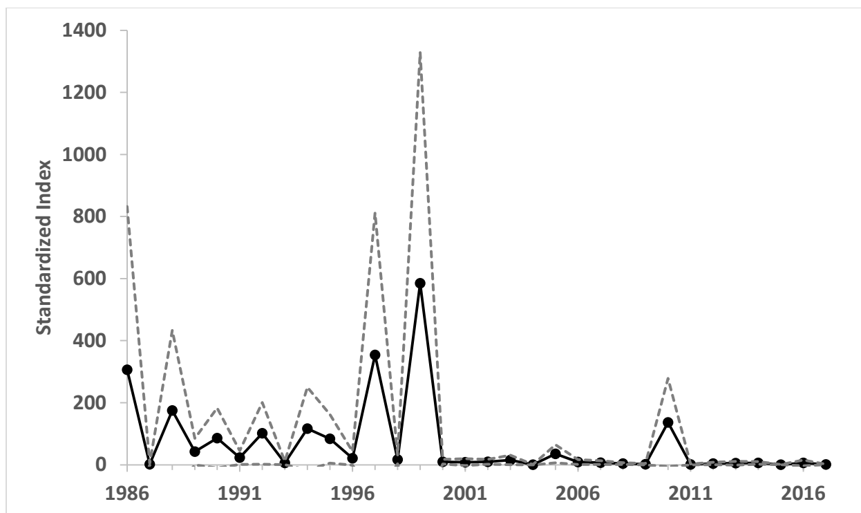
Figure 72. Standardized index of relative abundance of YOY Atlantic menhaden developed from the New Jersey Delaware River Striped Bass Seine Survey with 95% confidence intervals.
