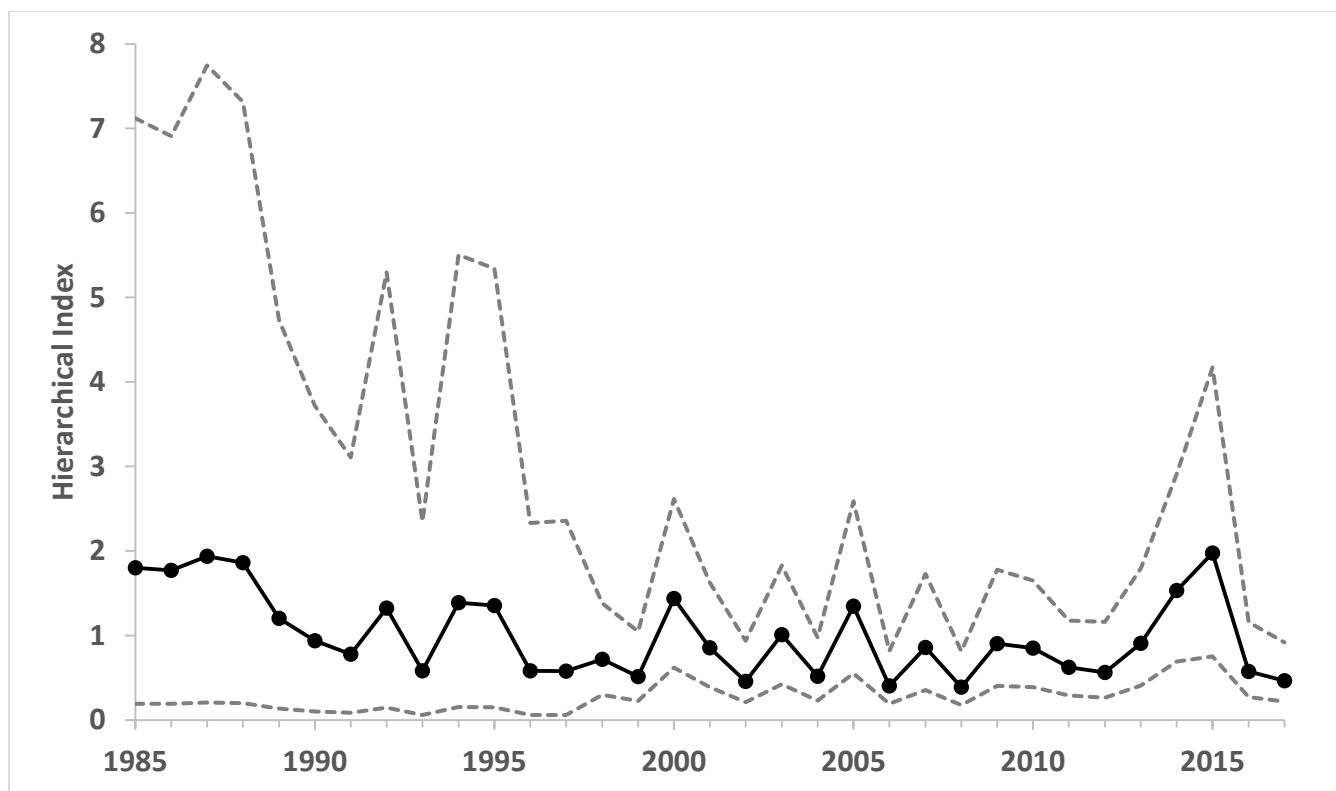
Figure 111. Time series of the Mid-Atlantic adult menhaden relative abundance index (MAD) as estimated from hierarchical analysis (Conn 2009). The black line gives the posterior mean and the grey, dashed lines represents a 95% credible interval about the time series.
