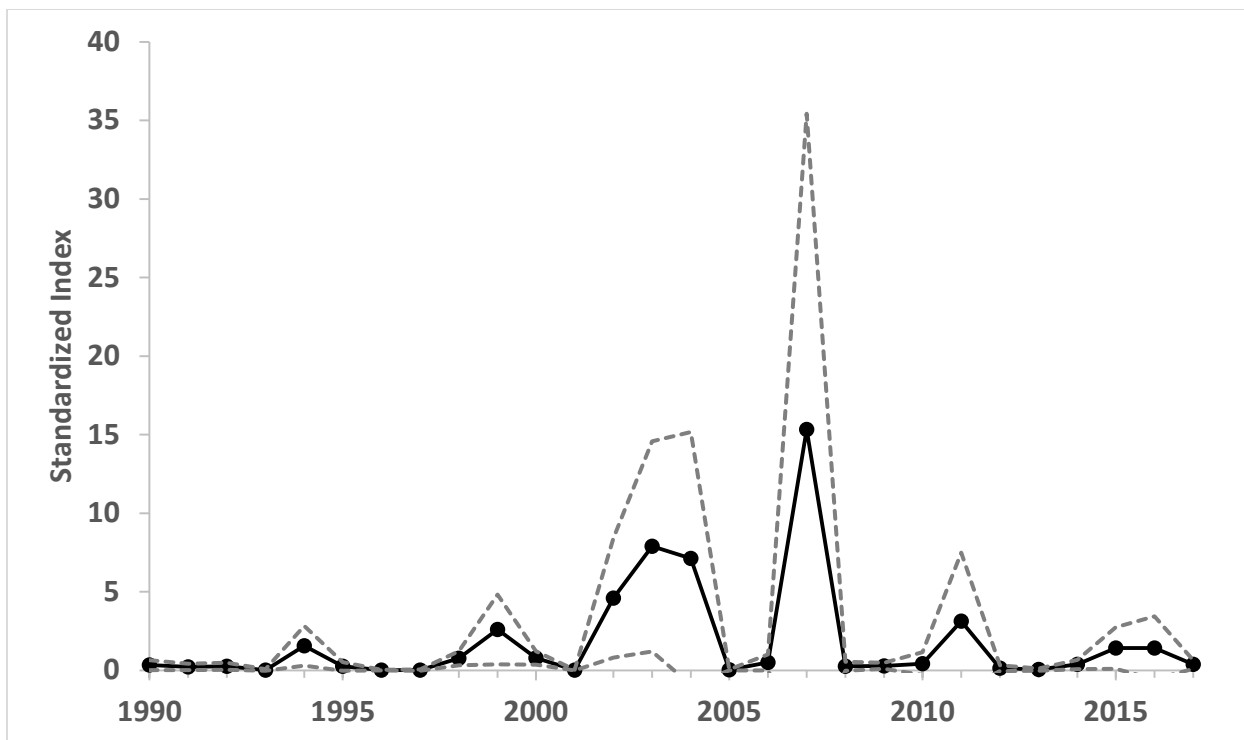
Figure 74. Standardized index of relative abundance of YOY Atlantic menhaden developed from the New Jersey Ocean Trawl Survey with 95% confidence intervals.
