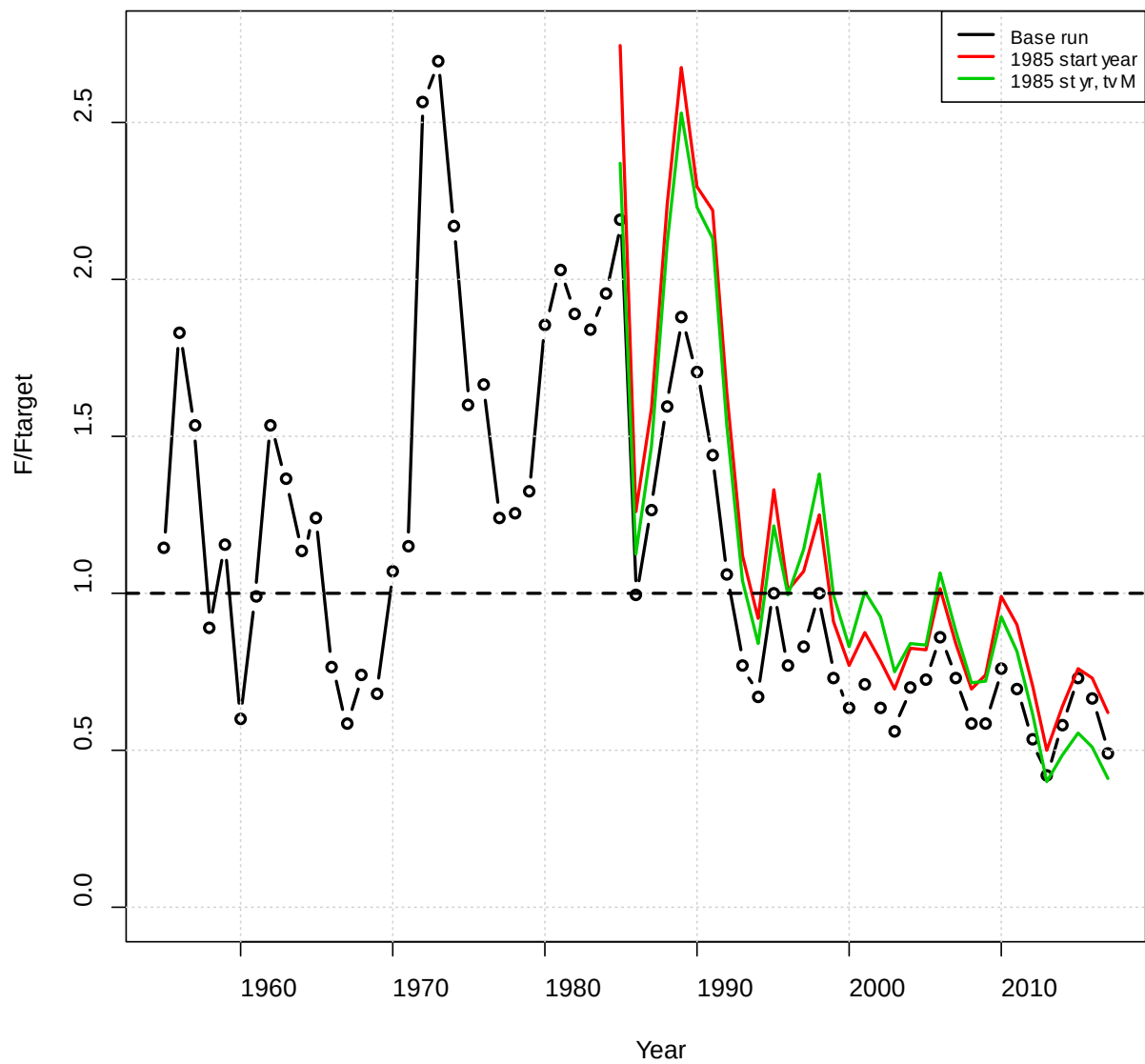
Figure 235. Fishing mortality rate divided by the target F for the suite of sensitivity runs related to start year and time-varying M .
