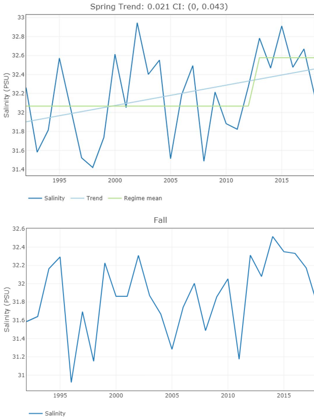
Figure 25. Trend and regime mean for spring and fall surface salinity from the NEFSC trawl survey strata included in the Atlantic Menhaden Ecosystem Context Report.
