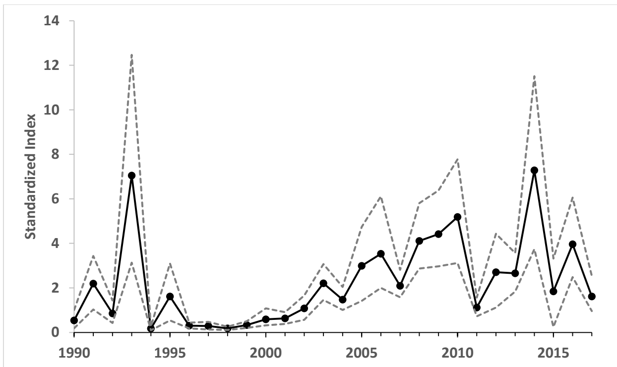
Figure 87. Standardized index of relative abundance of YOY Atlantic menhaden developed from the VIMS Juvenile Fish and Blue Crab Trawl Survey with 95% confidence intervals.
