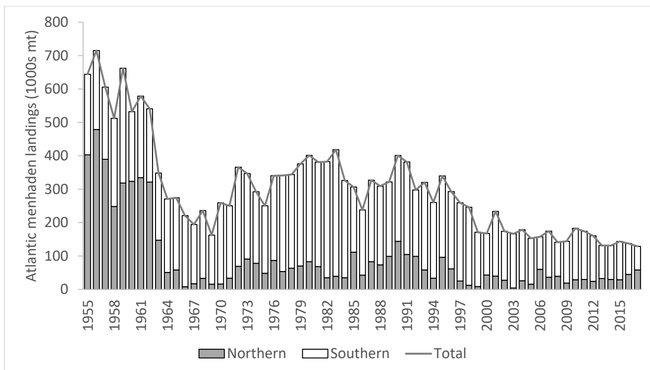
Figure 42. Atlantic menhaden reduction landings (1000s mt) from 1955-2017. The northern region is comprised of landings from north of Virginia Eastern Shore and the southern region is comprised of landings from Virginia Eastern Shore and south (Source: NMFS Beaufort).
