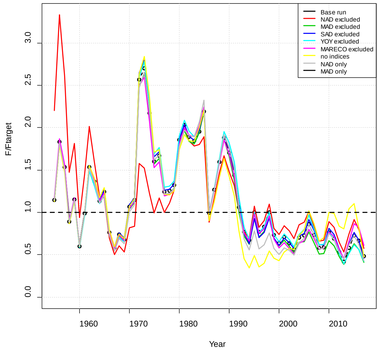
Figure 215. Fishing mortality rate divided by the target F for the suite of sensitivity runs related to index choice.
