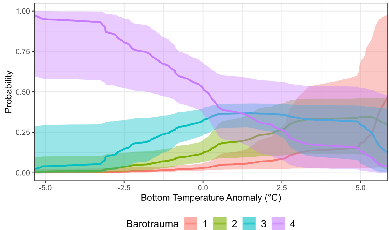
Figure 4: Bayesian Mixed Effects Ordinal Regression Model prediction of probability of barotrauma score as a function of bottom temperature anomaly.
