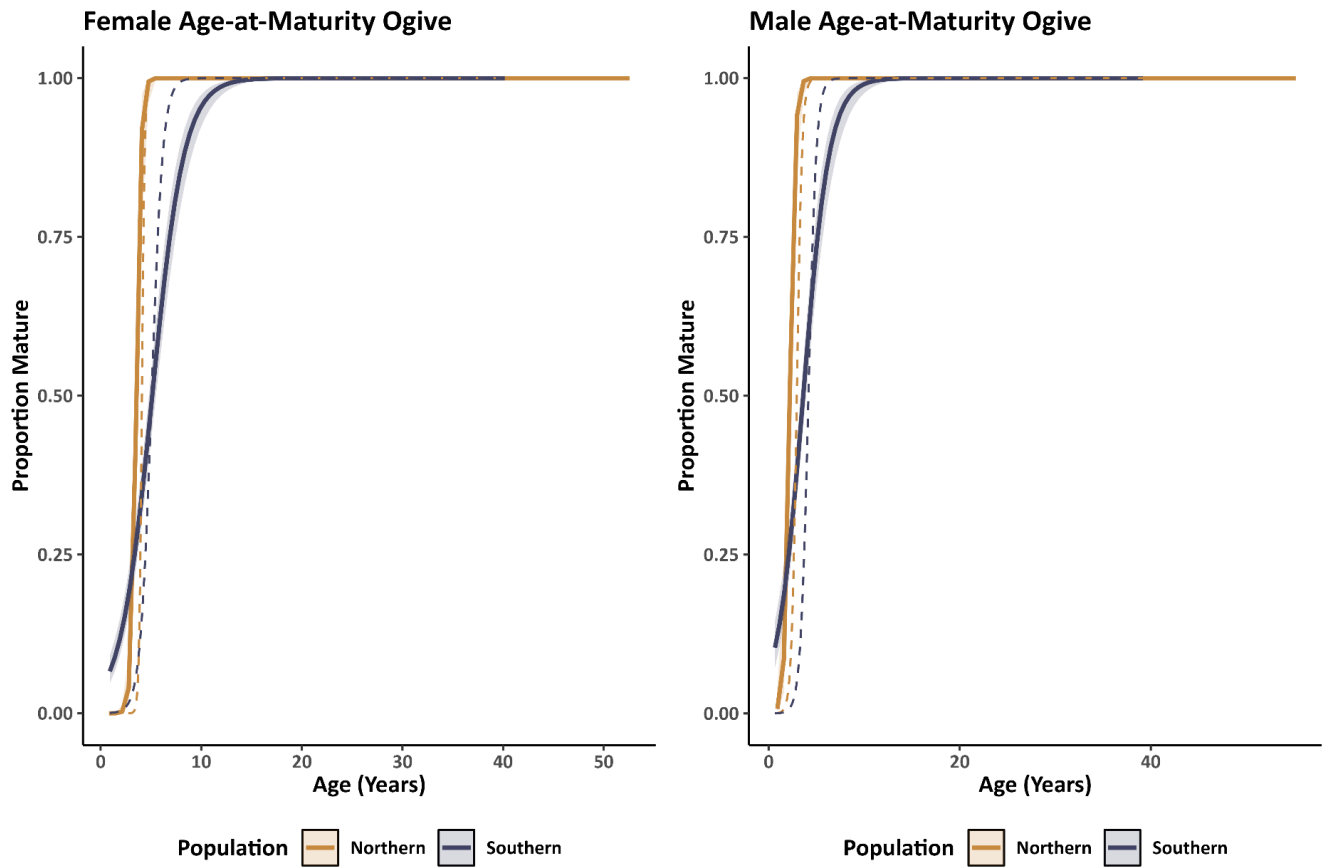
Figure 16. Best fit age-at-maturity ogives for female (left panel) and male (right panel) red drum from the southern (solid blue line) and northern (solid orange line) stocks. Shaded regions represent 95% confidence interval about the ogive. Dashed lines are the maturity ogives presented in SEDAR 44.
