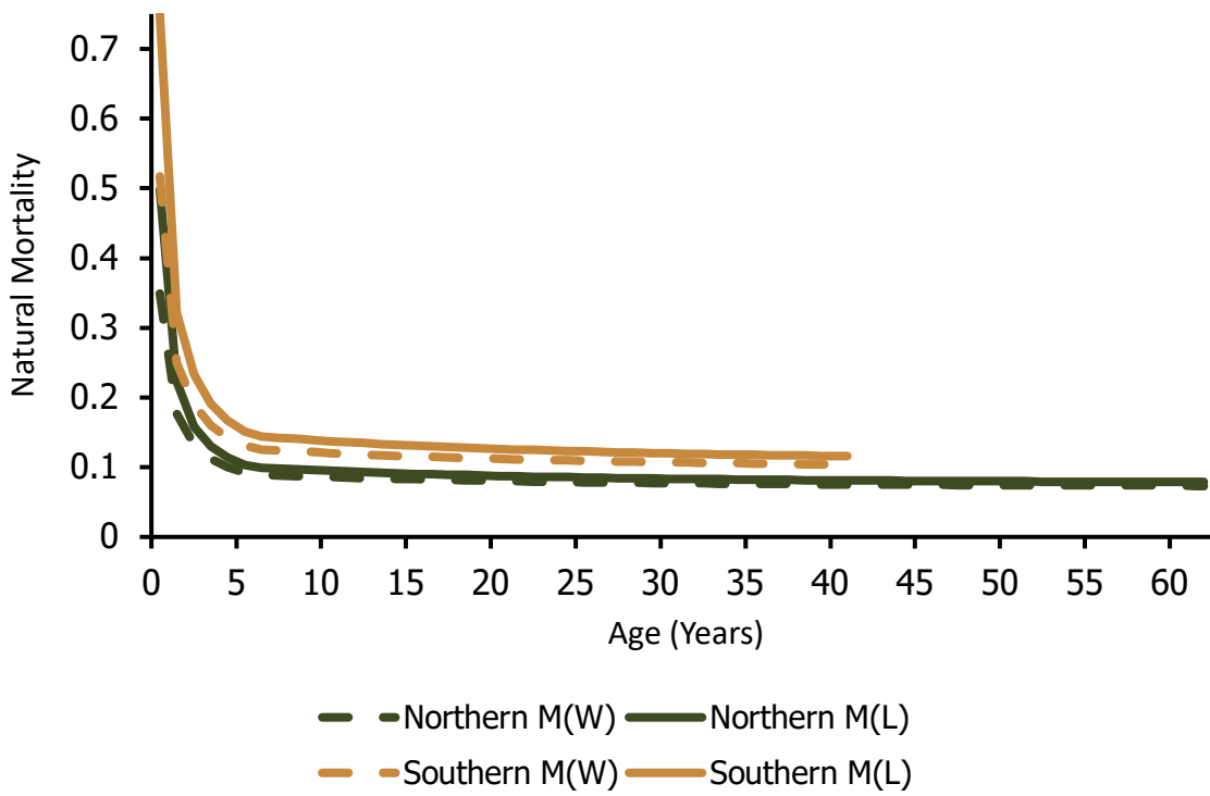
Figure 21. Northern (green lines) and southern (gold lines) externally derived natural mortality estimates based on stock-specific maximum age and either weight-based M-at-age (dashed lines; Lorenzen 1996) or length-based M-at-age (solid lines; Lorenzen 2022).
