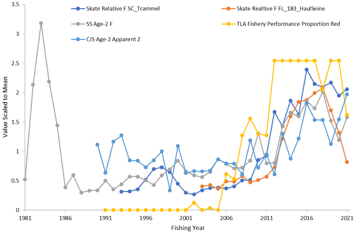
Figure 204. Comparison of scaled mortality estimates/metrics from analyses for the southern red drum stock.
