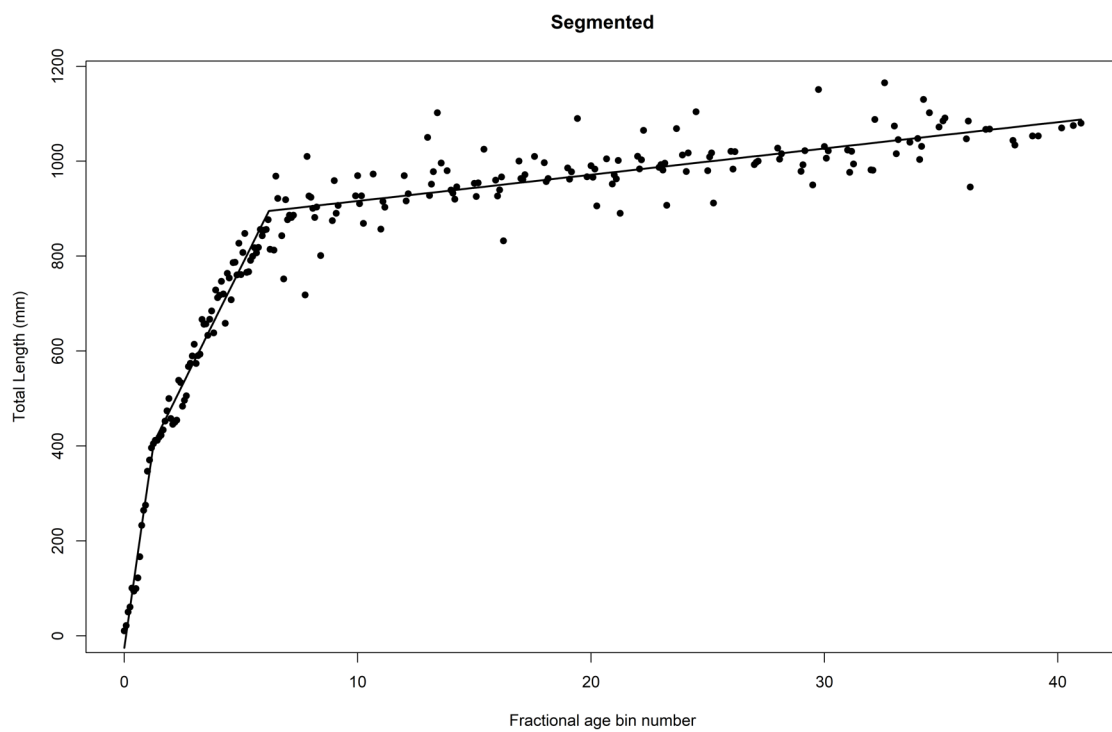
Figure 10. Segmented regression on red drum biological mean length-at-age by stock. (a) northern and (b) southern.
