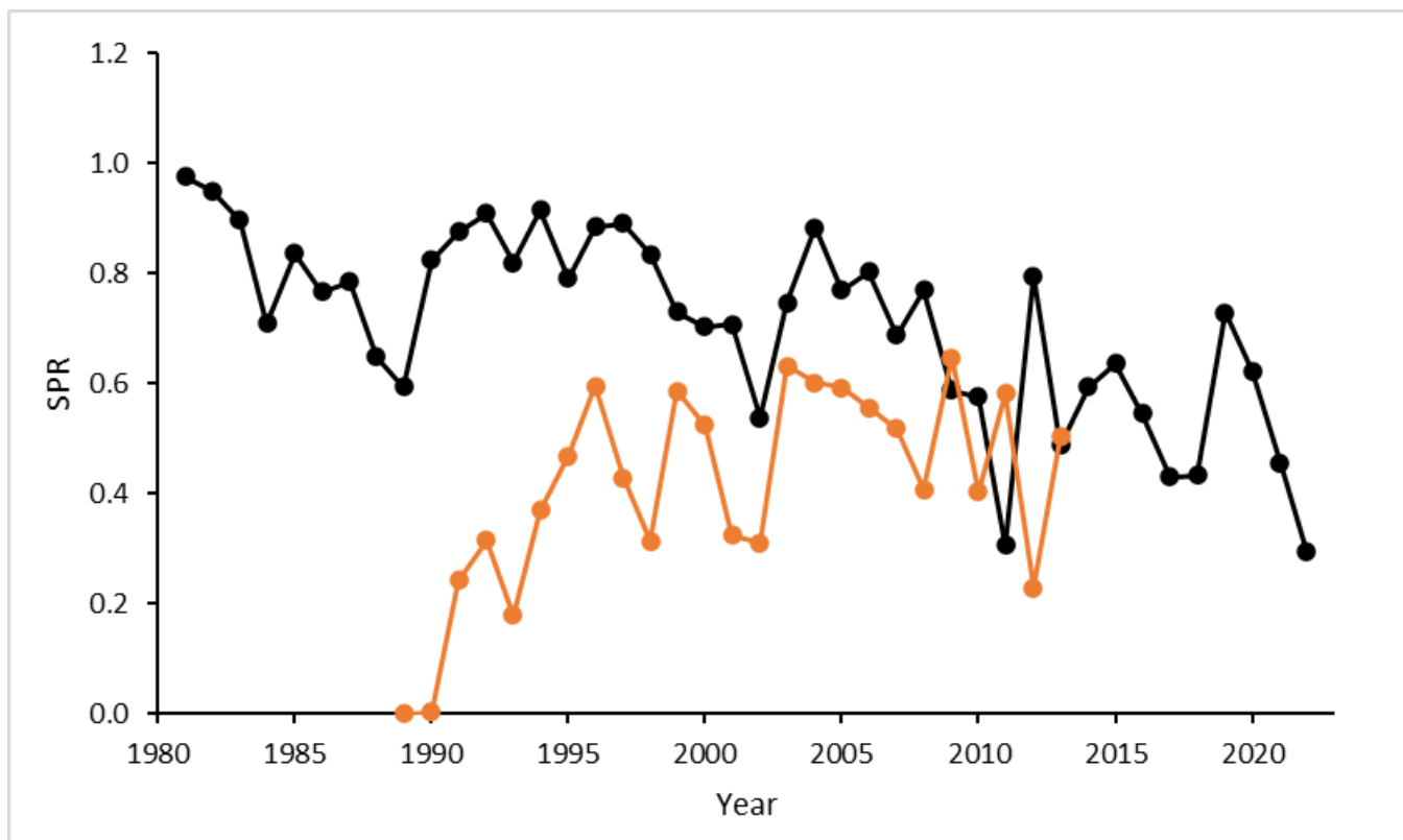
Figure 156. Spawning potential ratio estimates for the northern stock from the previous benchmark stock assessment using a custom statistical catch-at-age model (ASMFC 2017; orange) and the current benchmark assessment SS estimated selectivity model (black). Estimates from the previous assessment are for calendar years while estimates in the current assessment are for fishing years.
