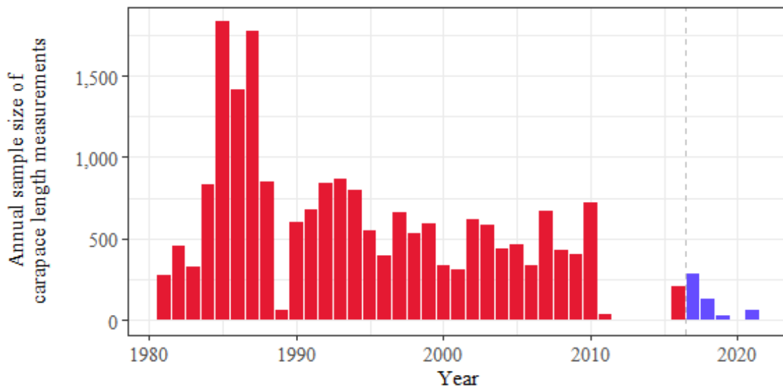
Figure 4.1: Annual counts of Caribbean Spiny Lobster carapace length samples from St. Croix used in the SEDAR 57 benchmark assessment (red) and update assessment (red and purple). The dashed vertical line denotes the terminal year of the SEDAR 57 benchmark assessment.
