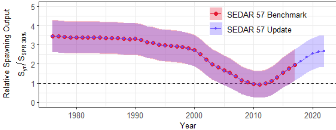
Figure 4.3: Relative spawning output of Caribbean Spiny Lobster for St. Croix. The line color relates to the source of the data. The shaded ribbons bound the 95th percent confidence intervals. The values plotted in purple nearly overlay the values plotted in red. Values below the horizontal dashed line indicate that the spawning output in a given year was smaller than the estimated S_{MSY Proxy} , defined in the SEDAR 57 benchmark assessment as S_{SPR 30\%} ; the spawning output associated with the stock at 30% of unfished stock size. Note: Unlike other Stock Synthesis estimates that are typically computed midyear, Stock Synthesis estimates of spawning output are “beginning of the year”. Therefore, an additional year is provided in these time series.
