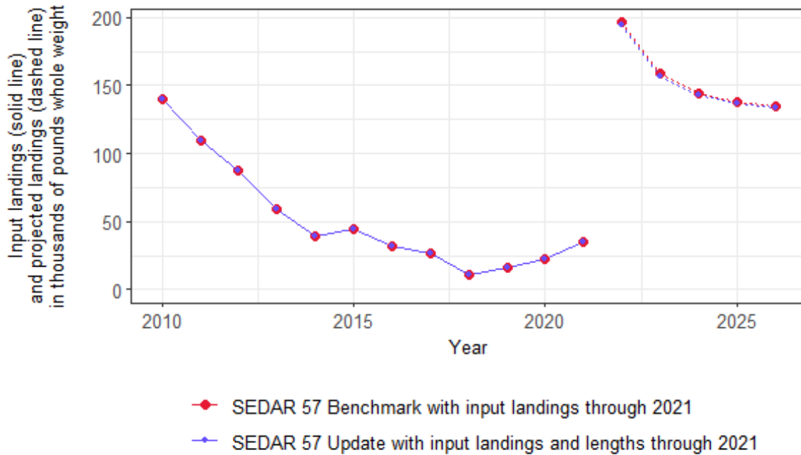
Figure 4.5: Caribbean Spiny Lobster landings and forecast OFLs for St. Croix plotted in pounds whole weight by year. The line color relates to the source of the data. The SEDAR 57 benchmark had input landings through 2021 and input lengths through 2016. The SEDAR 57 update had input landings and lengths through 2021. The line type refers to the status of the values plotted either as data inputs (solid lines) or as forecasted values from the stock assessment model projections (dashed lines). The data inputs plotted in purple exactly overlay those plotted in red while the forecast OFLs plotted in purple nearly exactly overlay those plotted in red.
