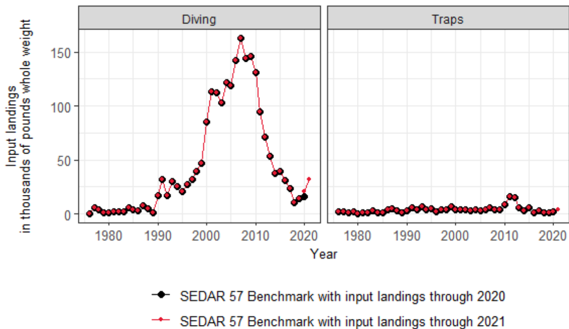
Figure 3.1: Caribbean Spiny Lobster landings from St. Croix are plotted in pounds whole weight by year and fleet. The color relates to the source of the data. The landings through 2021 are shown in red and the landings from the benchmark assessment through 2020 are shown in black. The values plotted in red overlay the values plotted in black in all years except 2019, 2020, and 2021.
