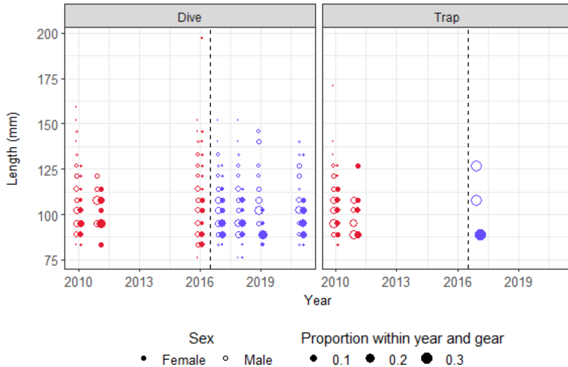
Figure 4.2: Relative proportion of male and female Caribbean Spiny Lobster carapace length samples by year and gear from St. Croix used in the SEDAR 57 benchmark assessment (red) and update assessment (red and purple). The dashed vertical line denotes the terminal year of the SEDAR 57 benchmark assessment. The proportions plotted are relative to the number of samples by year and gear, therefore, this plot does not indicate which gears and years have more total samples. The purpose of this plot is to indicate that the length compositions by year and gear of the update assessment (2017-2021) shown in purple were not unlike those from the most recent years of the SEDAR 57 benchmark assessment (2010-2016) shown in red.
