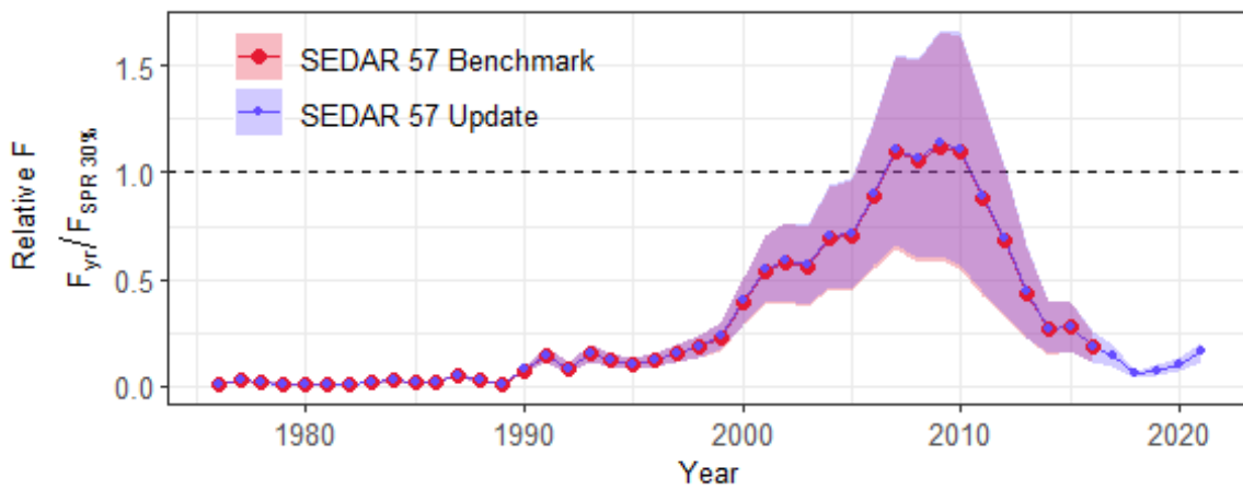
Figure 4.4: Relative fishing mortality of Caribbean Spiny Lobster for St. Croix. The line color relates to the source of the data. The shaded ribbons bound the 95th percent confidence intervals. The values plotted in purple nearly overlay the values plotted in red. Values above the horizontal dashed line indicate that the fishing mortality in a given year was larger than the estimated F_{MSY Proxy} , defined in the SEDAR 57 benchmark assessment as F_{SPR 30\%} ; the fishing mortality rate that would produce (in equilibrium) the same spawning output as the stock at 30% of unfished stock size.
