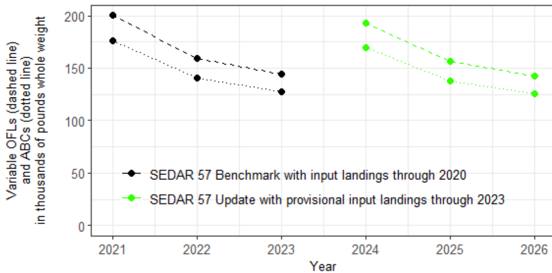
Figure 1.1: Caribbean Spiny Lobster variable-catch (annual) OFLs and ABCs for spiny lobster for St. Croix plotted in pounds whole weight. The line color relates to the source of the data. The line type refers to the forecasted values plotted from the stock assessment model projections as OFLs (dashed lines) or ABCs (dotted line).
