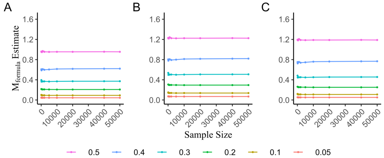
Figure A.2. Lineplots of calculated M_{\text{formula}} estimates (Y-axes) using the t_{1\%} approach across different sample sizes (X-axes). The color of the line indicates the M_{\text{model}} input value. All panels show similar trends with lower sample sizes producing slightly higher M_{\text{formula}} estimates, but estimates then level out once a sample size of approximately 5,000 is reached for Hoenig Combined (A), Then NLS (B), and Hamel Cope (C) longevity equations.
