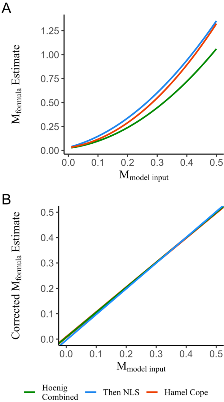
Figure 7. An example comparison of the average initial t_{99} M_{\text{formula}} estimates (Y-axis) generated from a sample size of 500 by each longevity equation in comparison to the respective M_{\text{model input}} rates (X-axis) from the simulation before (A) and after applying the correction (B). The data in 6A represent best fit polynomial trends in initial M_{\text{formula}} estimates before correction.
