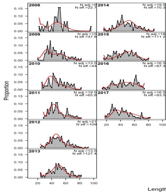
Figure 63. Observed and predicted length compositions for Gulf of Mexico Red Grouper caught in the Combined Video Survey for SEDAR 88 and SEDAR 61. Red lines represent predicted length compositions, while grey shaded regions represent observed length compositions. For SEDAR 88, 'N input' is the input sample size (trips) and 'N adj.' is the sample size after adjustment by the Dirichlet-Multinomial parameter. For SEDAR 61, 'N adj.' is the input sample size as the square root of the number of length observations ('N eff.' was not used).
