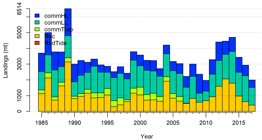
Figure 42. Expected landings by fleet for the SEDAR 88 OA Base Model and the SEDAR 61 Standard Base Model.
