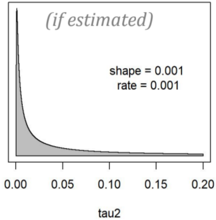
Figure 12: JABBA prior for observation error for all model configurations where estimated.
