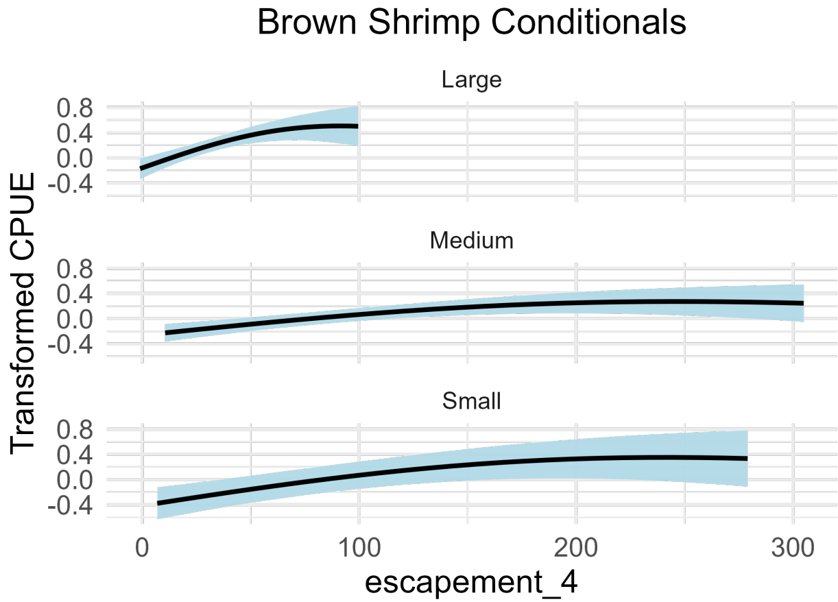
Figure 45: Length scale parameters for the 4th lag of abundance from the best performing model.
