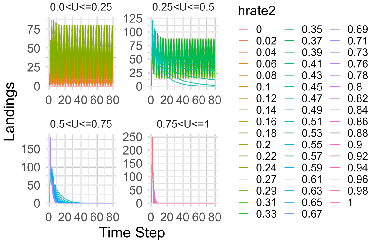
Figure 35: Variable harvest rate projections of landings from the best performing run for the Small shrimp population.
