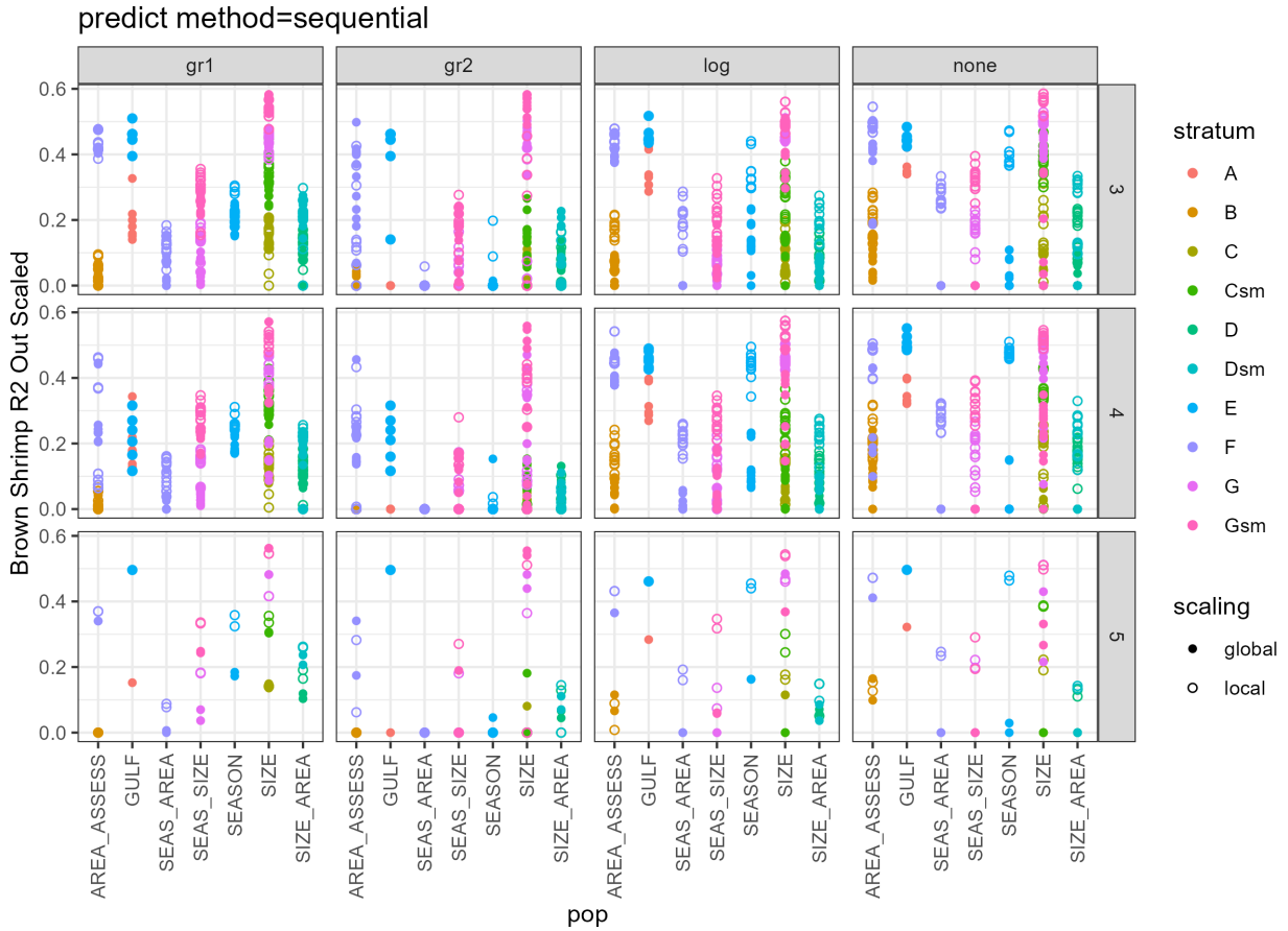
Figure 27: “Sequential” out-of-sample R2 fit statistic resulting from each model run. Facet columns show results based on different data transformations. Facet rows show results based on the embedding dimension. Within each facet, the x axis groups the models by the type of aggregation (spatial, size, season, or a combination). Models that locally scaled the data performed better than models that scaled globally for most transformations, which aligns with how we understand the data (e.g. populations are not directly comparable as defined here).
