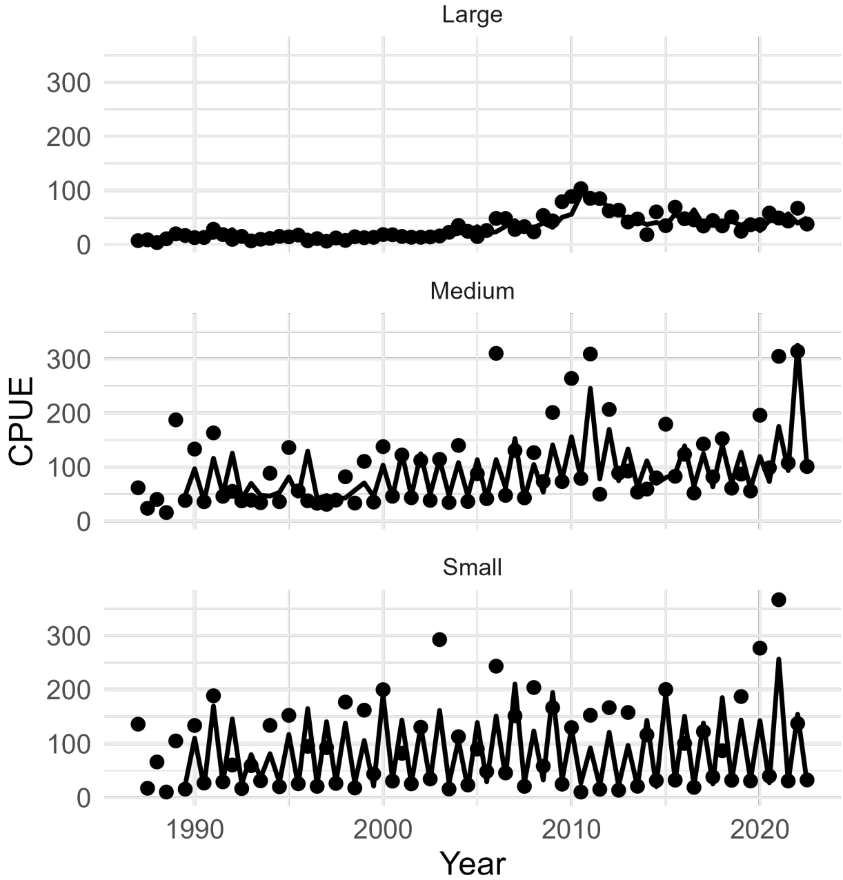
Figure 48: EDM model fits for the best performing run in raw units of SEAMAP CPUE.
