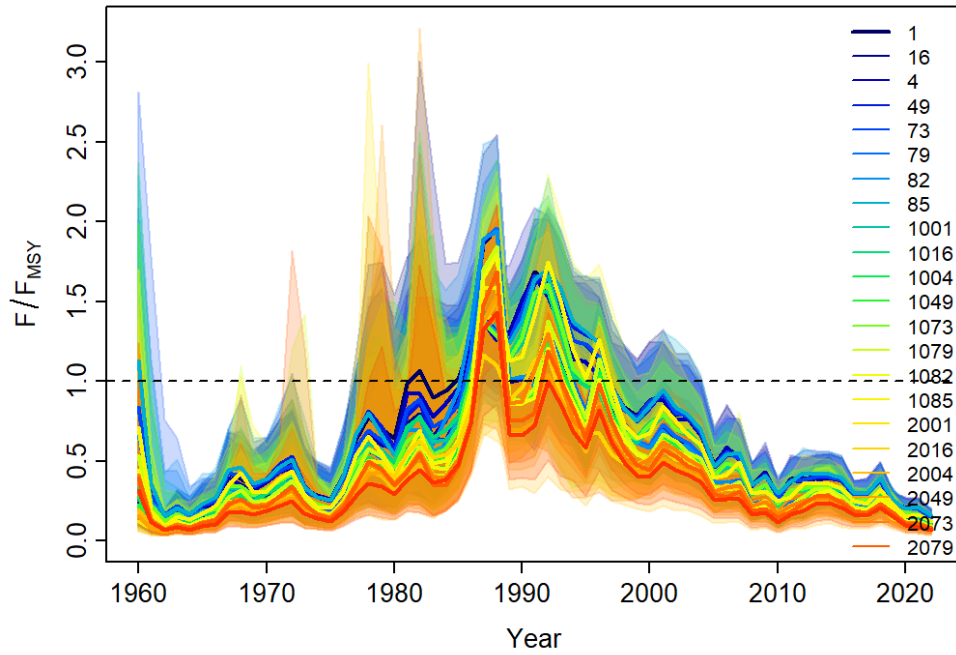
Figure 16: F/F_{MSY} estimates for Brown Shrimp across runs.
