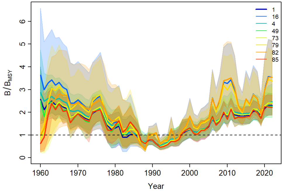
Figure 25: B/B_{msy} trajectories for top performing JABBA models, where Run 1 was the best model that passed most of the diagnostic tests.
