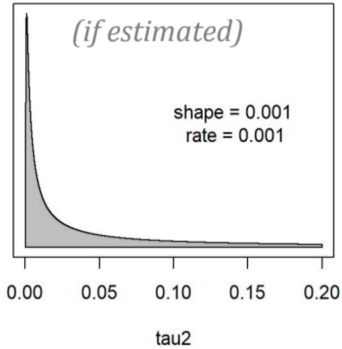
Figure 14: JABBA prior for observation error variance for all model configurations where estimated.
