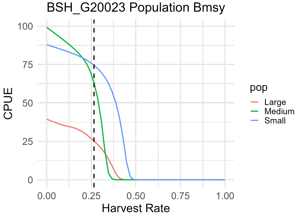
Figure 36: Average CPUE by harvest rate for individual populations for the best performing run. The dashed line indicates the seasonal harvest rate where MSY occurs, indicating population-wide Bmsy in units of CPUE for each population.
