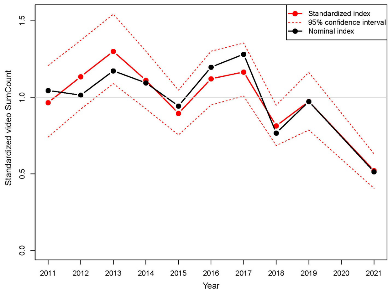
Figure 7. Gray triggerfish relative standardized index (red line and points) with 2.5% and 97.5% confidence intervals (red dashed lines) and the relative nominal index (black line with points) from SERFS video data using a zero-inflated negative binomial model.
