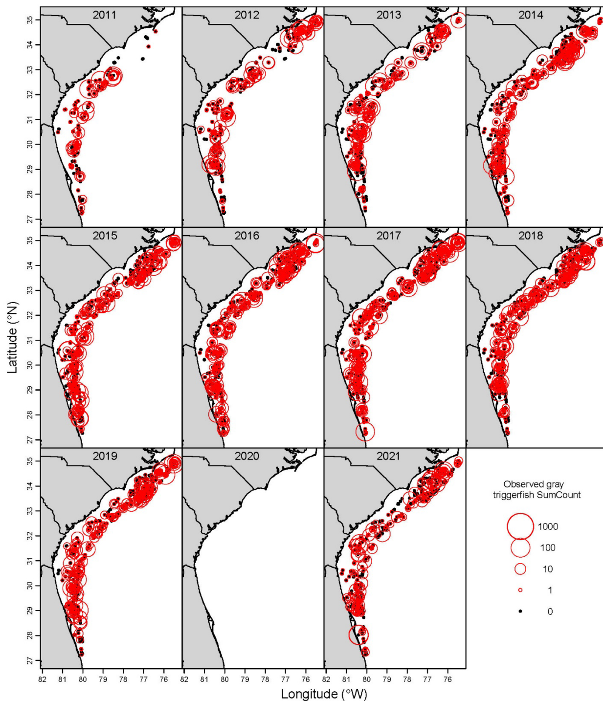
Figure 2. Bubble plots of gray triggerfish SumCounts from videos collected by the Southeast Reef Fish Survey, 2011–2021. Black points show locations where gray triggerfish were not observed on video and red bubbles show where gray triggerfish were observed on video, with the size of the bubbles scaled to their video SumCount . Note that points overlap often. No sampling occurred in 2020 due to the covid-19 pandemic.
