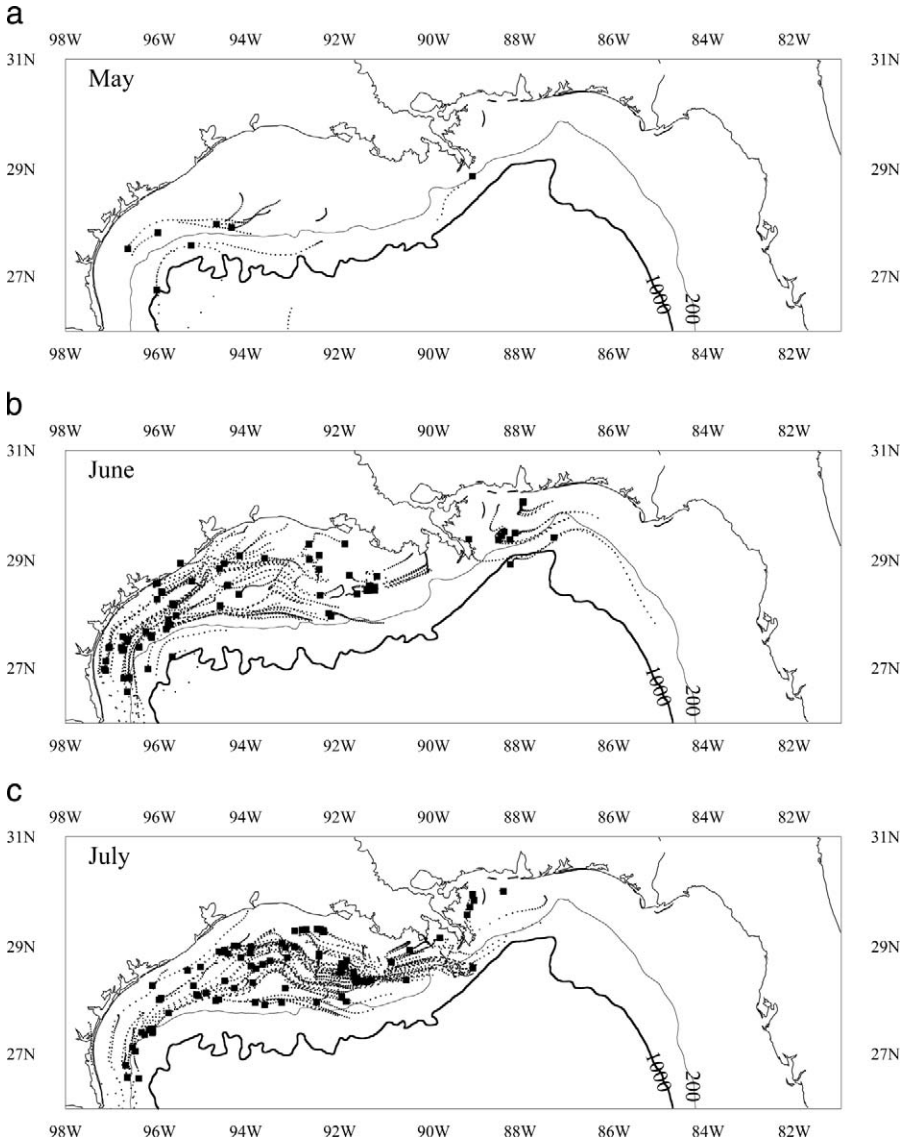
FIGURE 6.—Daily surface drift points from SEAMAP capture points during (a) May, (b) June, (c) July, (d) August, (e) September, and (f) October. Drifts are computed for 21 d forward and 11 d backward.
