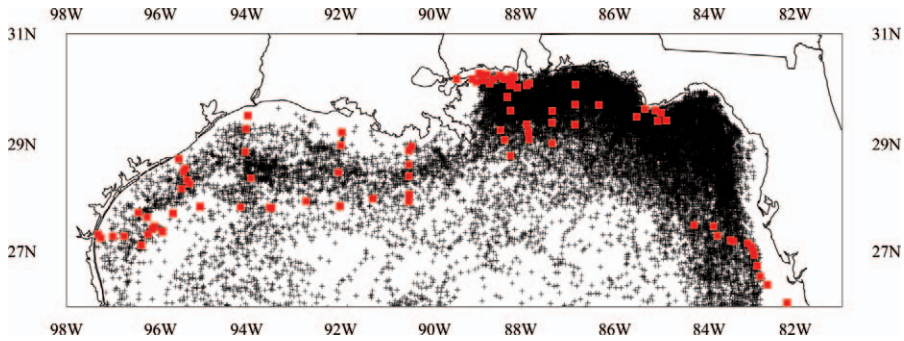
FIGURE 3.—Locations of observational currents. The small black crosses mark the locations of daily vectors from satellite-tracked drifters, the red squares the locations of moored current meters.
