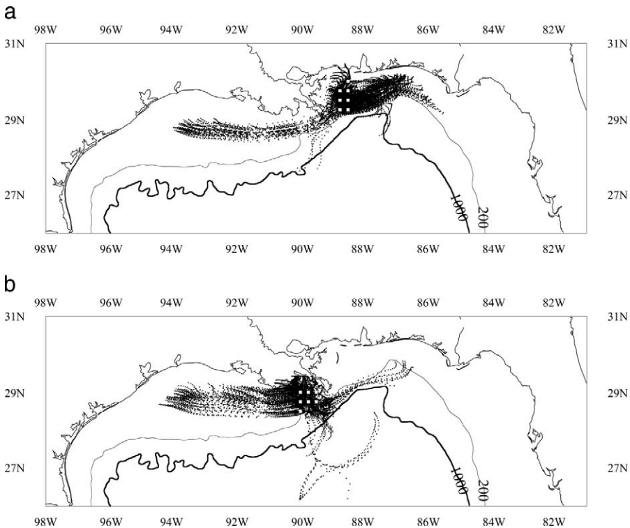
FIGURE 8.—Daily drift points launched from artificial grids (white squares) (a) east and (b) west of the Mississippi River delta. Launches were made every 3 d from May to October. Note that in (a) the tracks principally crossed within the 200-m isobath and onto the middle of the Louisiana–Texas shelf, whereas in (b) they principally crossed the delta outside of the 200-m isobath and onto the upper slope of the Mississippi Bight.
