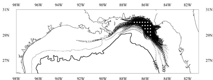
FIGURE 9.—Daily drift points launched from an artificial grid west of the Apalachicola peninsula. Launches were made every 3 d from May to October.
