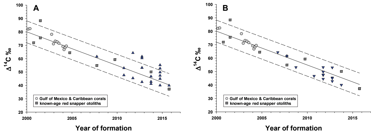
Figure 4. Gulf of Mexico gray triggerfish eye lens core \Delta^{14}\text{C} (blue triangles) versus estimated year of formation (birth year) for A) spine-derived and B) otolith-derived age estimates overlain on regional coral and known-age red snapper otolith samples. Solid line is linear regression fit to coral and red snapper time series. Dashed lines are 95% prediction intervals.
