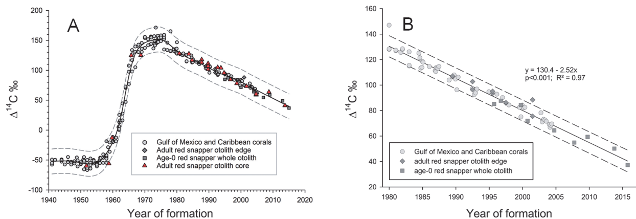
Figure 2. A) Scatterplot of regional coral plus known-age Gulf of Mexico red snapper (adult edge and whole age-0) otolith \Delta^{14}\text{C} values versus year of formation. The solid line is a loess regression fit to the combined data; dashed lines are 95% prediction intervals. Adult red snapper otolith core data plotted for samples that were undergoing age validation. B) Linear regression fit to coral and known-age red snapper otolith \Delta^{14}\text{C} values versus year of formation for the linear decline portion of the time series (source for both: Barnett et al. 2018).
