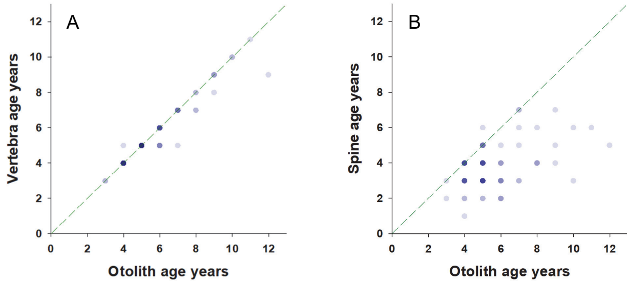
Figure 3. Age estimate comparisons between A) vertebral and otolith sections and B) spine and otolith sections for gray triggerfish sampled in US Atlantic waters. In each plot, n = 72 . Symbol shading indicates sample size, which ranges from 1 (lightest) to 12 (darkest) age pairs.
