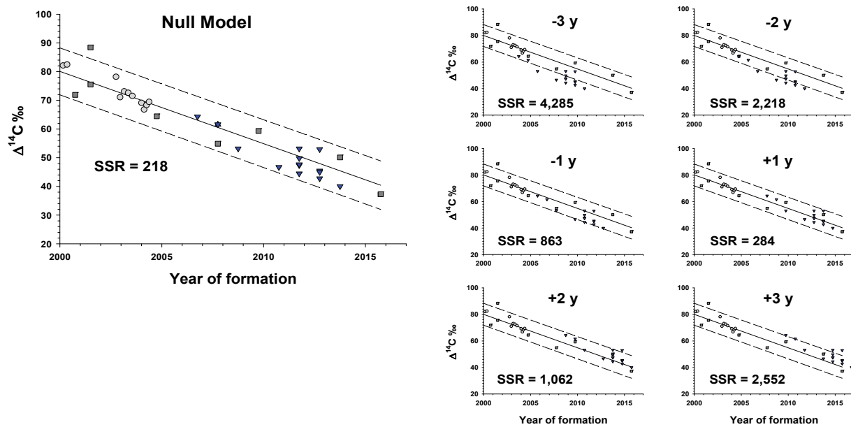
Figure 6. Results from Kastelle et al. (2008) approach to estimate ageing bias based on the bomb radiocarbon chronometer for Gulf of Mexico gray triggerfish spine-derived age estimates.
