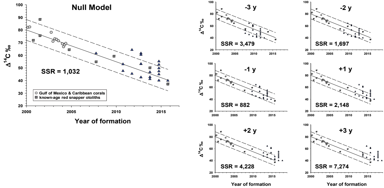
Figure 5. Results from Kastelle et al. (2008) approach to estimate ageing bias based on the bomb radiocarbon chronometer for Gulf of Mexico gray triggerfish spine-derived age estimates.
