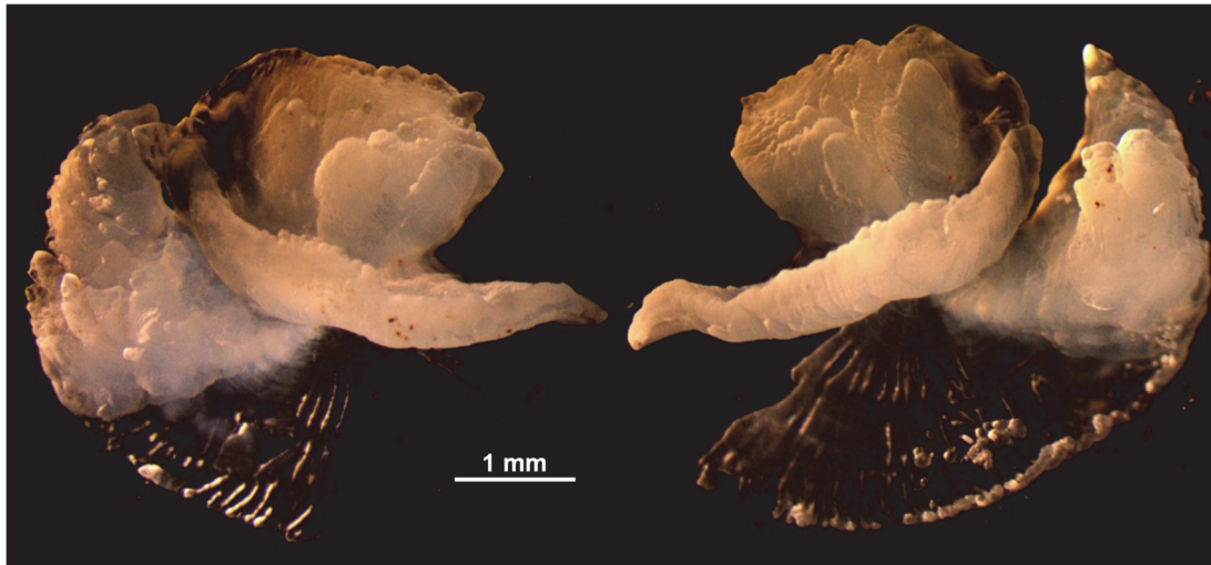
Figure 1. Digital images of a pair of gray triggerfish sagittal otoliths viewed with a light microscope and demonstrating their small size and fragile nature.
