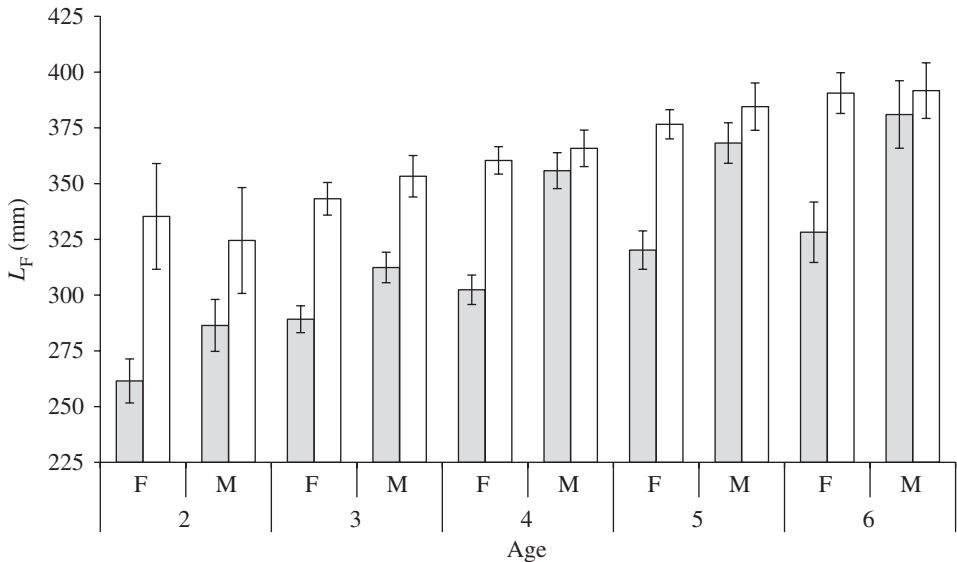
FIG. 3. Mean \pm 95% C.I. sex-specific fork length ( L_F ) at age for Balistes capriscus sampled on fishery-independent surveys ( \square ) or from recreational landings ( \square ) in the northern Gulf of Mexico. F, female; M, male.
