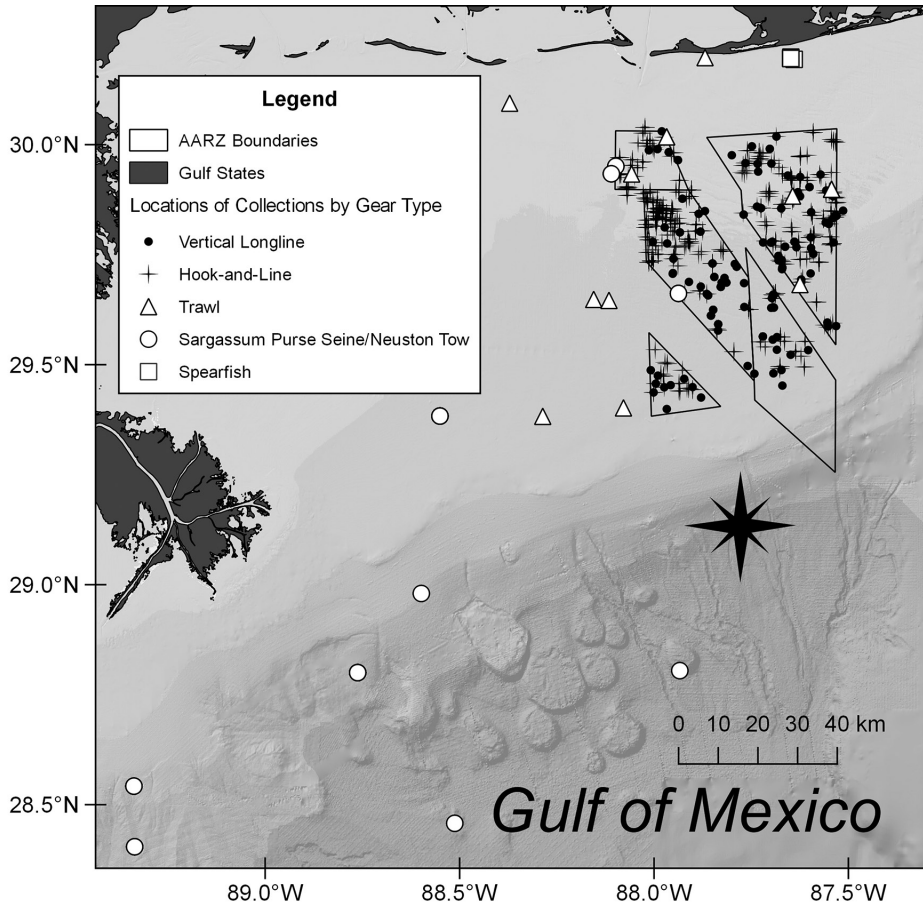
Figure 2. Collection locations of gray triggerfish, Balistes capricus , sampled for age analysis using multiple gear types both inside and outside the Alabama Artificial Reef Zone from 1999 to 2017.
