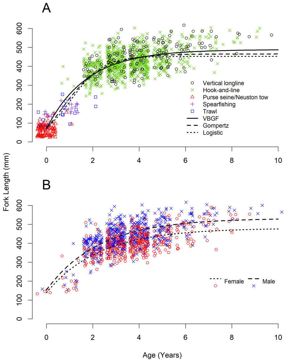
Figure 5. (A) Results of the multimodel framework approach. Each point represents the length and age data for a single gray triggerfish, Balistes caprisicus . (B) Gray triggerfish sex-specific von Bertalanffy growth function.
