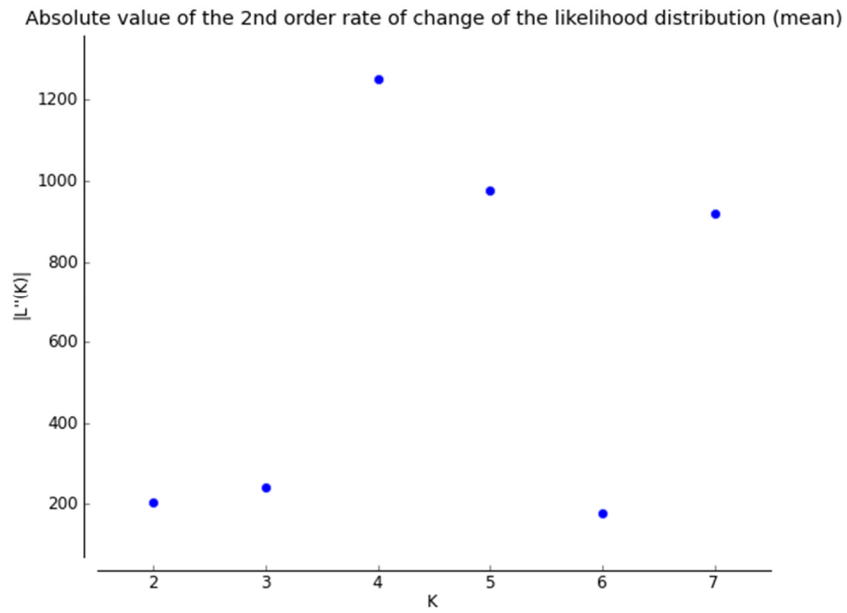
Figure 3. STRUCTURE Harvester result output for Absolute Value of the Second Order Rate of Change in the Mean Likelihood Distribution from the By State, Round 2 (no SC Inshore samples included) analysis indicating K=4.
