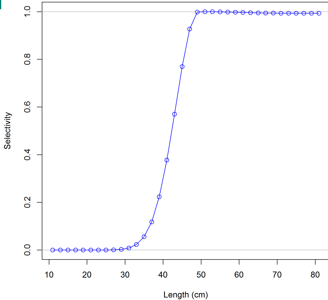
Ending year selectivity for CM_LL_3
