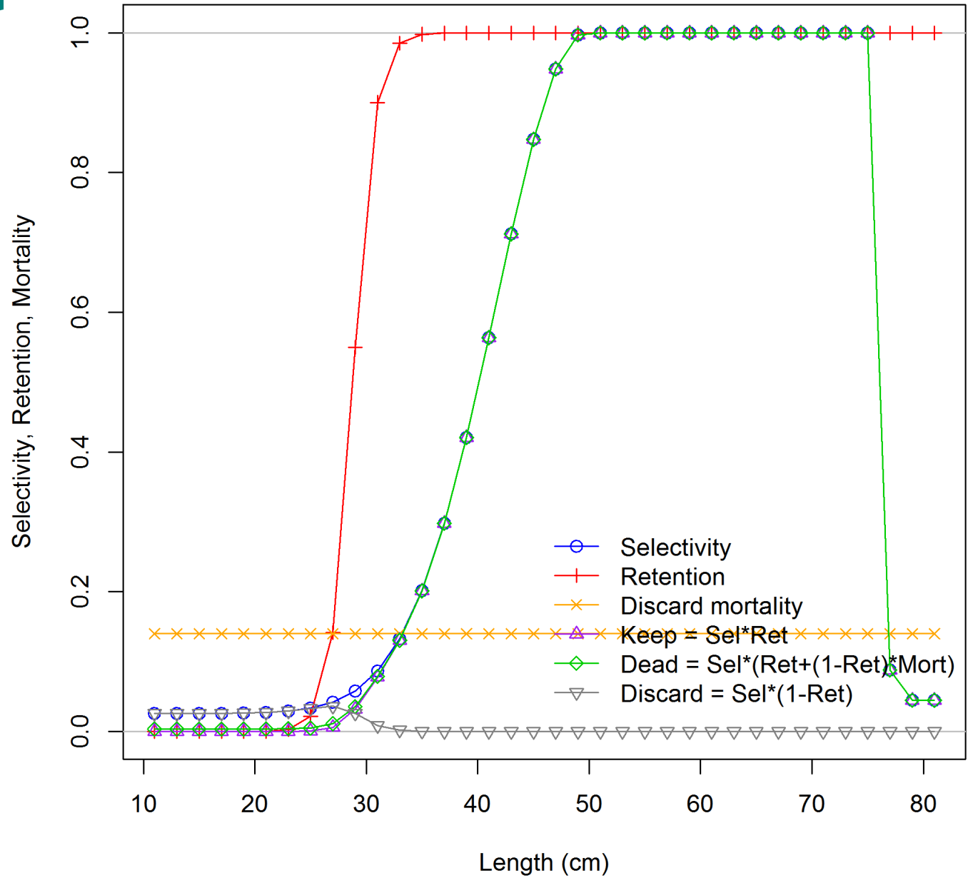
Ending year selectivity for CHL_nMC_2
