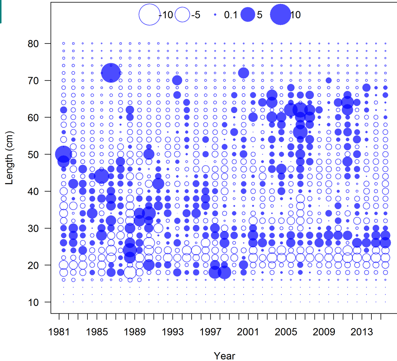
Pearson residuals, sexes combined, retained, REC_PR_4 (max=8.87)
