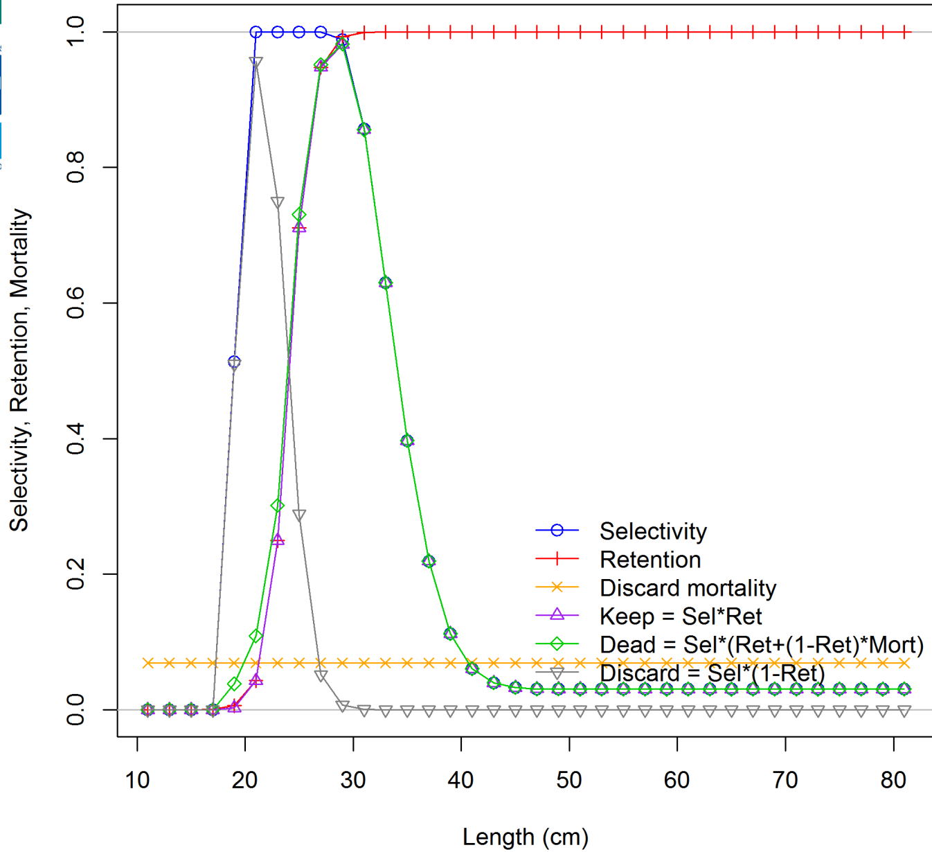
Ending year selectivity for Rec_Shore_5
