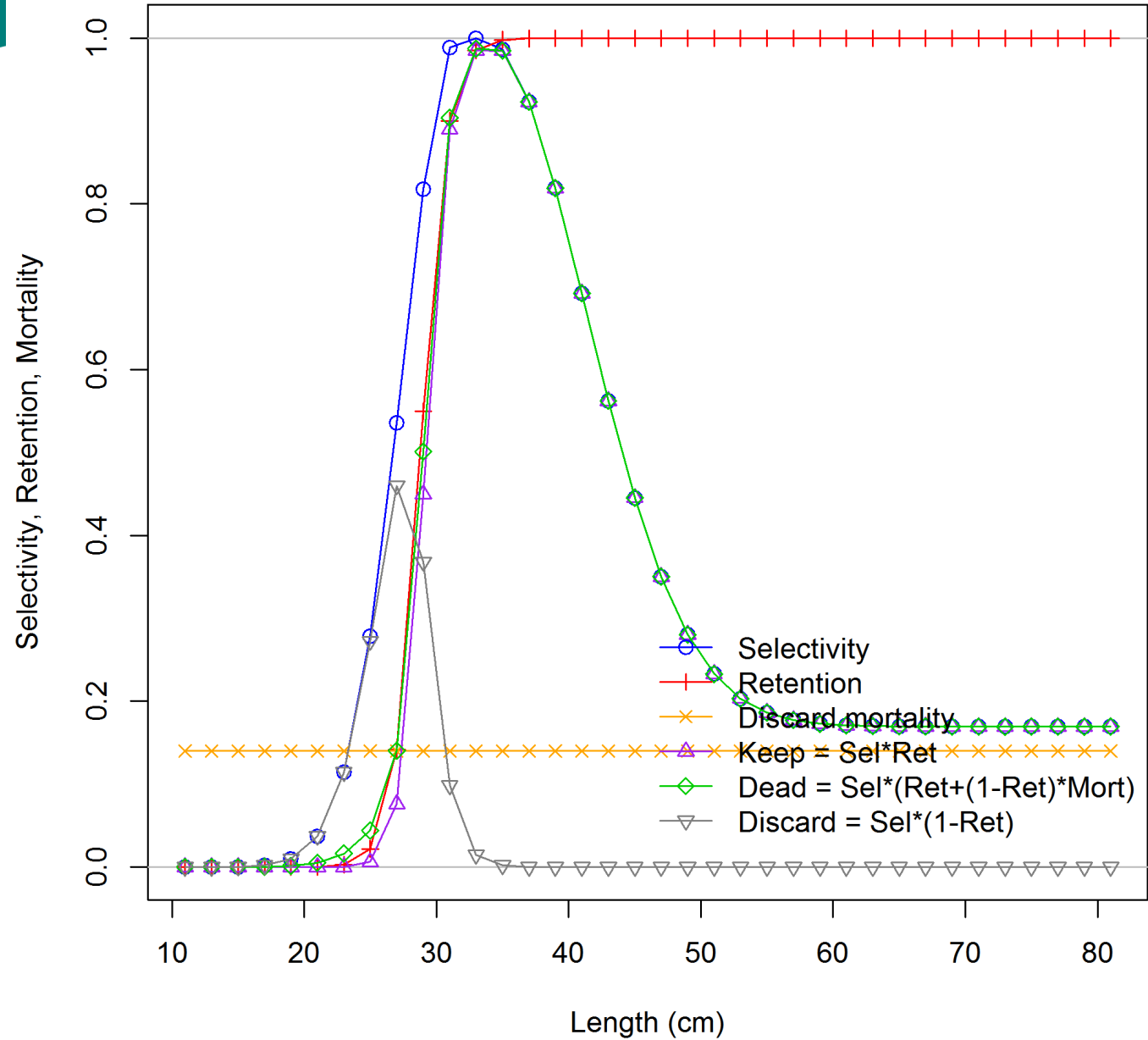
Ending year selectivity for CHL_MC_1
