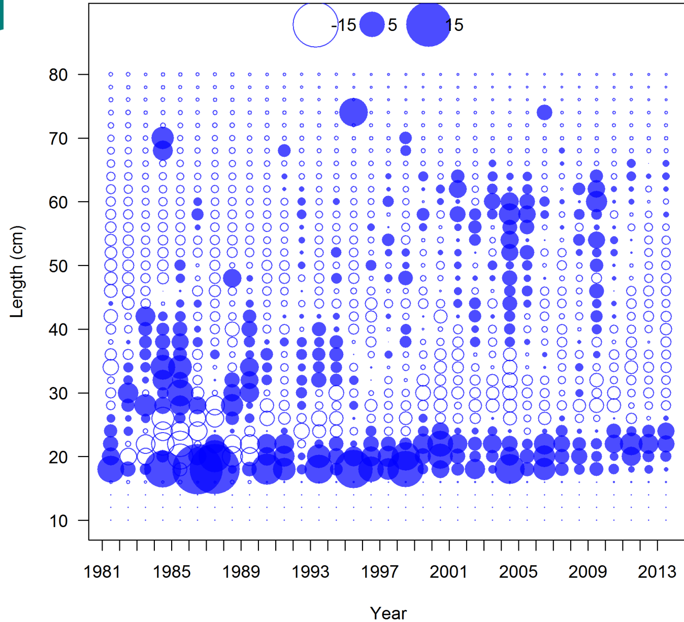
Pearson residuals, sexes combined, retained, Rec_HB_CBT6 (max=18.89)
