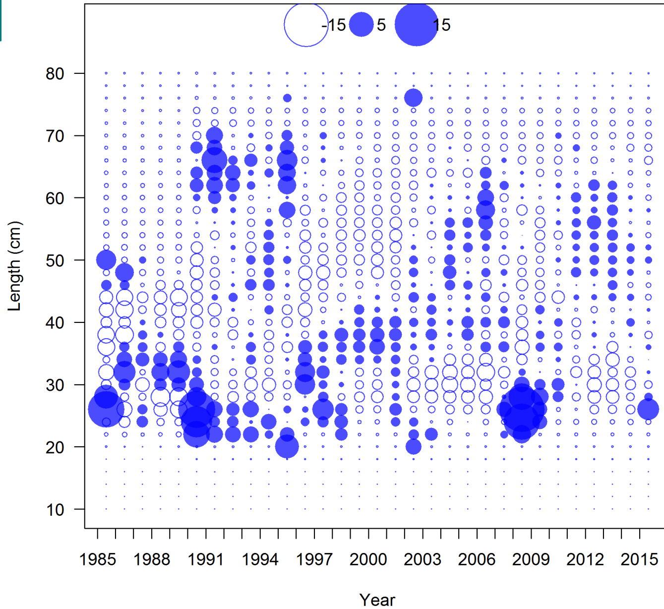
Pearson residuals, sexes combined, retained, CHL_nMC_2 (max=16)
