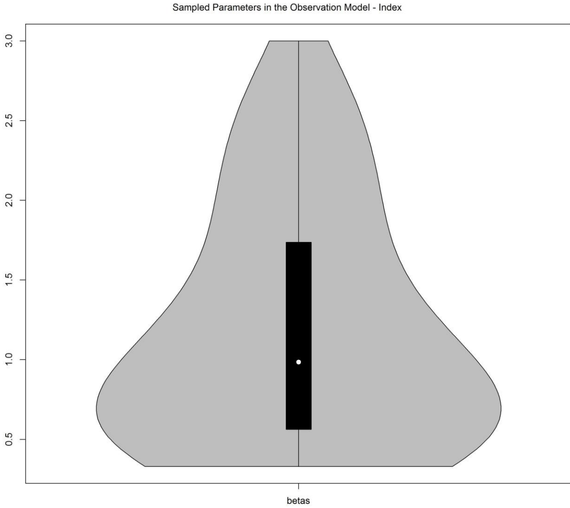
Figure 6. Sampled parameters in the observation model for the index of abundance. Betas is a parameter controlling hyperstability/hyperdepletion.
