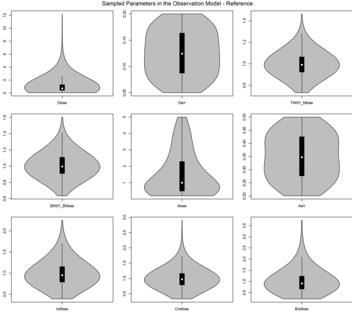
Figure 8. Sampled parameters in the observation model for the reference. Parameters as defined in Figure 3 caption, with exception of D = Depletion, A = abundance, Iref = reference index level, Cref = reference catch level, and Bref = reference biomass level. Bias refers to an inaccuracy in an observed parameter that occurs for the duration of a simulation.
