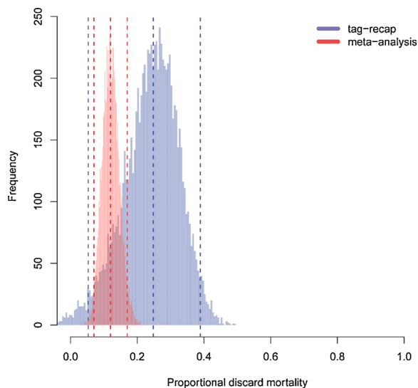
Fig. 3. Posterior probability distributions (posteriors) for the estimated overall rate of discard mortality in a hook and line recreational fishery for dolphinfish Coryphaena hippurus sampled in the southeastern US. The blue histogram is the posterior from a published tag-recapture ('tag-recap') study to estimate discard mortality through fitting a relative risk model to dolphinfish released in two different conditions (see Rudershausen et al., 2019 for details). The posterior from a two-step approach ('meta-analysis': this study) using published data and dockside sampling to estimate discard mortality is shown in the red histogram. Blue and red vertical lines (left to right) are 2.5, median, and 97.5 credible intervals for the respective posteriors.
