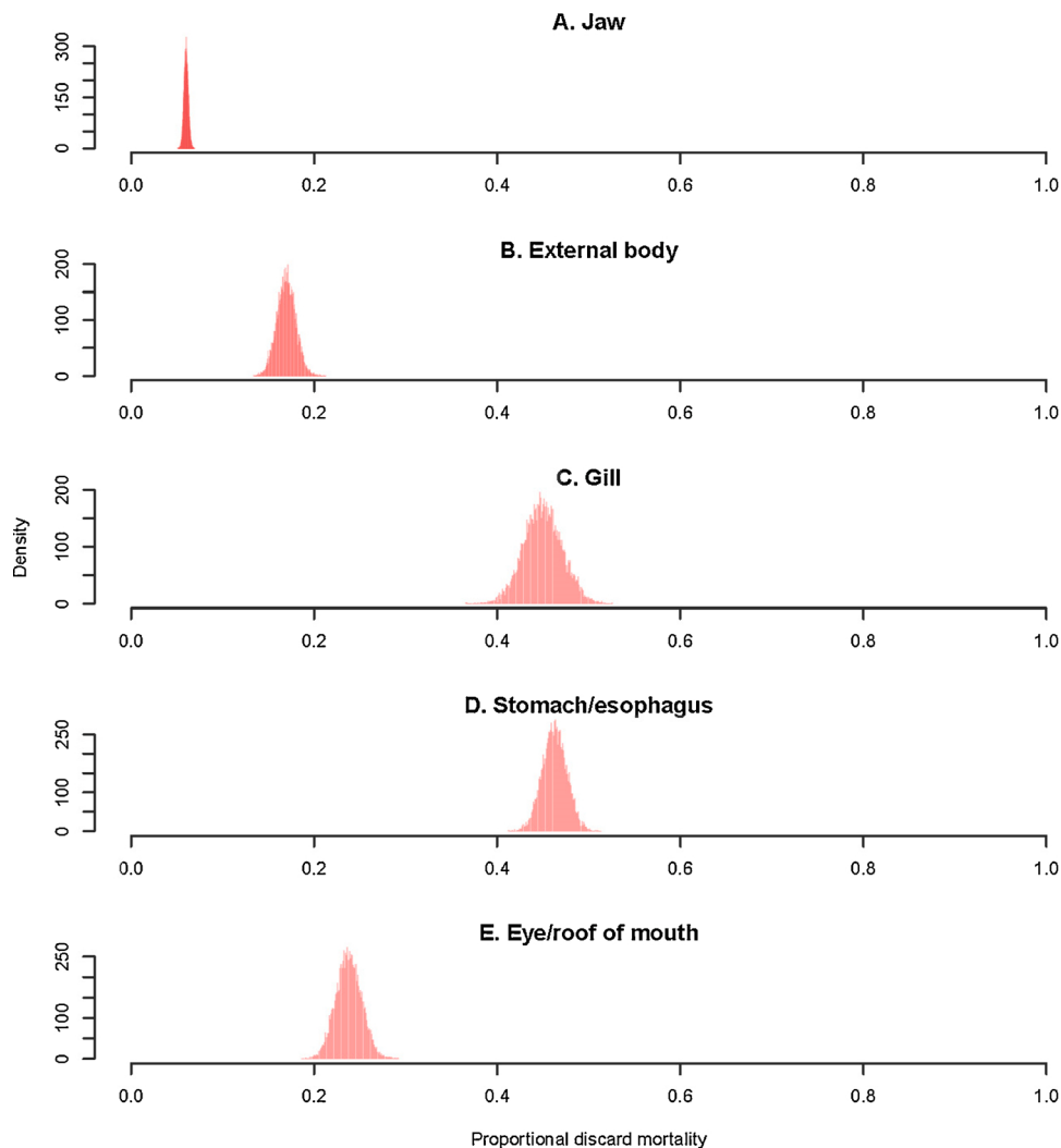
Fig. 1. Posterior probability distributions (posteriors) for the estimated proportional discard mortality of fishes hooked in five anatomical locations, based on data obtained from published literature. Each histogram displays the density (y-axis) of discard mortality estimates (x-axis) for retained updates across three chains (9000 retained updates total).
