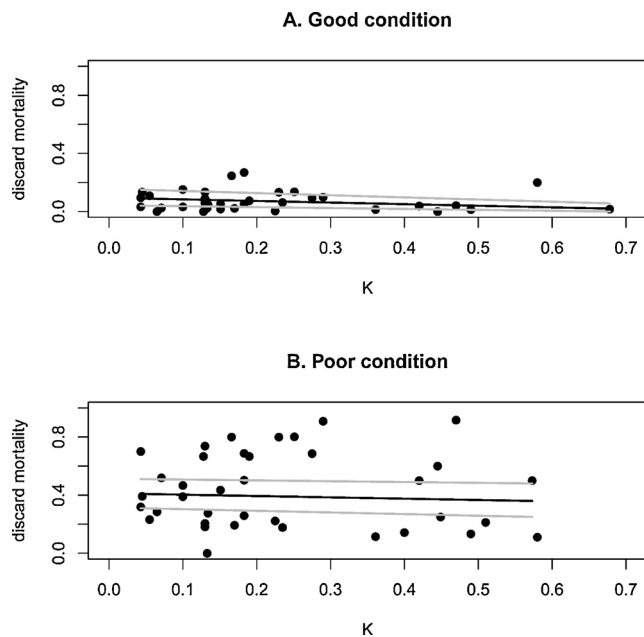
Fig. 2. Observed (circles) and predicted values (lines) for relationship between the Brody growth coefficient ( K ) (x-axis) and proportional discard mortality (y-axis) for a variety of fish species from a meta-analysis of discard mortality. Predictions include the median (black line) as well as 2.5 (lower gray line) and 97.5 credible values (upper gray line). Data and predictions are broken down between good-hooking condition (panel A) and poor-hooking condition (panel B). Predictions were obtained by fitting a binomially distributed model that included the effects of hooking condition and K and their interaction. The scale of the y-axis is identical between panels.
