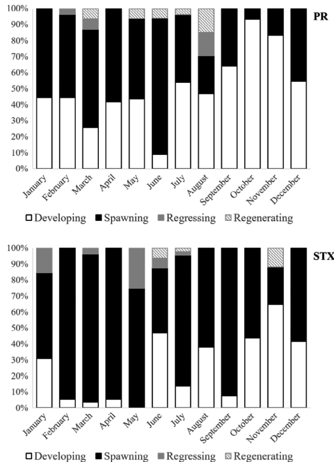
FIGURE 8. Reproductive seasonality of male Queen Triggerfish in Puerto Rico (PR) and St. Croix (STX). Monthly proportions of individual males in each reproductive phase are presented.
