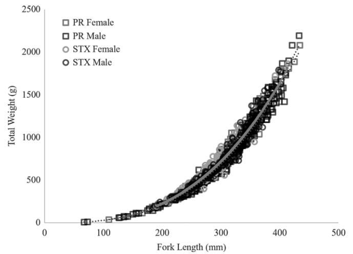
FIGURE 2. Queen Triggerfish FL versus weight for females and males from Puerto Rico (PR) and St. Croix (STX).
