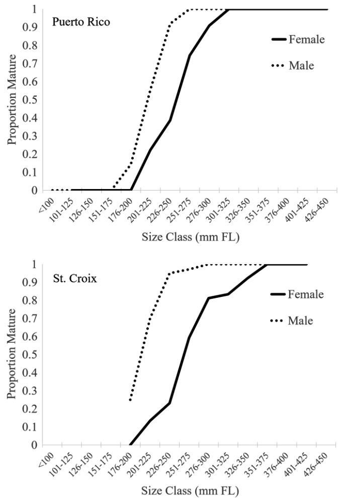
FIGURE 5. Female and male 50% sexual maturity curves for Queen Triggerfish sampled from Puerto Rico and St. Croix.
