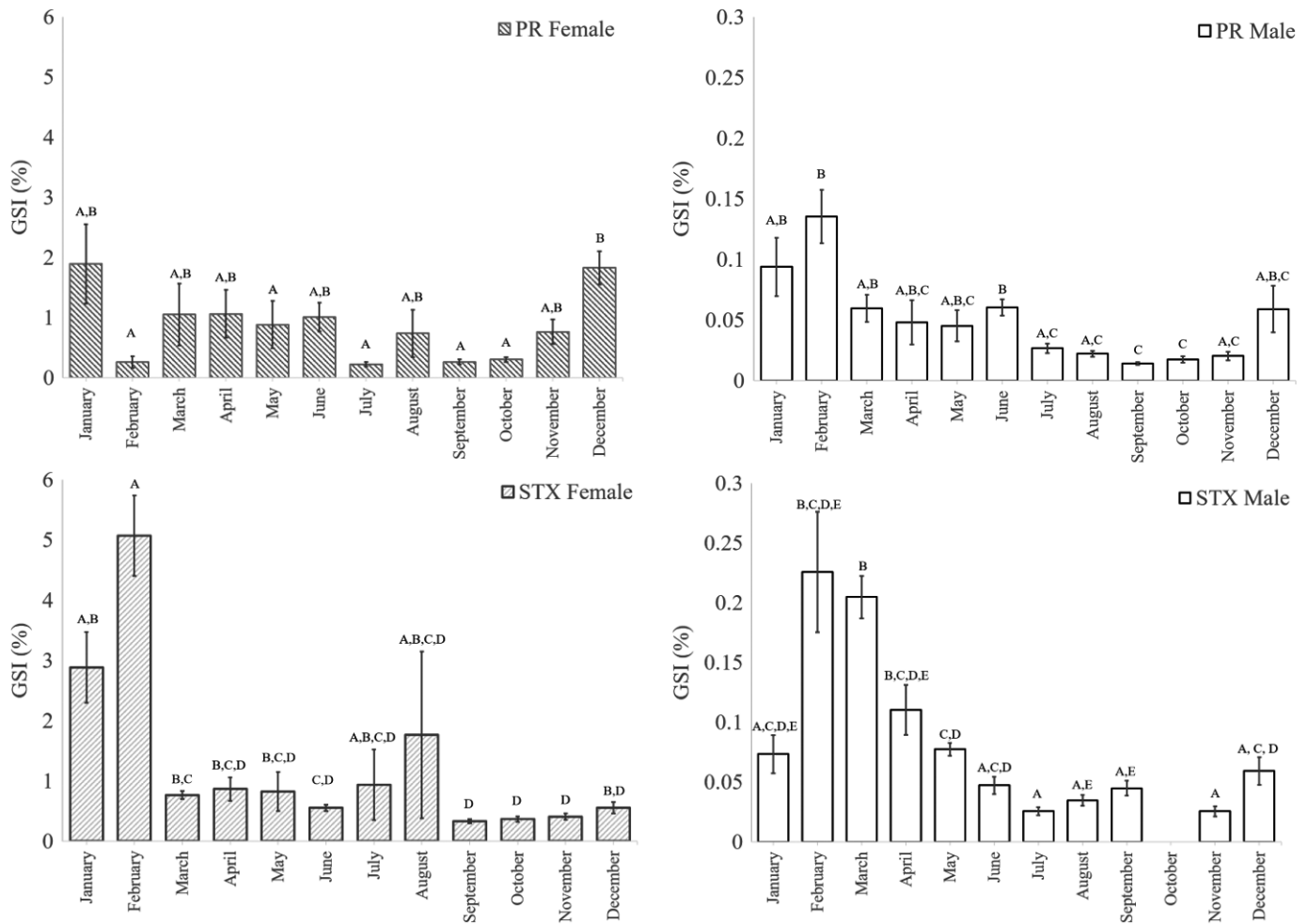
FIGURE 6. Mean ( \pm SE) monthly gonadosomatic index (GSI) values for sexually mature Queen Triggerfish females and males from Puerto Rico (PR) and St. Croix (STX). Letters within each graph indicate significant differences in monthly mean GSI for pairwise comparisons ( \alpha = 0.05 ). No mean value is presented for STX males in October because the scale for weighing gonads (nearest 0.01 g) malfunctioned before testes could be weighed.
