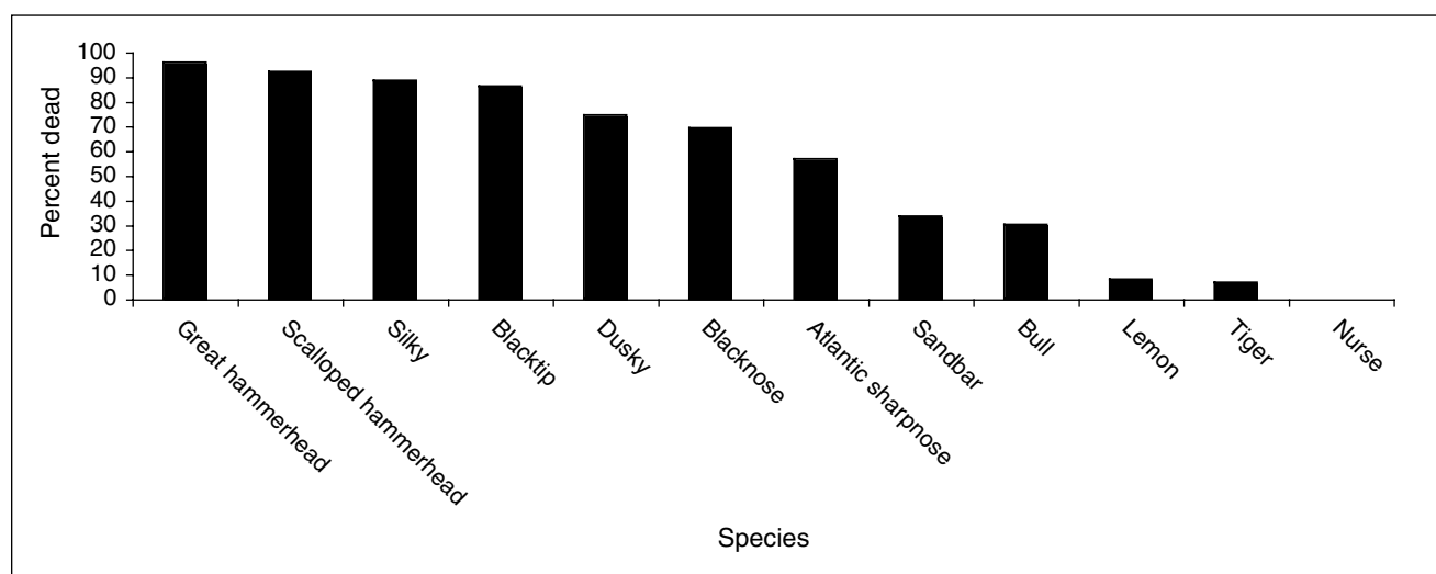
Figure 9.—Mortality rates for shark species (at the vessel) commonly observed caught in the BLL fishery.
