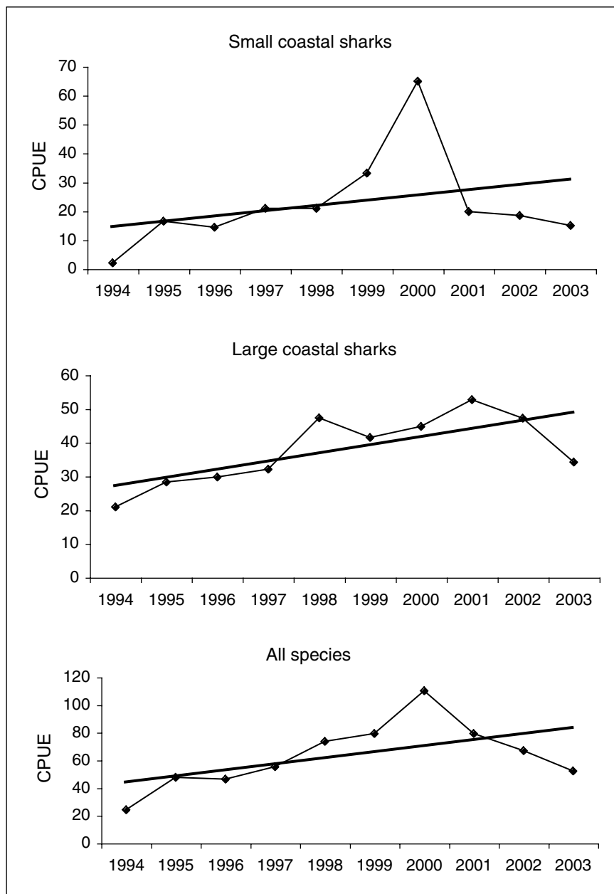
Figure 11.—Annual CPUE (sharks per 10,000 hook hours) for large coastal sharks, small coastal sharks, and all species combined.
