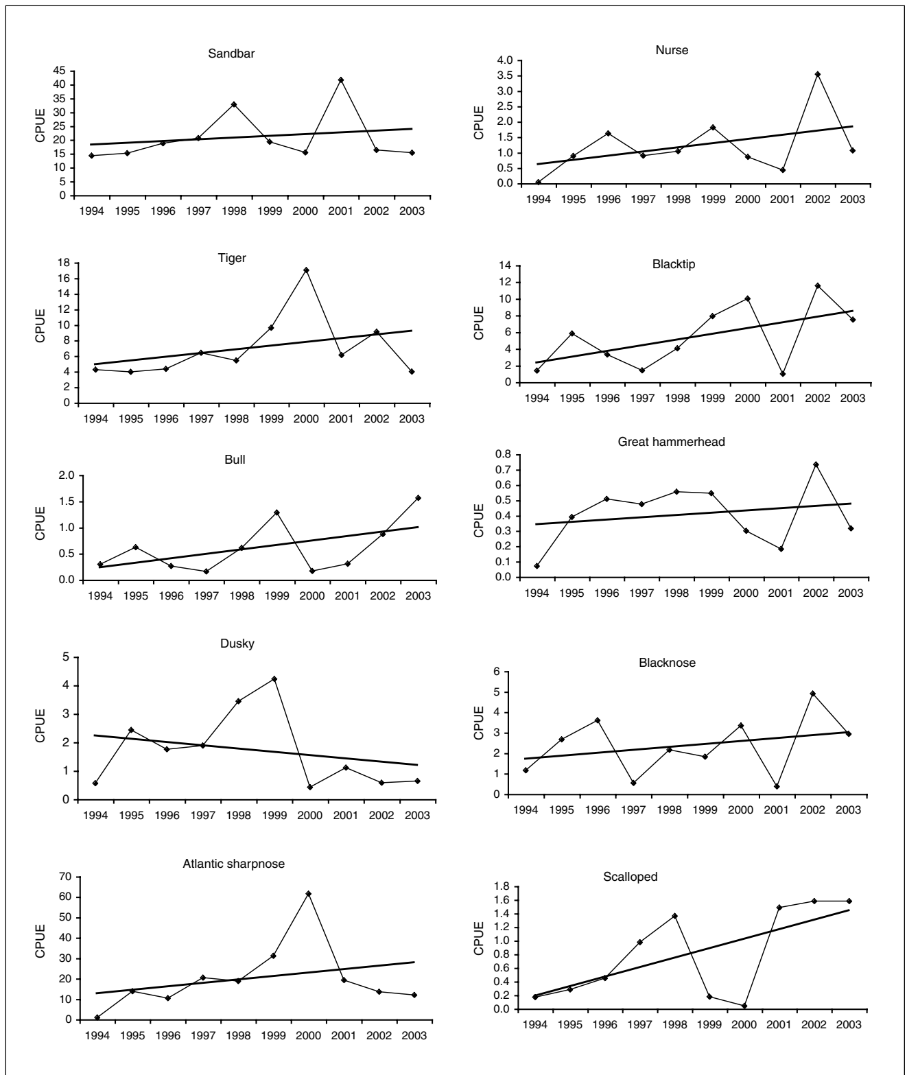
Figure 10.—Annual CPUE (sharks per 10,000 hook hours) by year for shark species commonly observed caught in the BLL fishery. The y-axis ranges are different for individual species.
