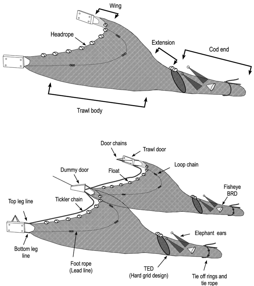
Figure 3.—Typical gear components for U.S. southeastern shrimp vessels.
