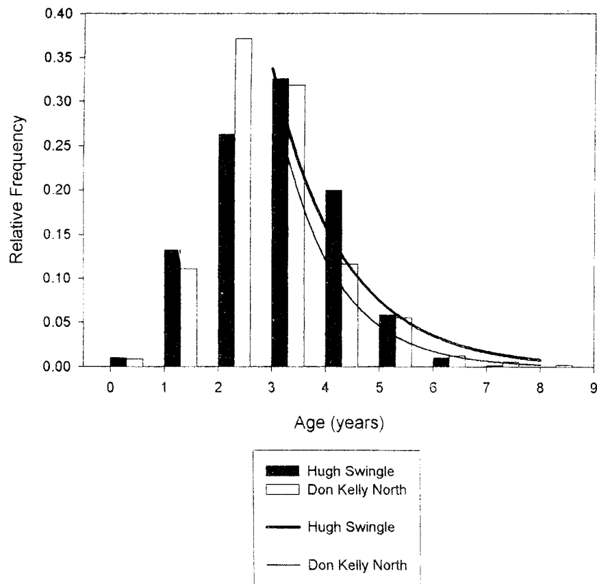
Figure 3.26. Age-frequency and decay of frequency of gray triggerfish over time for fish captured in the Hugh Swingle and Don Kelly North General Permit Areas.
