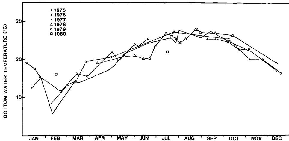
Figure 5. Bottom water temperature, September 1975 through July 1980.
