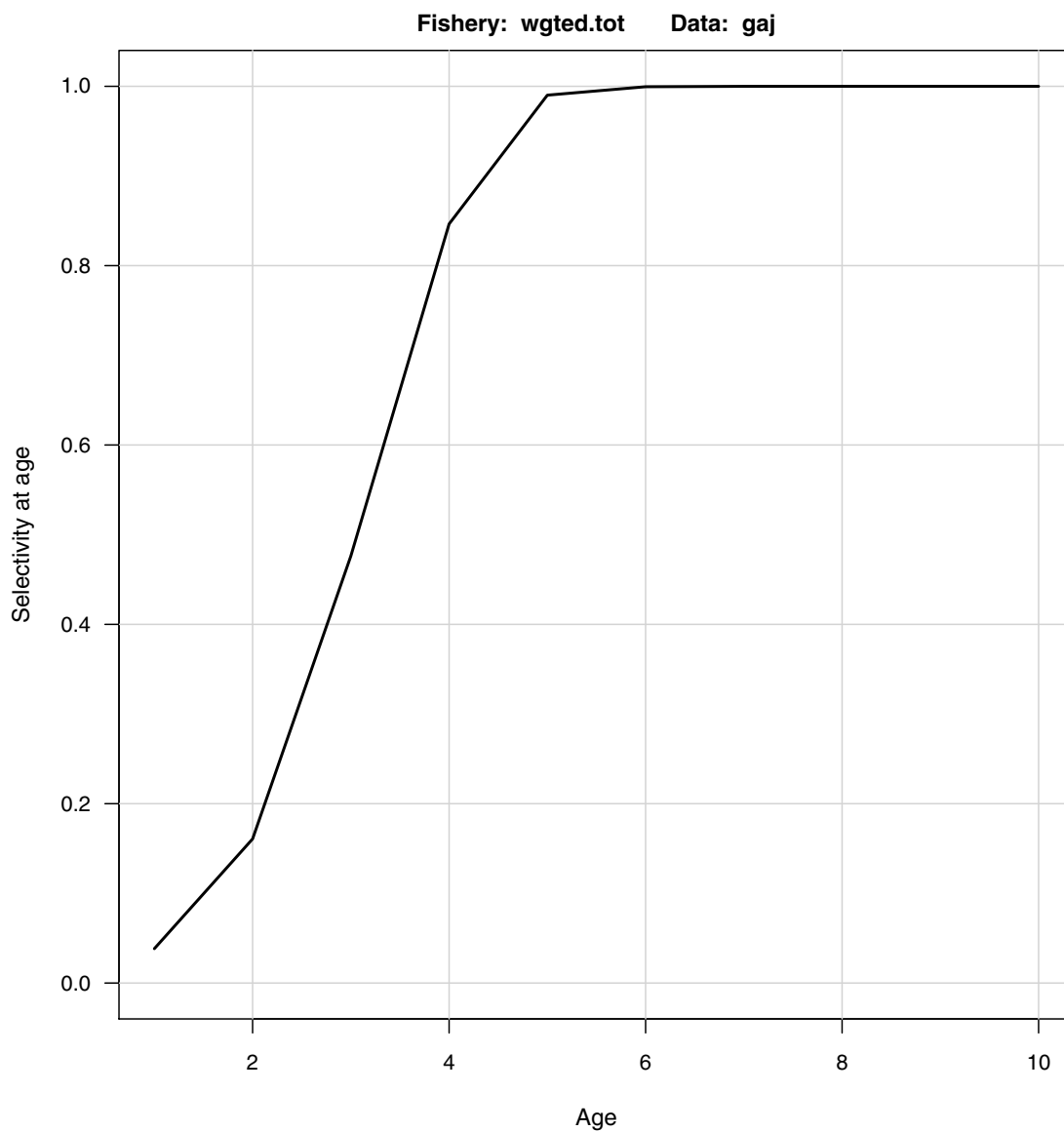
Figure 3.36. Greater amberjack- Base run: Estimated selectivity for landed and discarded fish used in MSY calculations computed from the 3-year geometric mean weighted fishing mortality rates ( F ) for all fishery gear types.
