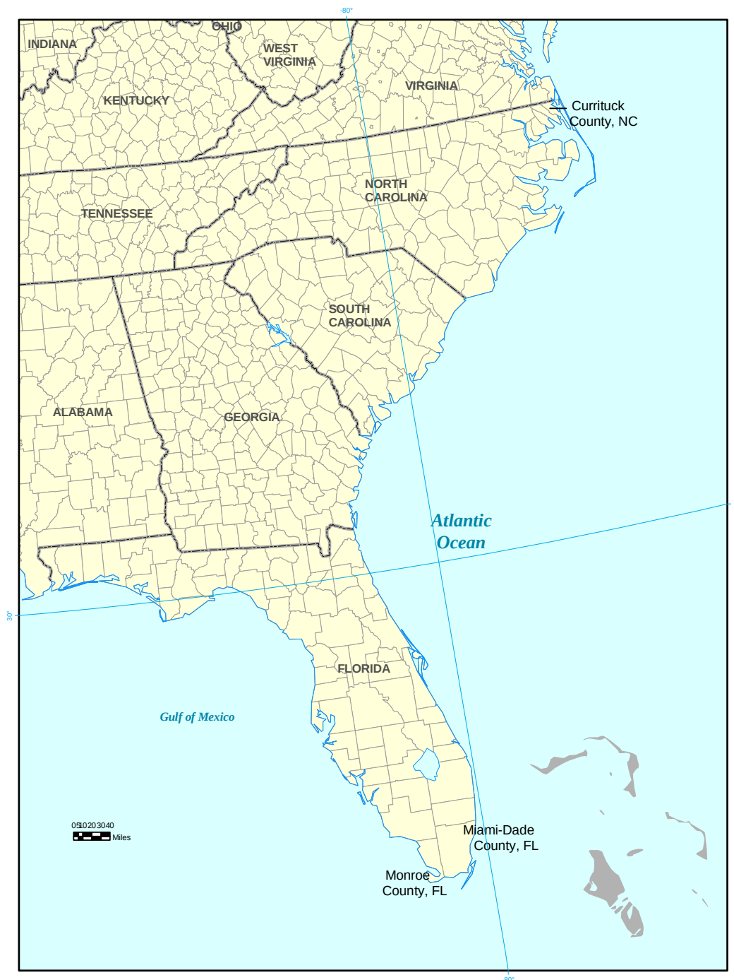
Figure 5.9. Counties sampled by the MRFSS, as used to compute the index of abundance, included those along the coast from Currituck County, NC through Miami-Dade County, FL.
