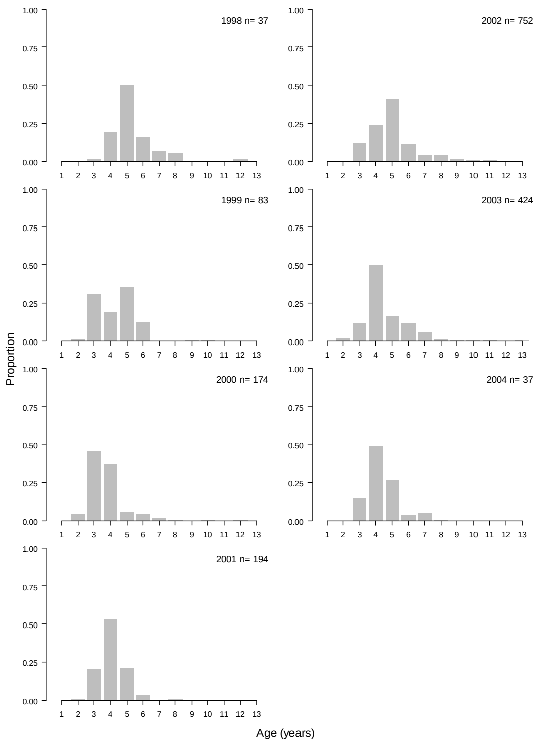
Figure 3.11. Age composition of greater amberjack for commercial handline from TIP, 1998-2004. Weighting based on corresponding length composition available for 1998-2004. Sample size and year shown on each subplot.
