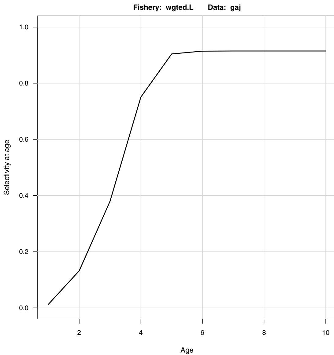
Figure 3.34. Greater amberjack- Base run: Estimated selectivity for landed fish used in MSY calculations computed from the 3-year geometric mean weighted fishing mortality rates ( F ) for all fishery gear types.
