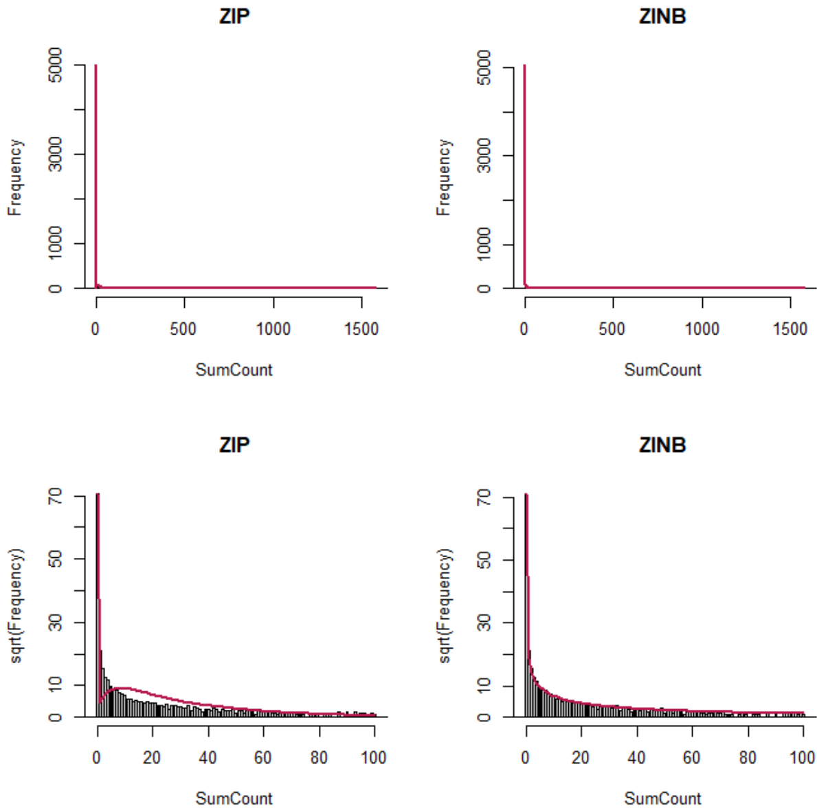
Figure 9: Model formulation comparison, with ZIP (left) and ZINB (right) fitted values plotted against the original data distribution. The lower panels are square root transformed and truncated at 100 fish for inspection of goodness of fit over the range of values for the bulk of the data.
