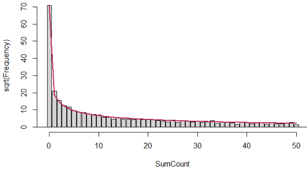
Figure 10: Model diagnostic plots of fitted model values (red line) against the original data distribution. Limited x-axis distribution view (lower).
