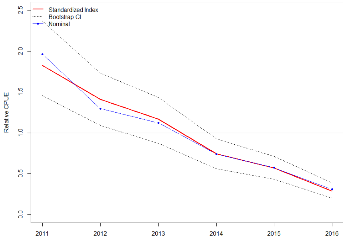
Figure 13: Relative standardized index (solid line) with 2.5% and 97.5% confidence intervals (dashed lines) and the relative nominal index (blue) for black sea bass in the SERFS video survey.
