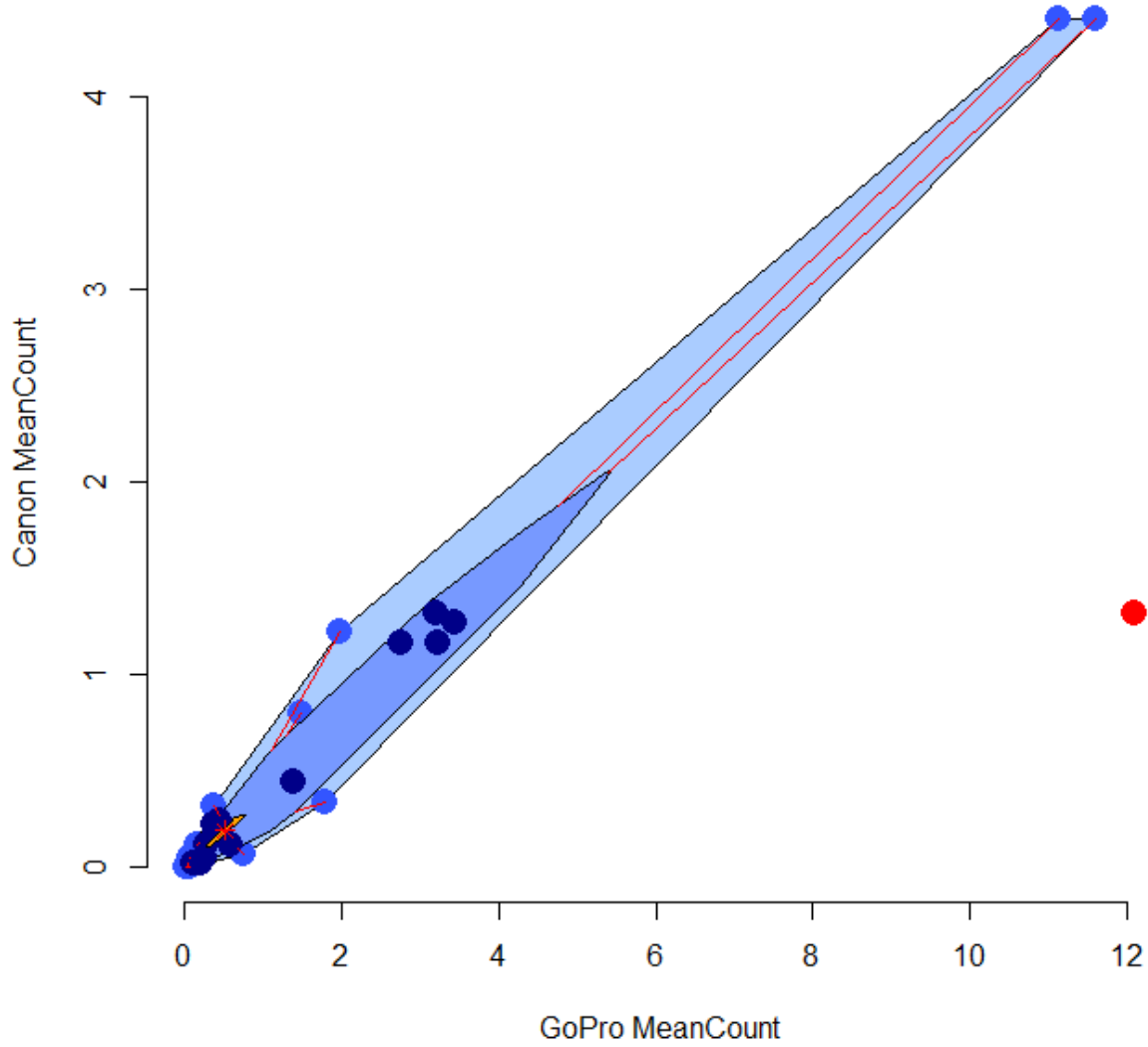
Figure 12: Bagplot of paired video counts from Canon and GoPro cameras. This method of visualizing outliers indicated the same pair of data as an outlier.
