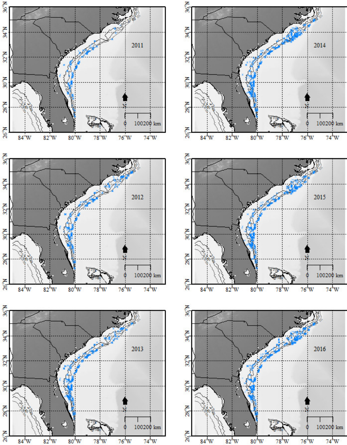
Figure 2: Annual spatial distribution of underwater video samples collected by SERFS in 2011 – 2016 where no black sea bass were seen on video. Bottom contours are drawn at the breaks for the depth factor (27, 35, and 50 meters).
