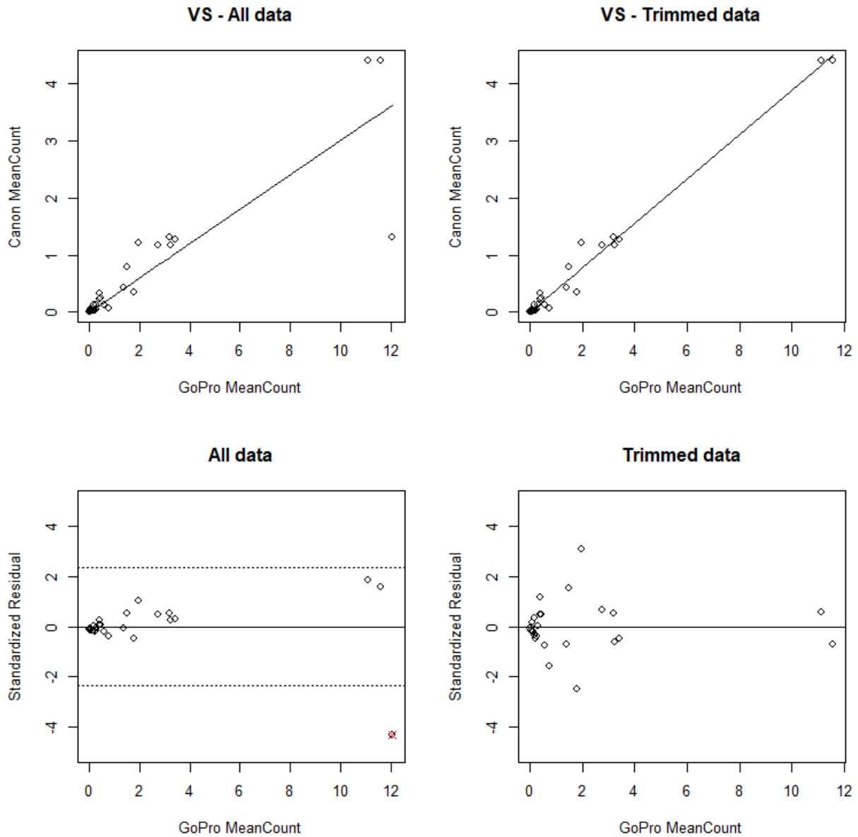
Figure 11: Linear regressions (intercept=0,top panels) and standardized residuals (bottom panels) using all data of the calibration study (left panels) and using trimmed data (right panels). Data points outside the Z-score associated with 99 th percentile of the standardized residuals (dotted lines -bottom, left panel) were removed.
