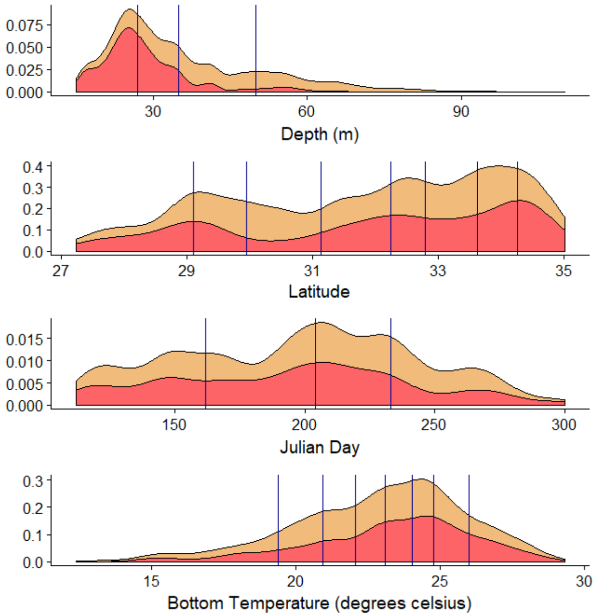
Figure 7: Sample distribution of data collected as continuous variables for positive (red) and zero (orange) counts. Vertical lines represent break points for factor definitions.
