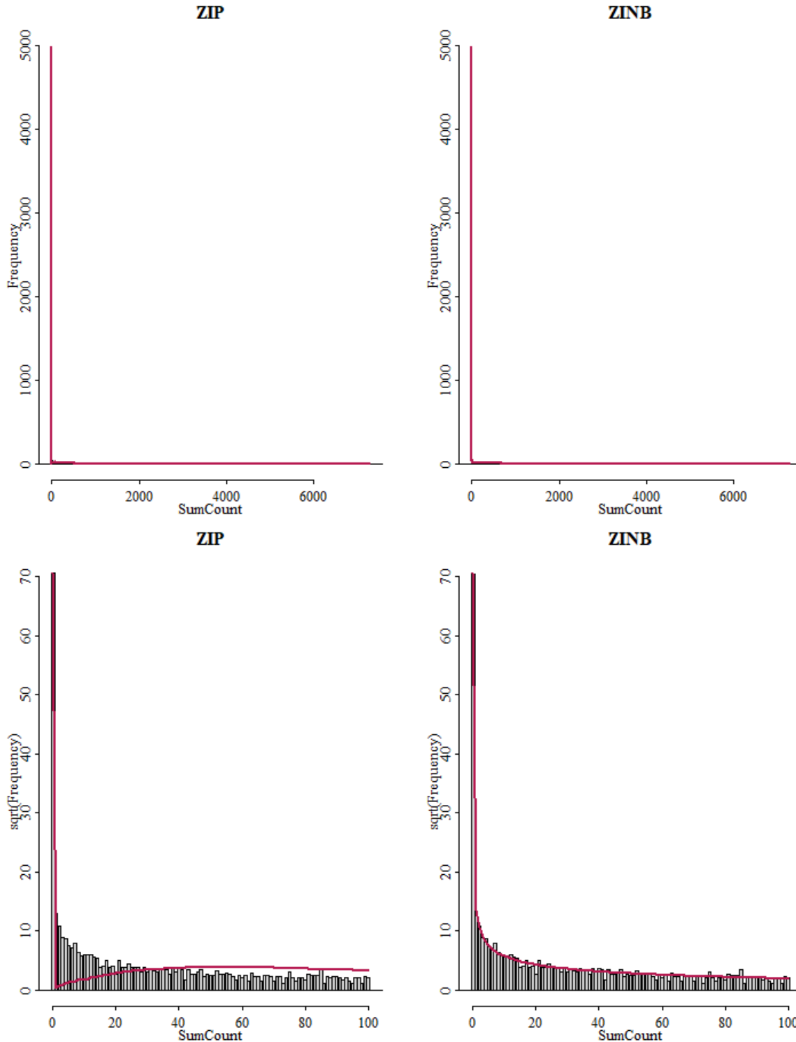
Figure 10: Model formulation comparison, with ZIP (left) and ZINB (right). The red line is the sum of the modeled probability at each SumCount across all observations. The upper panel retains the full range of SumCount values and Frequency in numbers. The lower panel are rootograms showing the square root of the frequency and SumCount is limited to a range of 0 – 100.
