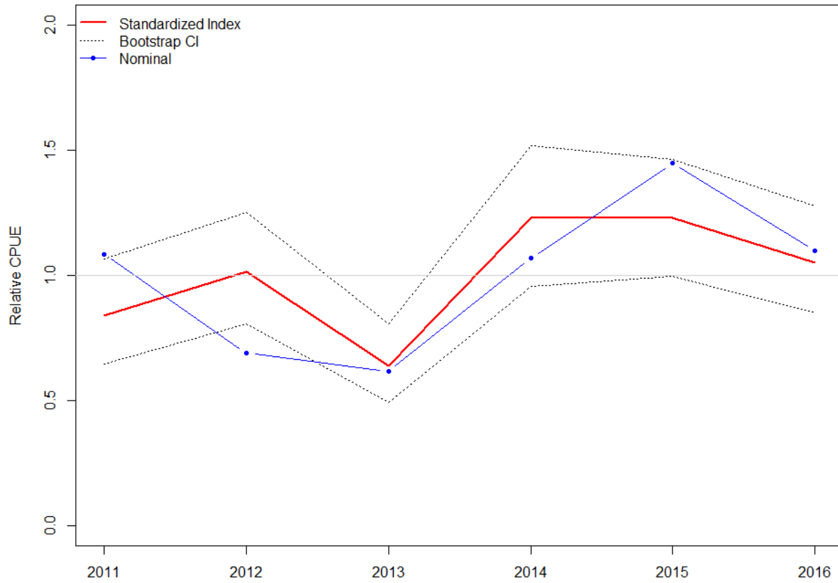
Figure 13: Relative standardized index (solid line) with 2.5% and 97.5% confidence intervals (dashed lines) and the relative nominal index (blue) for vermilion snapper in the SERFS video survey.
