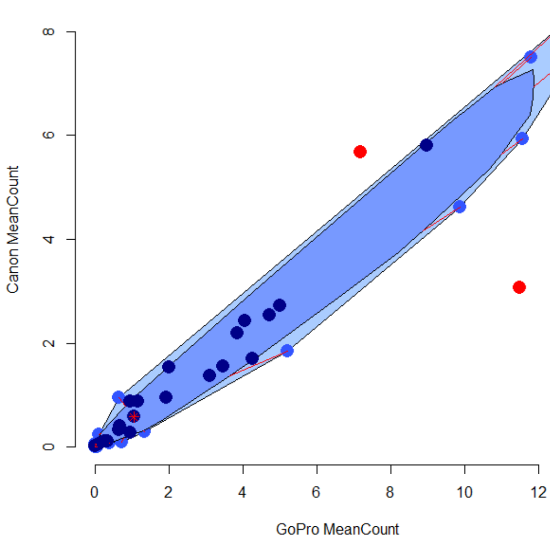
Figure 12: Bagplot of paired video counts from Canon and GoPro cameras. This method of visualizing outliers indicated the same pair of data as an outlier.
