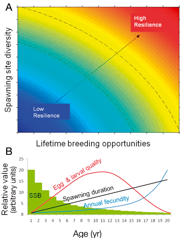
Fig. 1. (A) Conceptual model of reproductive resilience based on spatio-temporal diversity. Dashed curves show how a given resilience level can be met through tradeoffs between spatial and temporal diversity. (B) Potential relationships with age of reproductive traits impacting reproductive success: spawning stock biomass (SSB; a proxy for abundance), annual fecundity (blue), spawning duration as a proxy for the distribution of spawning events within a spawning season (black), and the maternal effects on egg and larval quality (red)
