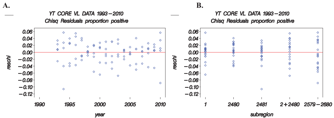
Figure 12. Diagnostic plots for the binomial component of the core area yellowtail snapper commercial vertical line gear core area model: A. the Chi-Square residuals by year and B. the Chi-Square residuals by subregion.
