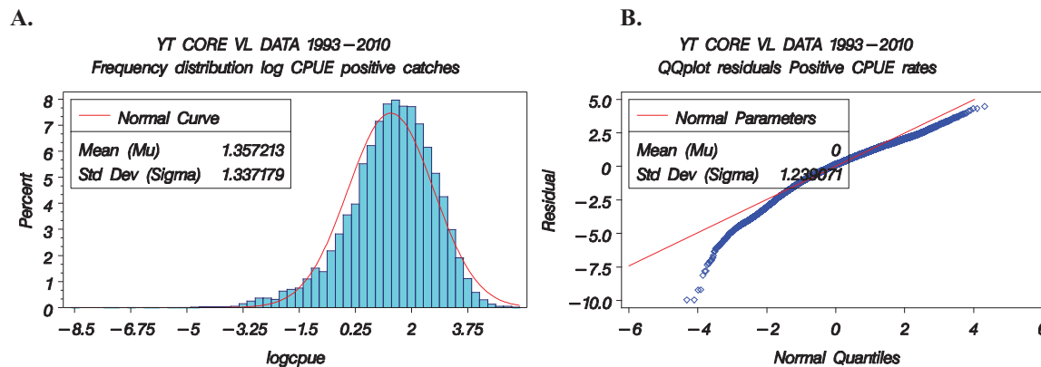
Figure 13. Diagnostic plots for the lognormal component of the core area yellowtail snapper commercial vertical line gear model: A. the frequency distribution of log(CPUE) on positive trips, B. the cumulative normalized residuals (QQ-Plot) from the lognormal model. The red line is the expected normal distribution.
