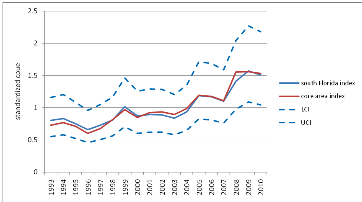
Figure 6. Comparison of the south Florida index with the core area index. Confidence intervals of the south Florida index are also provided.
