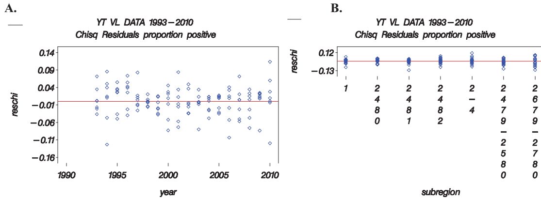
Figure 8. Diagnostic plots for the binomial component of the yellowtail snapper commercial vertical line gear south Florida model: A. the Chi-Square residuals by year and B. the Chi-Square residuals by subregion.
