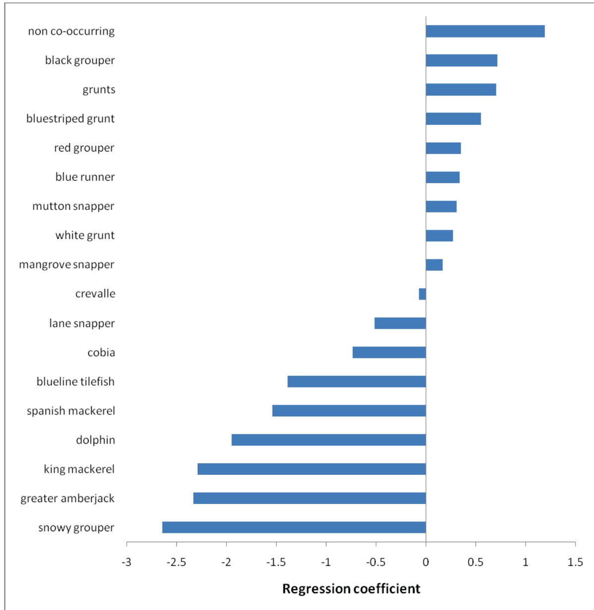
Figure 3. Regression coefficients from the core area Stephens & MacCall analyses. Positive coefficients signify species that had positive associations with the target species. The magnitude of the coefficients indicates the predictive impact of each species. The value for “non co-occurring” is the regression intercept and denotes the probability a trip was fishing in the target species’ habitat, but did not report any of the listed species. Species included were reported on at least one percent of vertical line trips in the South Atlantic.
