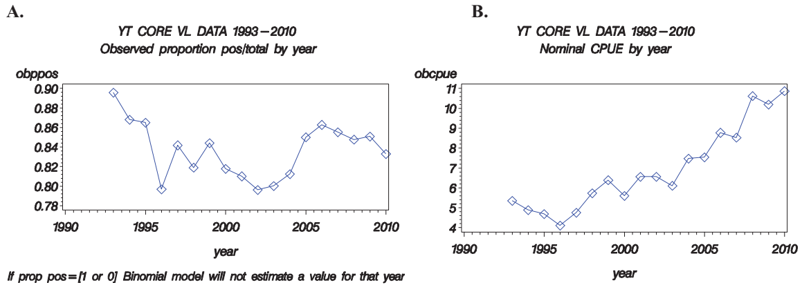
Figure 11. Core area yellowtail snapper commercial vertical line gear data set annual trends in A. the proportion of positive trips and B. nominal CPUE.
