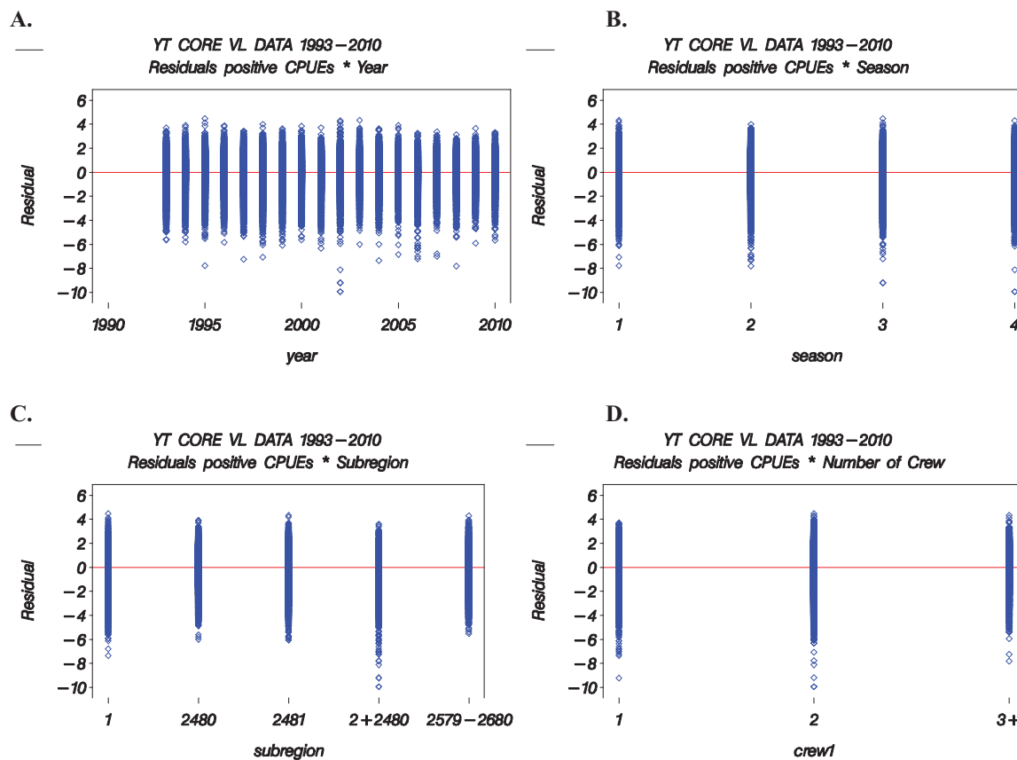
Figure 14. Diagnostic plots for the lognormal component of the core area yellowtail snapper commercial vertical line gear model: A. the Chi-Square residuals by year; B. the Chi-Square residuals by season; C. the Chi-Square residuals by subregion; D. the Chi-Square residuals by number of crew; and E. the Chi-Square residuals by days at sea.
