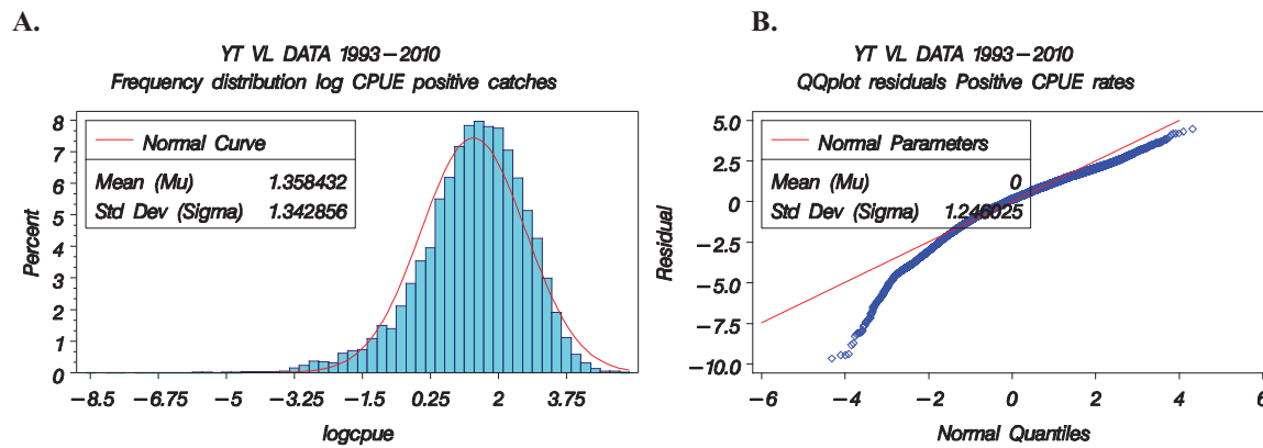
Figure 9. Diagnostic plots for the lognormal component of the south Florida yellowtail snapper commercial vertical line gear model: A. the frequency distribution of log(CPUE) on positive trips, B. the cumulative normalized residuals (QQ-Plot) from the lognormal model. The red line is the expected normal distribution.
