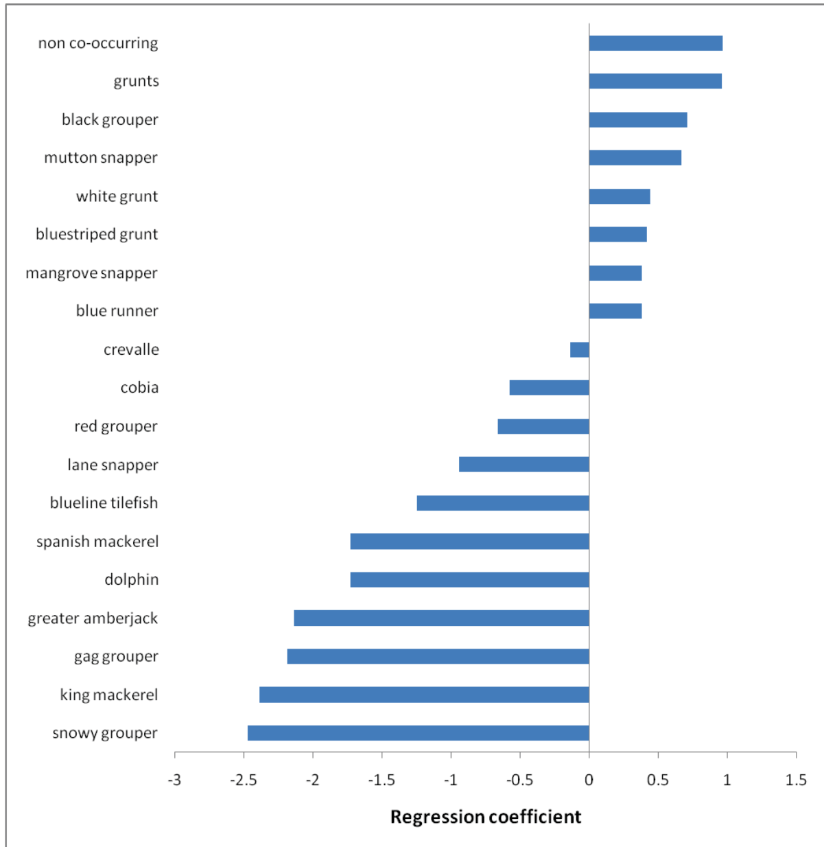
Figure 2. Regression coefficients from the south Florida Stephens & MacCall analyses. Positive coefficients signify species that had positive associations with the target species. The magnitude of the coefficients indicates the predictive impact of each species. The value for “non co-occurring” is the regression intercept and denotes the probability a trip was fishing in the target species’ habitat, but did not report any of the listed species. Species included were reported on at least one percent of vertical line trips in the South Atlantic.
