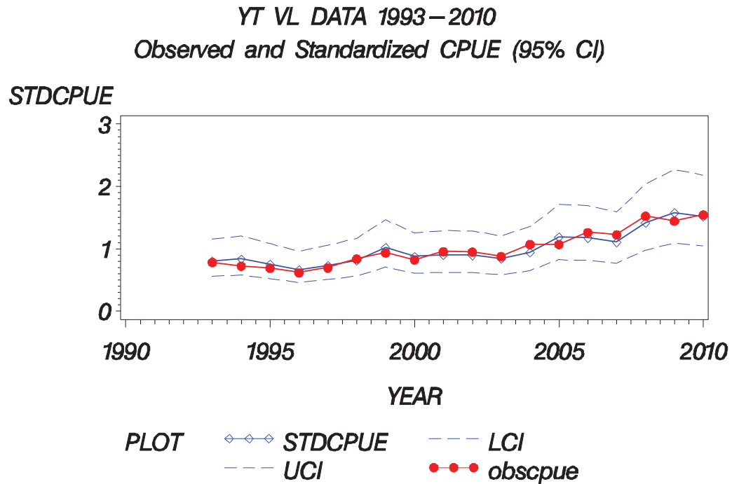
Figure 5. Yellowtail snapper core area nominal CPUE (solid circles), standardized CPUE (open diamonds) and upper and lower 95% confidence limits of the standardized CPUE estimates (dashed lines) for commercial vessels fishing vertical line gear.
