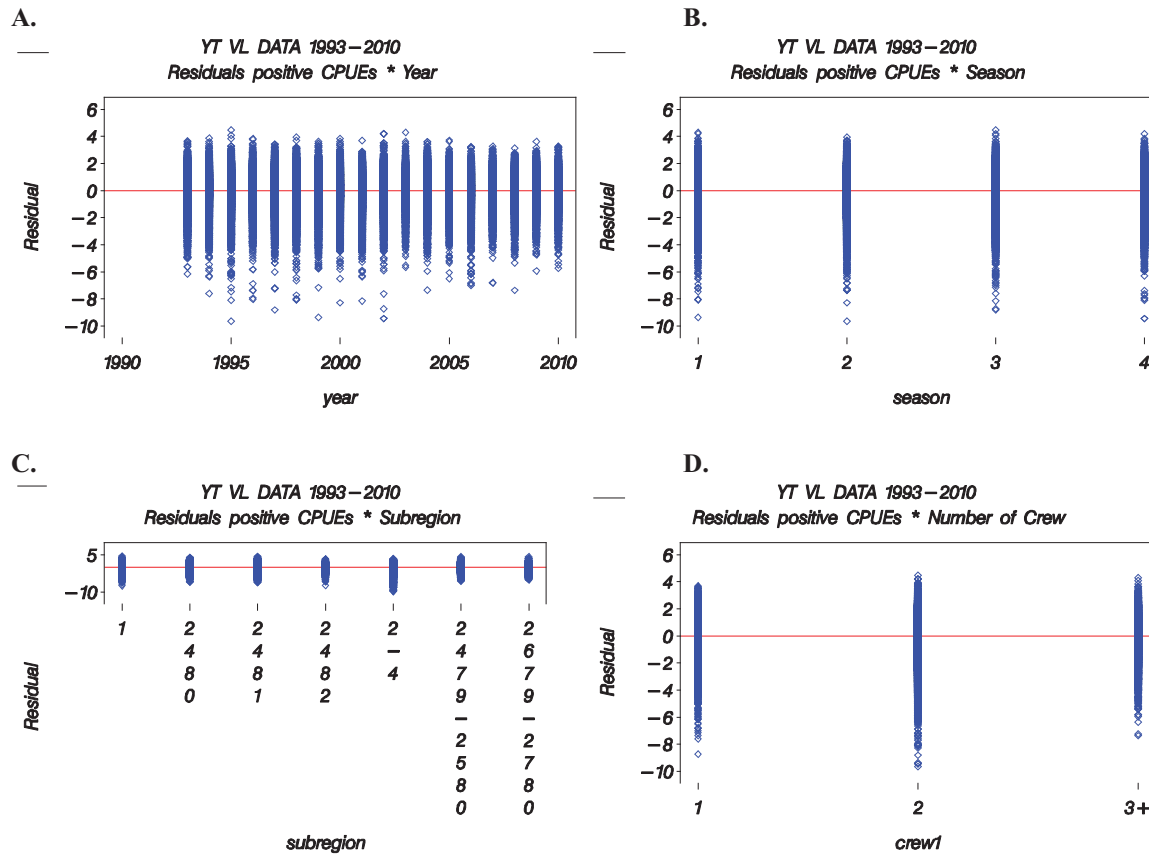
Figure 10. Diagnostic plots for the lognormal component of the south Florida yellowtail snapper commercial vertical line gear model: A. the Chi-Square residuals by year; B. the Chi-Square residuals by season; C. the Chi-Square residuals by subregion; and D. the Chi-Square residuals by number of crew.
