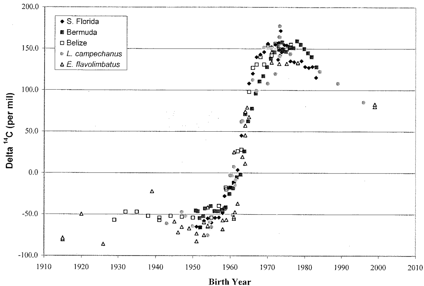
Figure 7. \Delta^{14}\text{C} values from the otolith cores ( n=39 ) of yellowedge grouper in relation to published \Delta^{14}\text{C} chronologies for Gulf of Mexico red snapper (Baker and Wilson, 2001), and corals from south Florida (Druffel, 1989), Bermuda (Druffel, 1989), and Belize (Druffel, 1980). Yellowedge grouper data points represent year of birth although core samples may contain up to three years of growth. Birth year was calculated from capture date and age estimated by counting otolith annuli.
