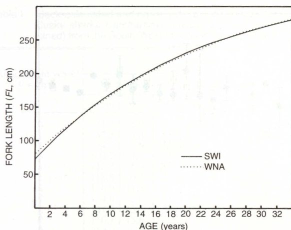
Fig. 5: Comparison of Von Bertalanffy growth curves derived from back-calculated vertebral data (sexes combined) for dusky sharks Carcharhinus obscurus from the South-West Indian Ocean (SWI) and the west-north Atlantic Ocean (WNA)
