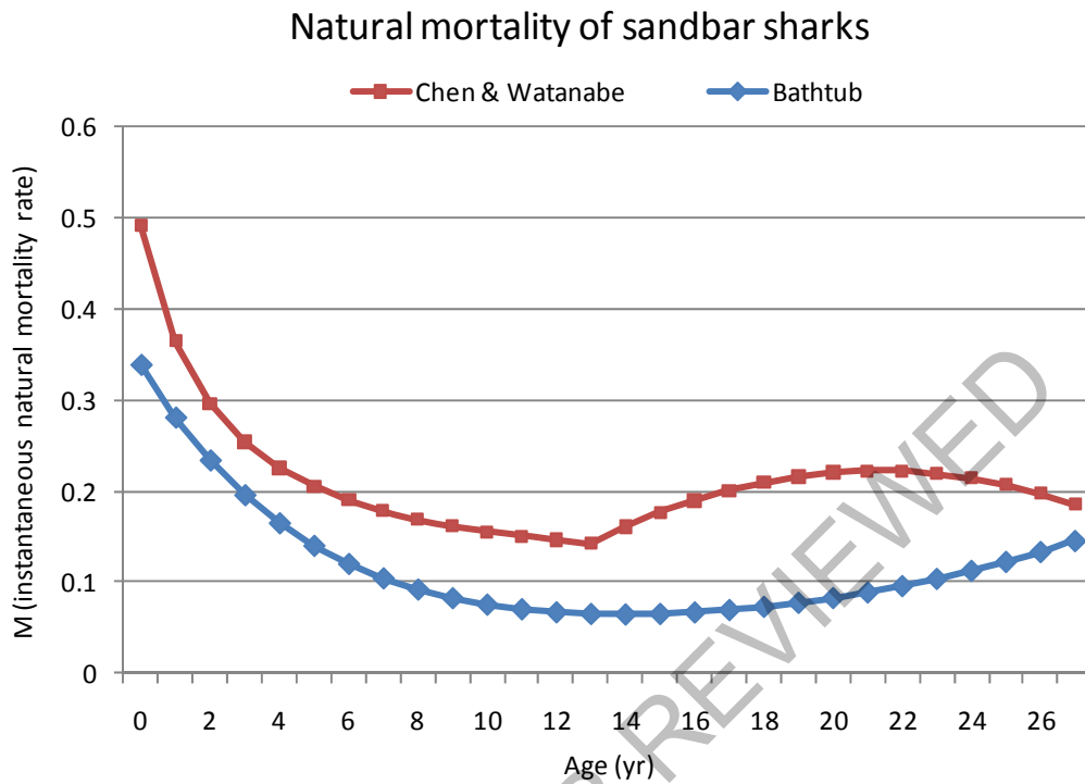
Figure 3.1. Natural mortality at age derived from the Chen and Watanabe (1989) and “bathtub” methods. The “bathtub” method was used to approximate the values of the Chen and Watanabe method while providing a better U shape.
