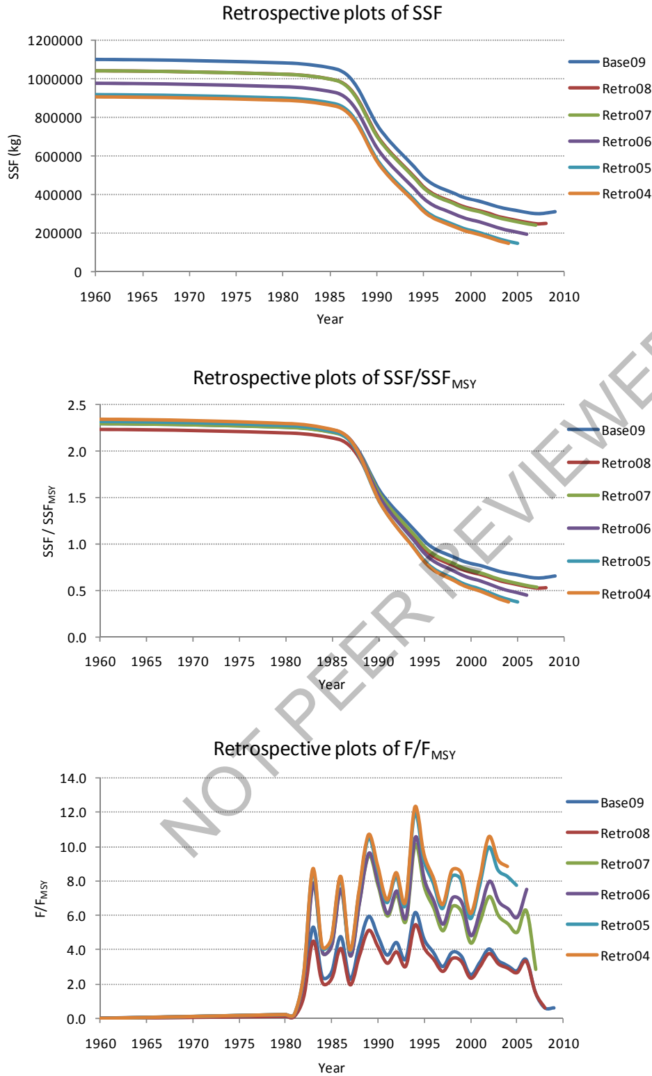
Figure 3.20. Retrospective analysis for sandbar shark with last five years of data sequentially removed from the model. Model quantities examined include spawning stock fecundity (top), relative spawning stock fecundity (middle), and relative fishing mortality rate (bottom).
