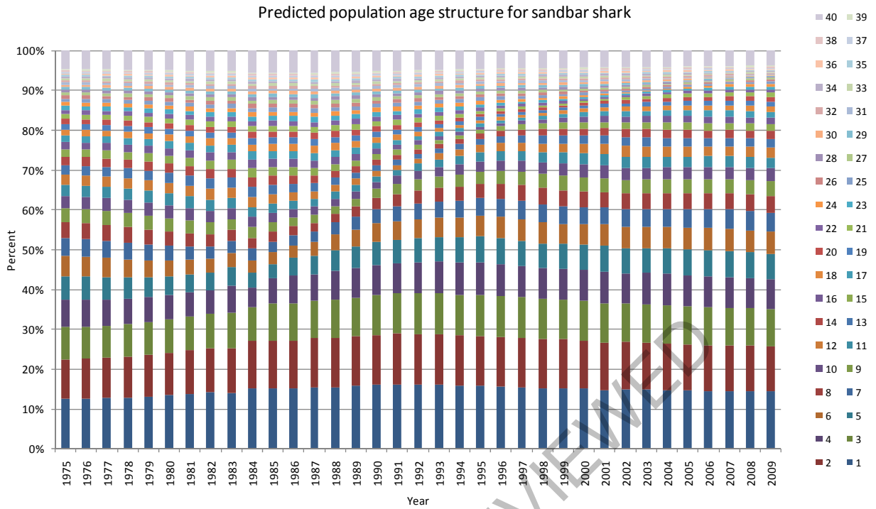
Figure 3.7. Predicted abundance at age for sandbar shark.
