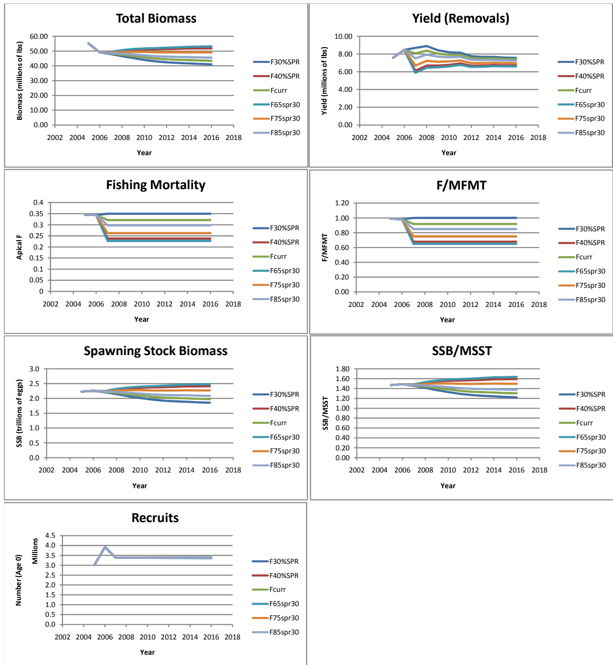
Figure 3.26. Projection results for the staus quo case, Atlantic.
