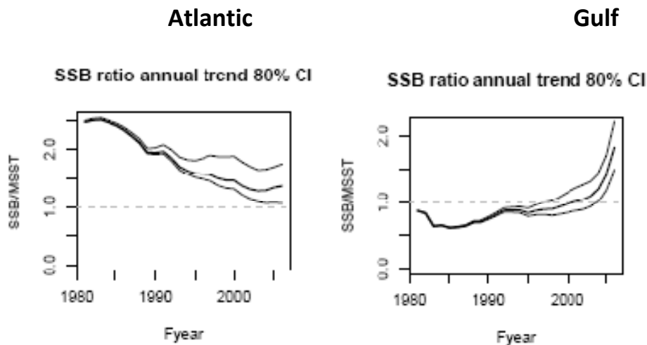
Figure 3.14. Annual trend in SSB/MSST for base models with upper and lower 80% confidence intervals.
