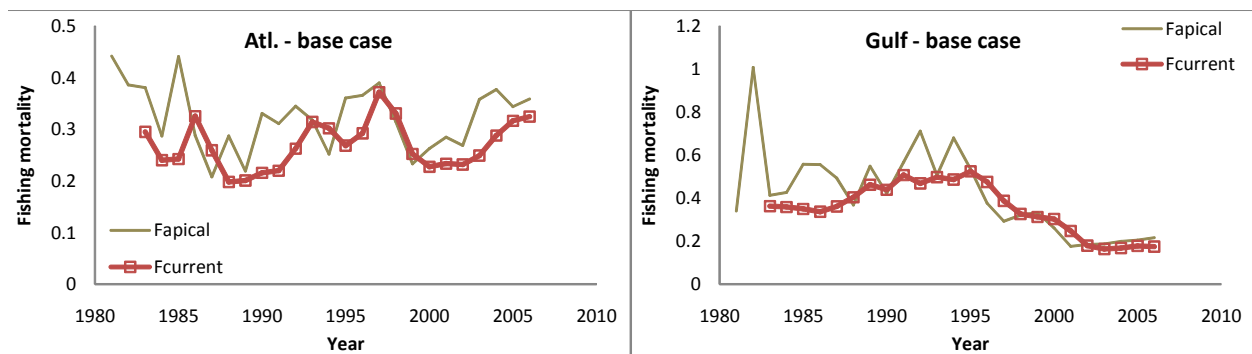
Figure 3.16. Annual trend in apical fishing mortality and current fishing mortality for base models. .
