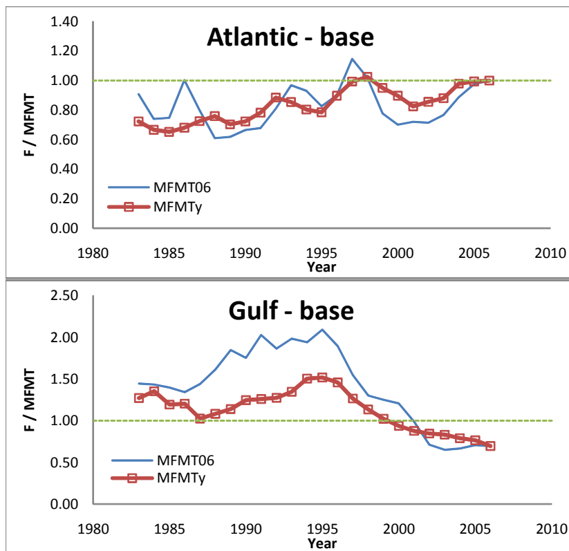
Figure 3.18. Annual trend in F/MFMT for base models using two different measures of MFMT. MFMT y corresponds to F 30% calculated with the selectivity vector corresponding to each year's current selectivity (based on the mean F values for years y-2, y-1 and y); MFMT 2006 is calculated with the 2006 current F selectivity vector (based on F for years 2004-2006). .
