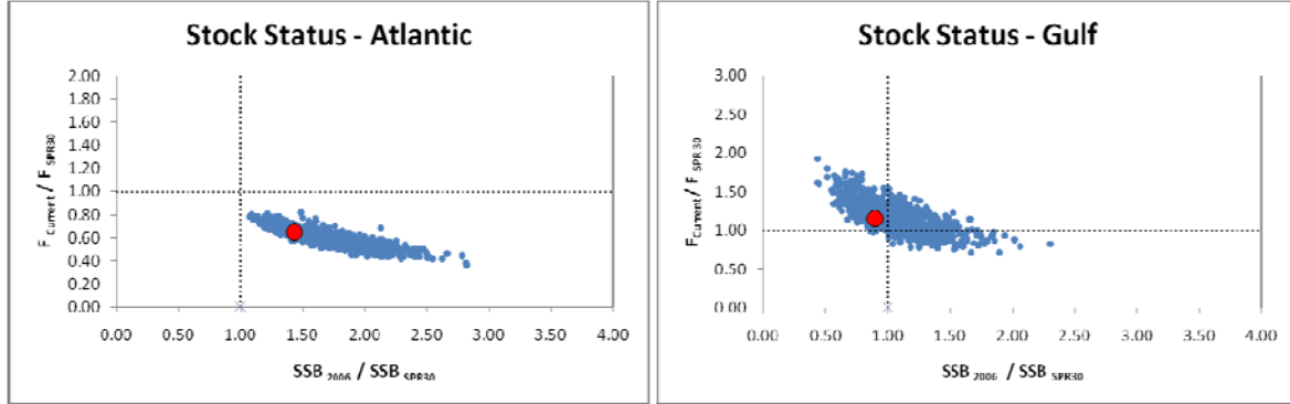
Figure 12. Model uncertainty concerning estimates of stock status for the Atlantic (a) and Gulf (b) migratory groups. Blue points are the results of 1000 non-parametric bootstraps runs. The deterministic run is indicated by the red circle. F_{\text{Current}} is the average F 2003-2005.
