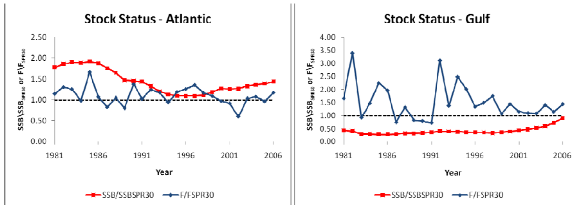
Figure 11. Spawning stock biomass and fishing mortality relative to SSB and F at SPR30 for the Atlantic (a) and Gulf (b) migratory groups.
