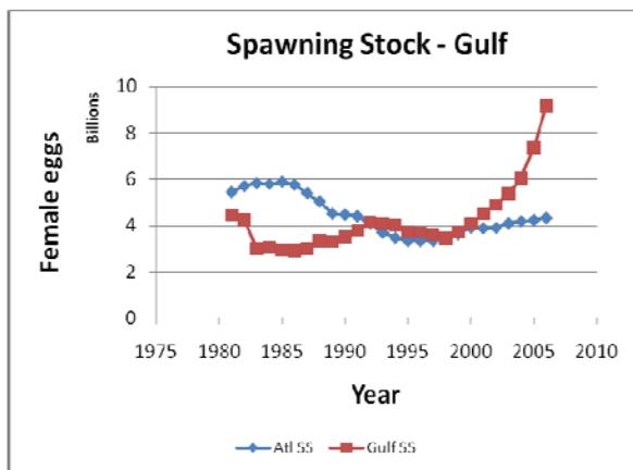
Figure 10. Annual trends in spawning stock biomass.
