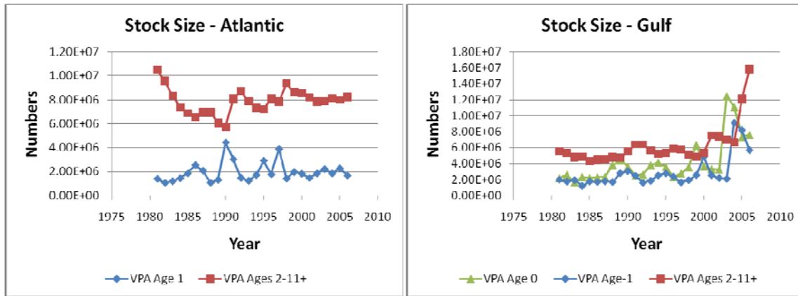
Figure 3. Number of king mackerel at various ages in the Atlantic (a) and Gulf (b).
