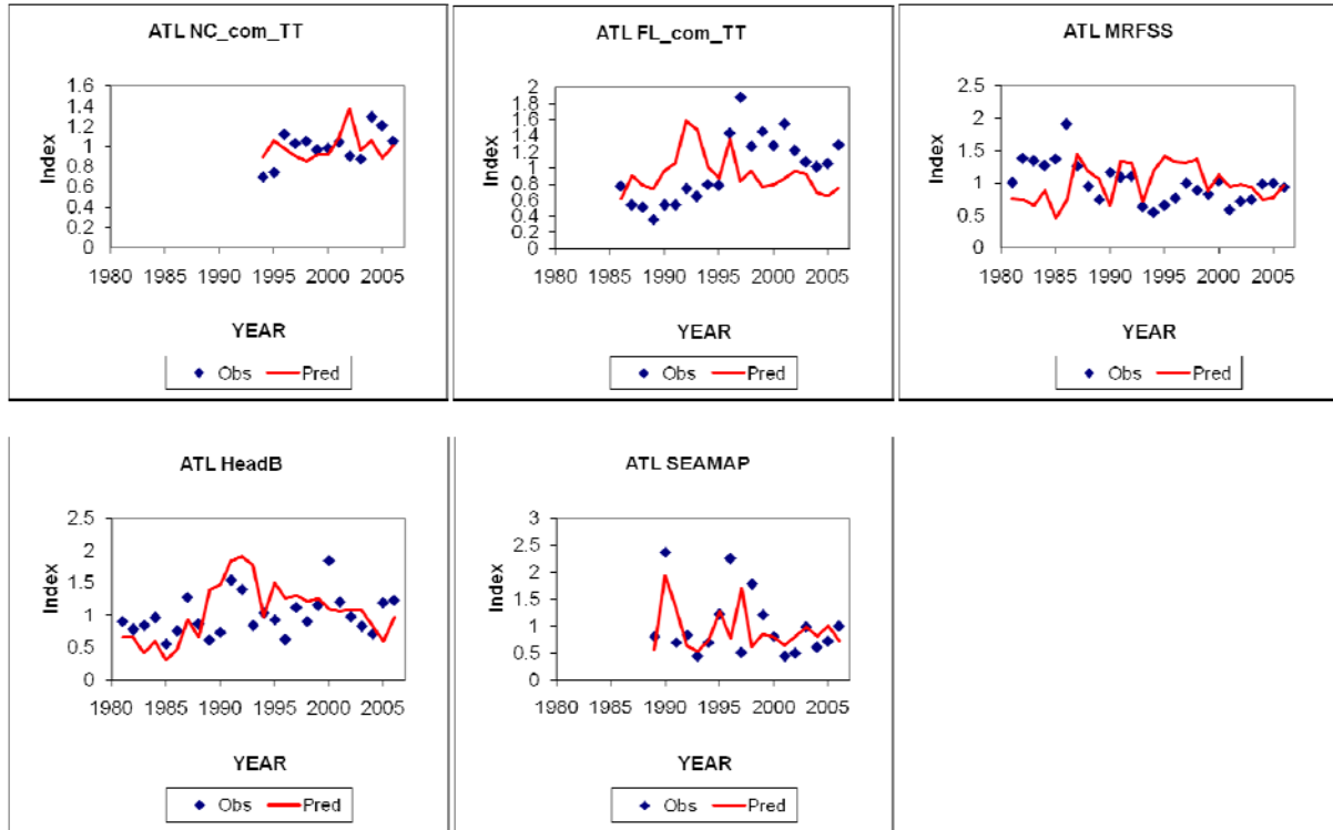
Figure 1. Fits to the indices for the Atlantic VPA-2BOX continuity run.
