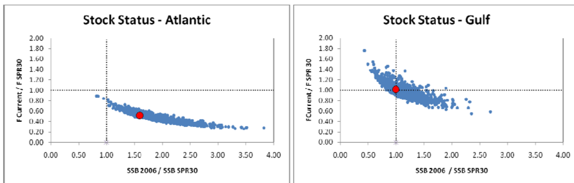
Figure 7. Model uncertainty concerning estimates of stock status for the Atlantic (a) and Gulf (b) migratory groups. Blue points are the results of 1000 non-parametric bootstraps runs. The deterministic run is indicated by the red circle. F_{\text{Current}} is the average F during 2003-2005.
