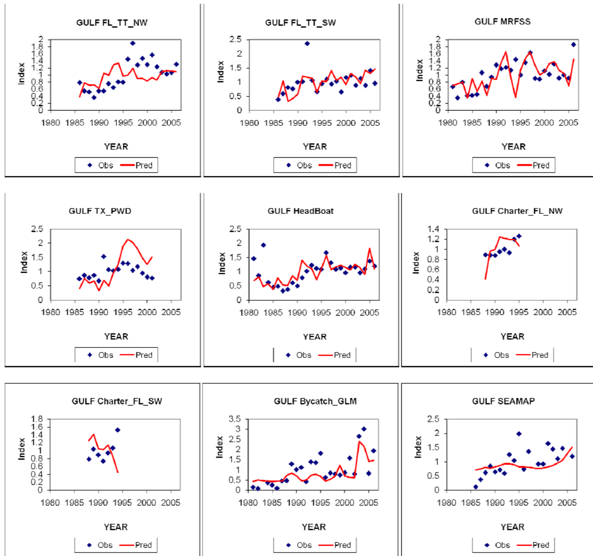
Figure 2 Fits to the indices for the Gulf VPA-2BOX continuity run.
