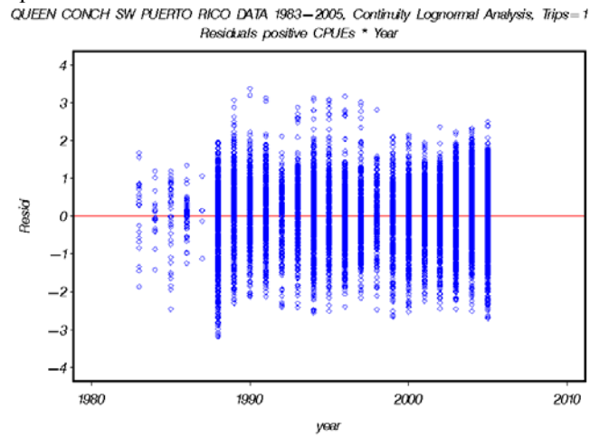
Figure A41. Residuals for the lognormal model on successful catch rates for southwest Puerto Rico lognormal analysis on trips=1.
