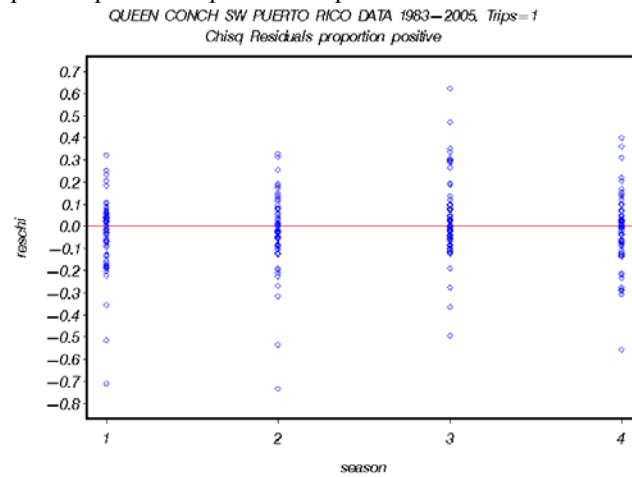
Figure A104. Residuals for the delta-lognormal model on successful catch rates for southwest Puerto Rico binomial analysis on proportion positive trips where trips=1.
