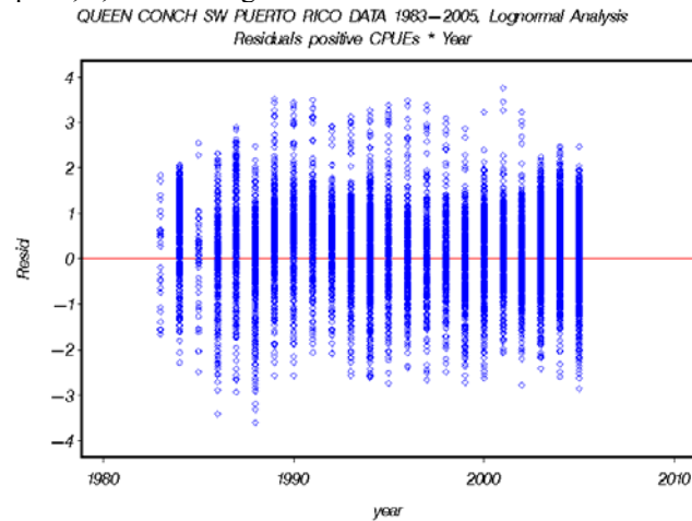
Figure A77. Residuals for the lognormal model on successful catch rates for southwest Puerto Rico lognormal analysis on trips=1, 0, and missing.
