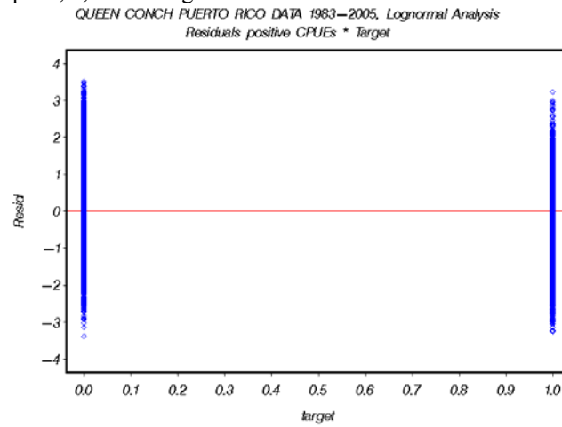
Figure A46. Residuals for the lognormal model on successful catch rates for Puerto Rico lognormal analysis on trips=1, 0, or missing.
