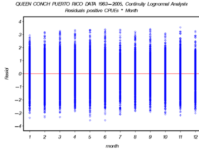
Figure A4. Residuals for the lognormal model on successful catch rates for Puerto Rico lognormal analysis on trips=1, 0, or missing.
