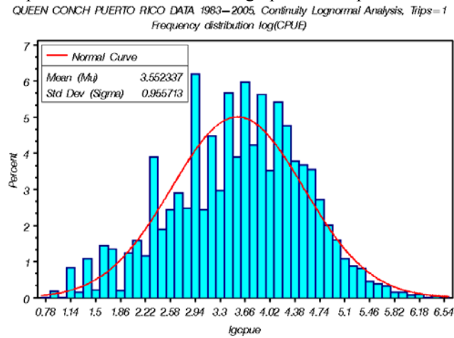
Figure A7. Error distribution \ln(\text{CPUE}) of the final lognormal 2002 model of Puerto Rico conch landings data, included data from trips=1. The solid line in each graph is the expected normal distribution.
