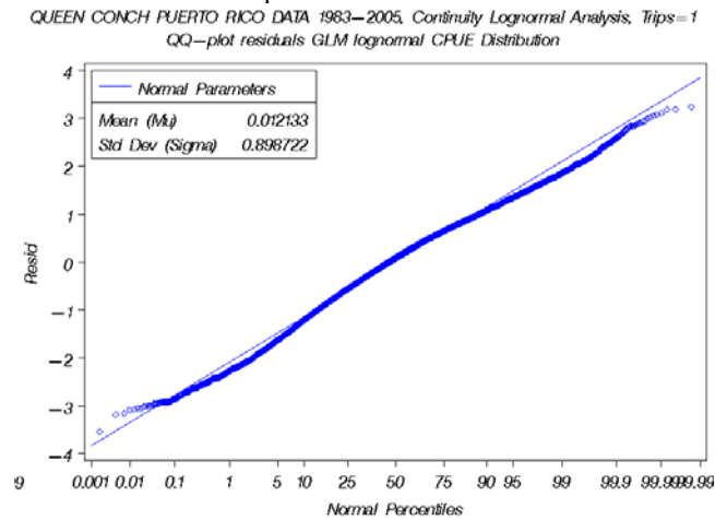
Figure A8. QQ plots of residuals of the final lognormal 2002 model of successful catch rates for vessels landing queen conch in Puerto Rico where trips=1.
