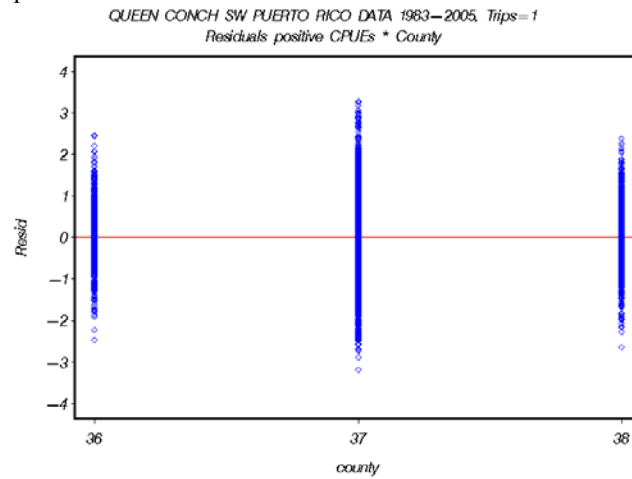
Figure A101. Residuals for the delta-lognormal model on successful catch rates for southwest Puerto Rico lognormal analysis on trips=1.
