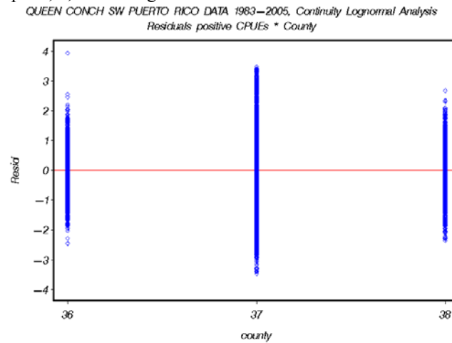
Figure A37. Residuals for the lognormal model on successful catch rates for southwest Puerto Rico lognormal analysis on trips=1, 0, or missing.
