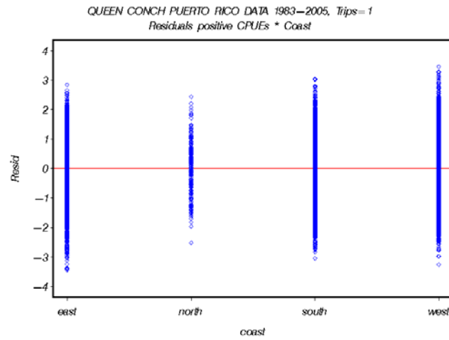
Figure A71. Residuals for the lognormal model on successful catch rates for Puerto Rico lognormal analysis on trips=1.
