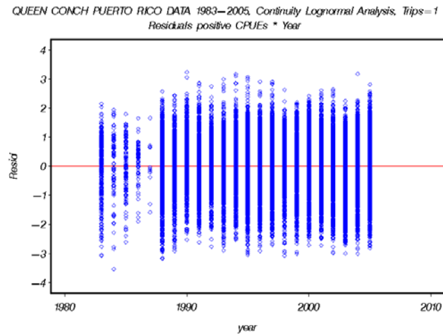
Figure A9. Residuals for the lognormal model on successful catch rates for Puerto Rico lognormal analysis on trips=1.
