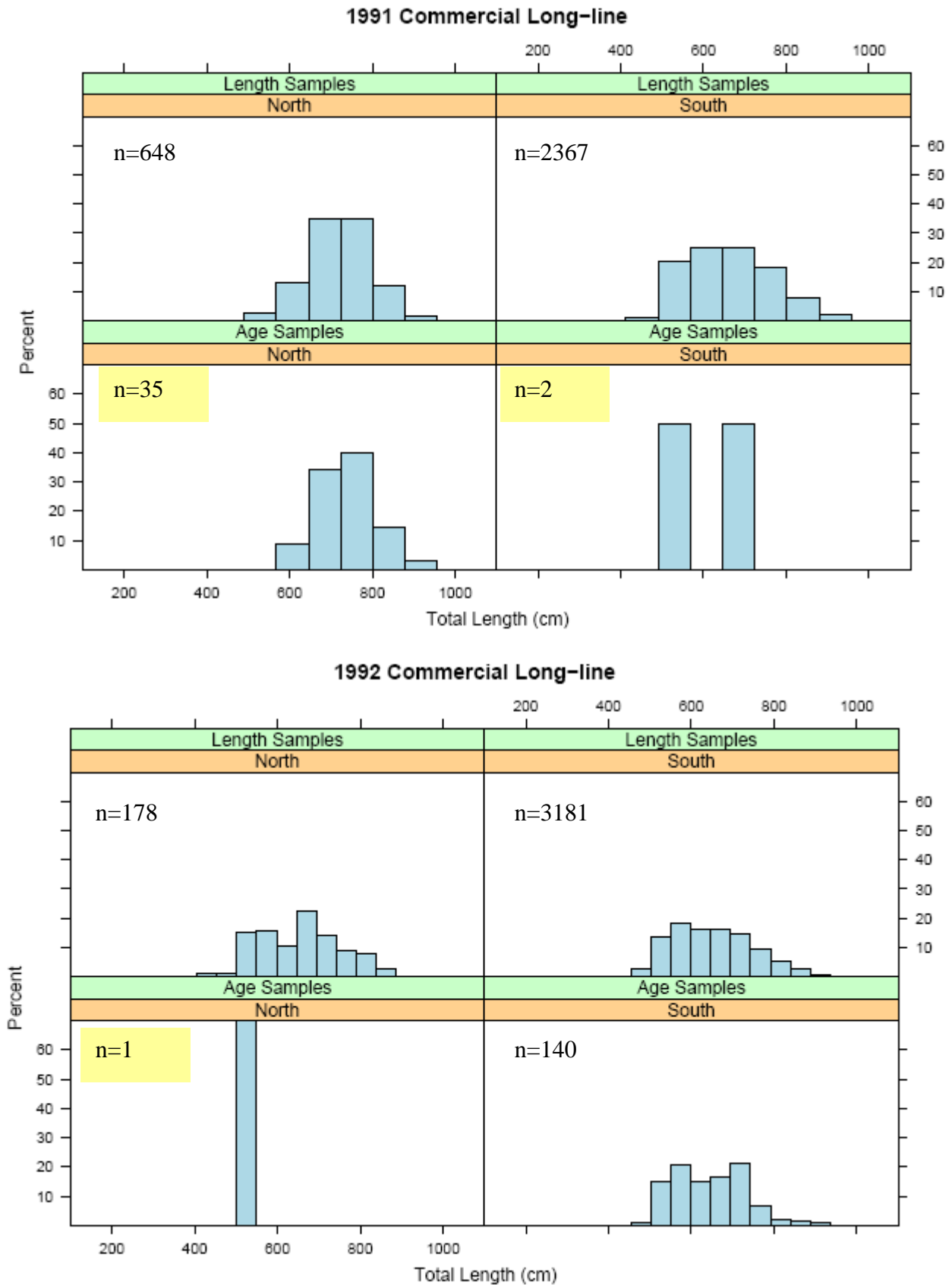
Figure 5. Commercial long-line length frequency distributions by region and by sampling type: length or age based.
