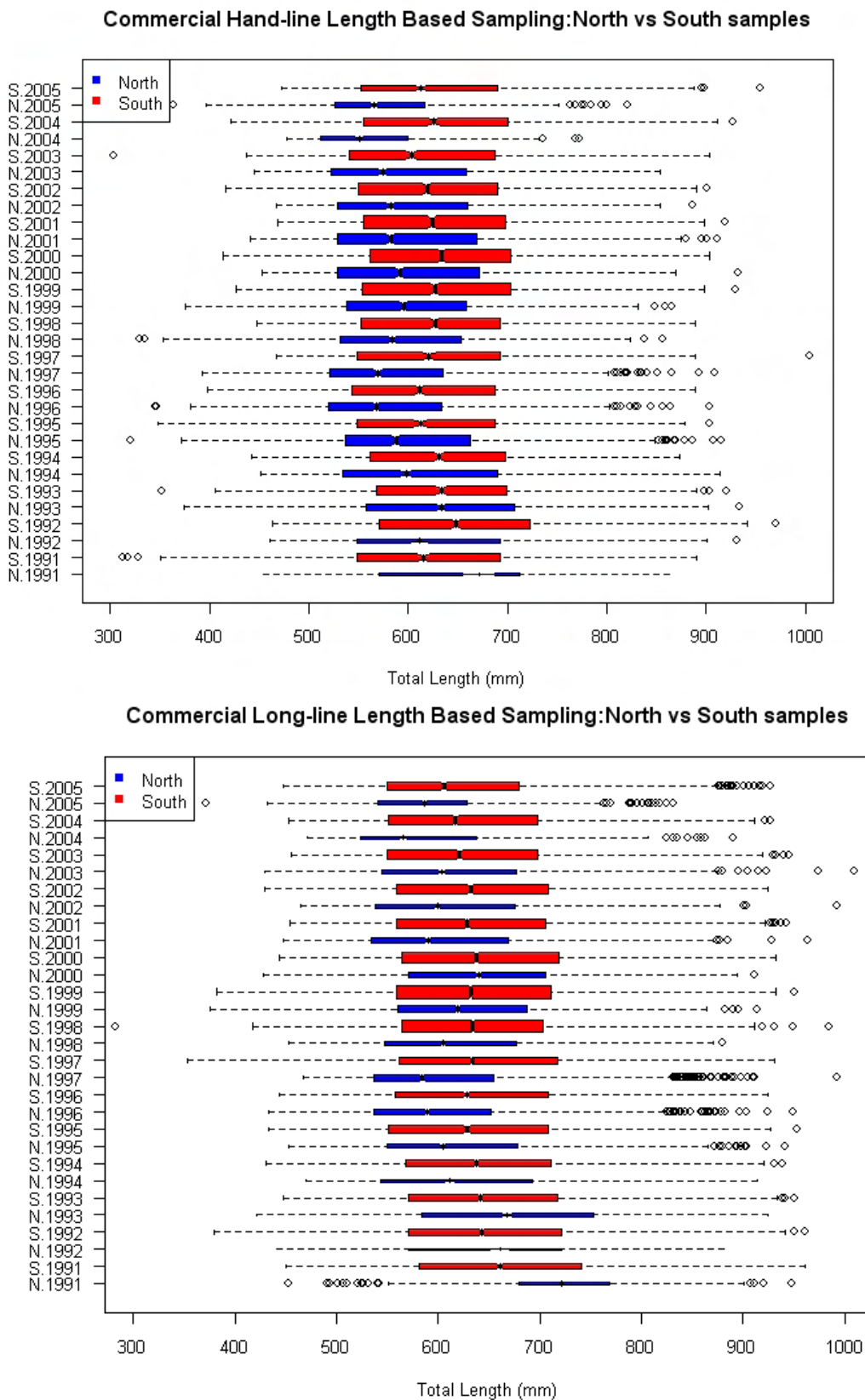
Figure 1. Box plots of the gear specific commercial length based samples by region, including the median, upper and lower quartiles (boxes: drawn in proportion to the square root of the sample size), upper and lower range (dashed line), and outliers (open circles).
