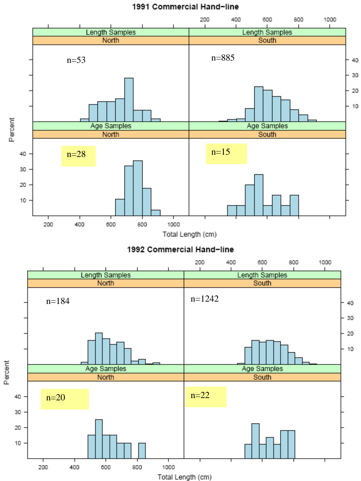
Figure 4. Commercial hand-line length frequency distributions by region and by sampling type: length or age based.
