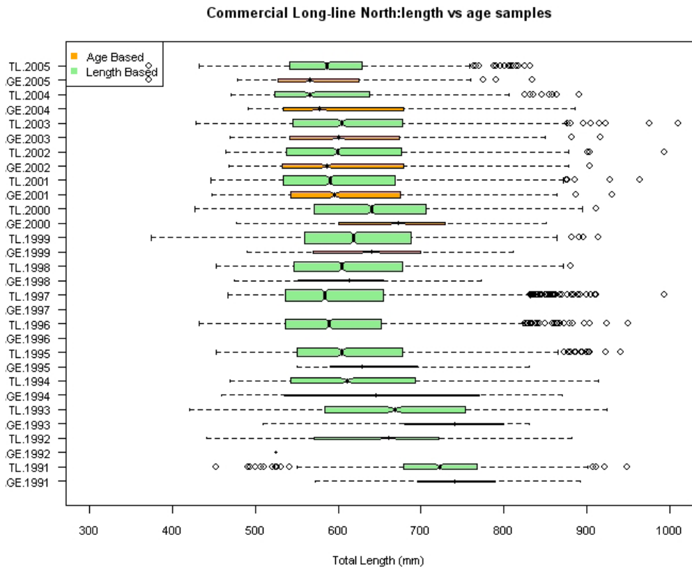
Figure 3. Box plots of region specific commercial long-line length and age based samples, including the median, upper and lower quartiles (boxes: drawn in proportion to the square root of the sample size), upper and lower range (dashed line), and outliers (open circles).
