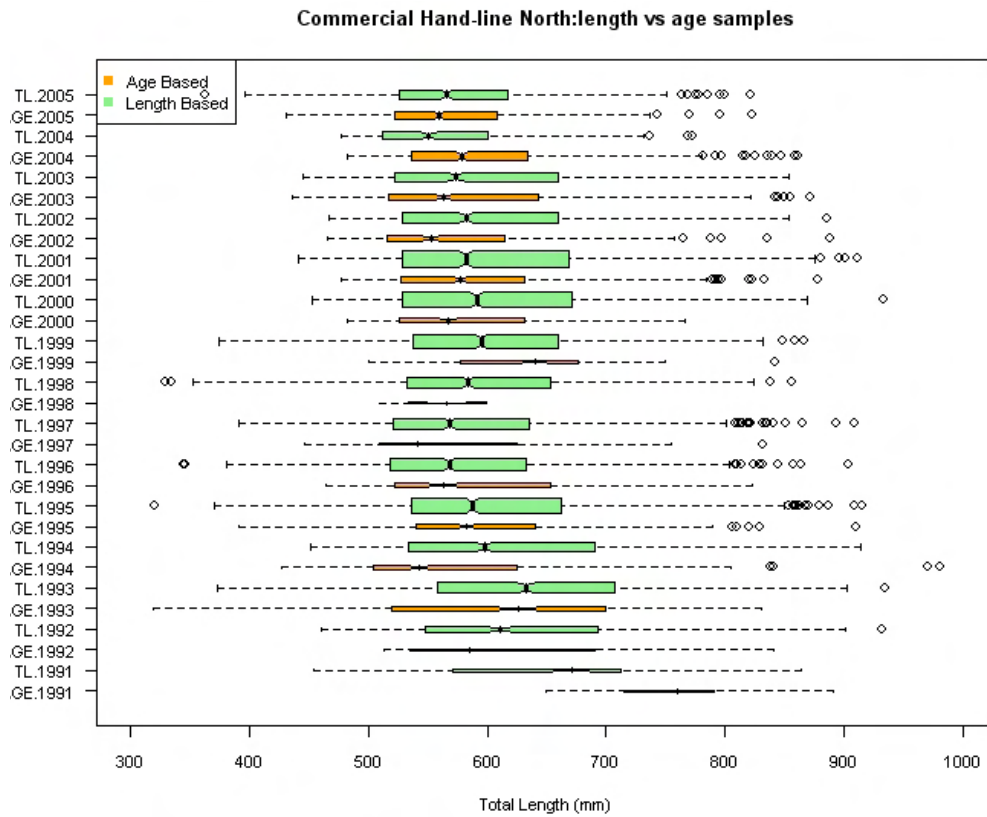
Figure 2. Box plots of region specific commercial hand-line length and age based samples, including the median, upper and lower quartiles (boxes: drawn in proportion to the square root of the sample size), upper and lower range (dashed line), and outliers (open circles).
