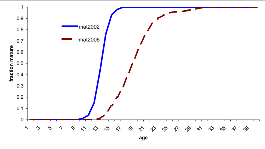
Figure 4. Maturity ogives for the continuity model (mat2002) and the maturity ogive accepted by the data workshop for the 2006 base model (mat2006).
