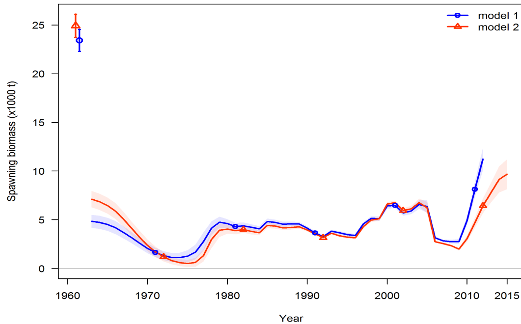
Figure 4. Spawning stock biomass estimates from SEDAR 33 (model 1) and the update assessment (model 2)
