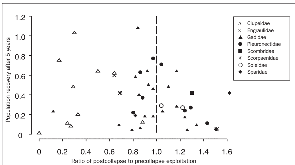
Figure 3. Recovery of marine fish populations 5 years after the proportionately largest 15-year decline by each population (as a ratio of postcollapse to precollapse exploitation rate). Populations that experienced reductions in fishing mortality after the collapse are shown to the left of the dashed line; those in which exploitation increased are to the right.
