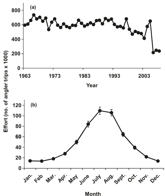
Fig. 2. Annual (a) and mean monthly (b) trends in fishing effort by the commercial passenger fishing vessel (CPFV) fleet in southern California from 1963 to 2008. Vertical bars indicate standard error.
