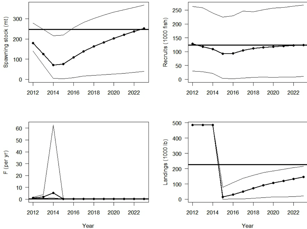
Figure 2. Scenario 1: F=F_{\text{rebuild}} with 50% probability. For this assessment, discards were combined with landings so the ABC reflects both landings and dead discards (landings and dead discards are separated in the associated Tables). Annual ABCs are a single quantity while other values presented are medians. Error bars represent the 5 th and 95 th percentiles of the 10,000 projection runs.
