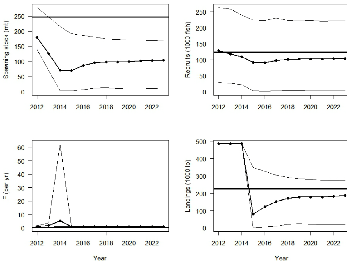
Figure 4. Scenario 1: F = F_{\text{current}} (geometric mean F from 2009, 2010, and 2012). For this assessment, discards were combined with landings so the ABC reflects both landings and dead discards (landings and dead discards are separated in the associated Tables). Annual ABCs are a single quantity while other values presented are medians. Error bars represent the 5 th and 95 th percentiles of the 10,000 projection runs.
