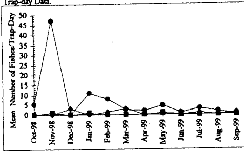
Figure 13a. Monthly Mean Number of Haemulon flavolineatum Caught Per Trap-Day for Northeast St. Croix Embayments Based on Pooled Trap-day Data.
