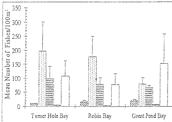
Figure 5a. Mean Fish Densities For Southeast St. Croix Embayment By Habitat Based on Pooled Monthly and Transect Site Data
