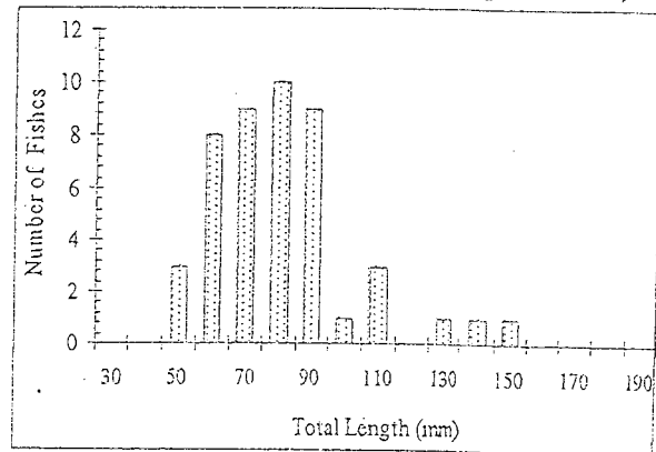
Figure 19h. Length Frequency Distribution of Trachinotus falcatus Caught by Seine Net-Hauls in Robin Bay Based on Pooled Monthly and Seine-Net Haul Data (subsample, N=46)
