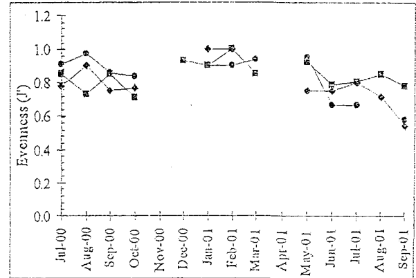
Figure 4b. Monthly Pielou Evenness Index ( J' ) For Each Southeast St. Croix Embayment based on Pooled Transect Site Data
