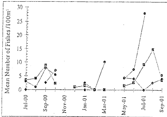
Figure 9a. Mean Monthly Sparisoma radians Densities for Southeast St. Croix Embayments Based on Pooled Transect Site and Size Group Data
