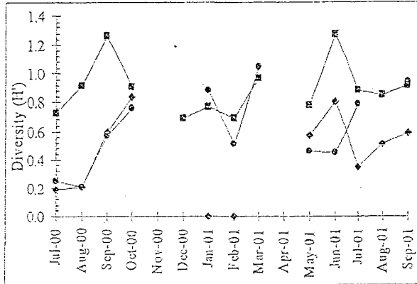
Figure 4a. Monthly Shannon Wiener Diversity Index ( H' ) For Each Southeast St. Croix Embayment based on Pooled Transect Site Data
