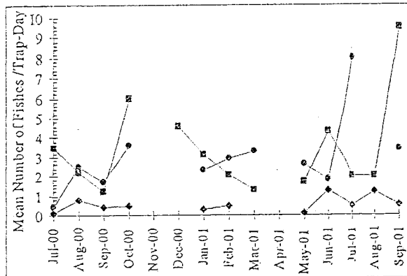
Figure 11a. Mean Number of Fish Caught Per Trap-Day in Southeastern St. Croix Embayments by Month (Pooled Trap-day Data)
