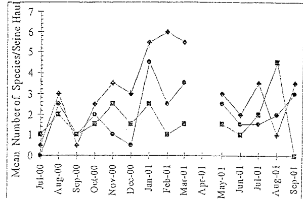
Figure 17b. Mean Monthly Number of Species Caught Per Seine-Haul for Southeast St. Croix Embayments Based on Pooled Seine-Haul Data.
