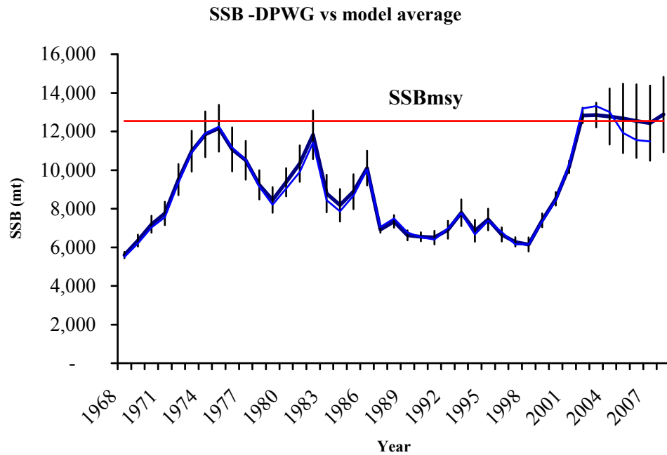
Figure 15. Spawning stock biomass predicted by SCALE model (thin line) for DPWG model and model average update (heavy line). 95% CI reflect variation among 10 models used in model average. SSB MSY value from DPWG results.
