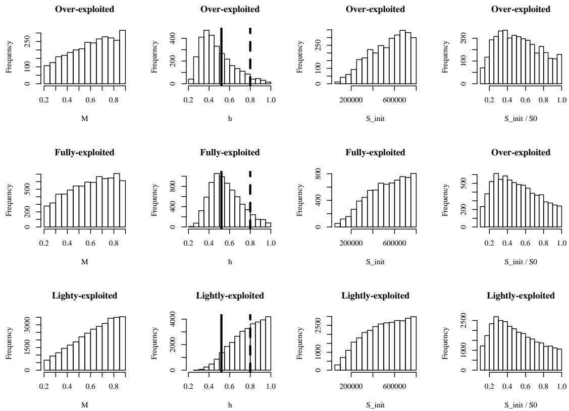
Figure 12. Kept values for M , steepness ( h ), initial spawning biomass ( S_{init} ) and the initial depletion ( S_{init} / S_0 ) for the simulation model using the truncated time series of catch data (1978-2014). The dashed and solid vertical lines represent the values of steepness from Myers et al. (1999) for Atlantic mackerel and all members of the family Scombridae , respectively.
