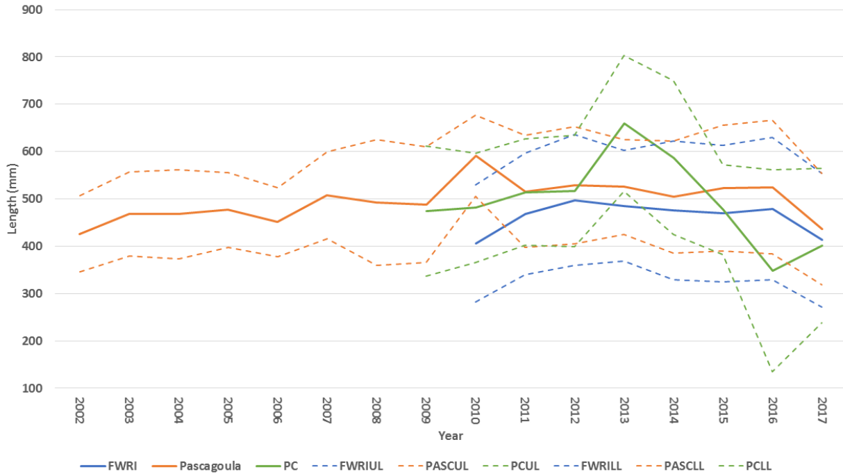
Figure 2.33. Comparison of mean length (solid lines) and standard error (dashed line) of Red Grouper from each video survey: FWRI (in blue), NMFS Mississippi Laboratories (orange), and NMFS Panama City Laboratory (green).
