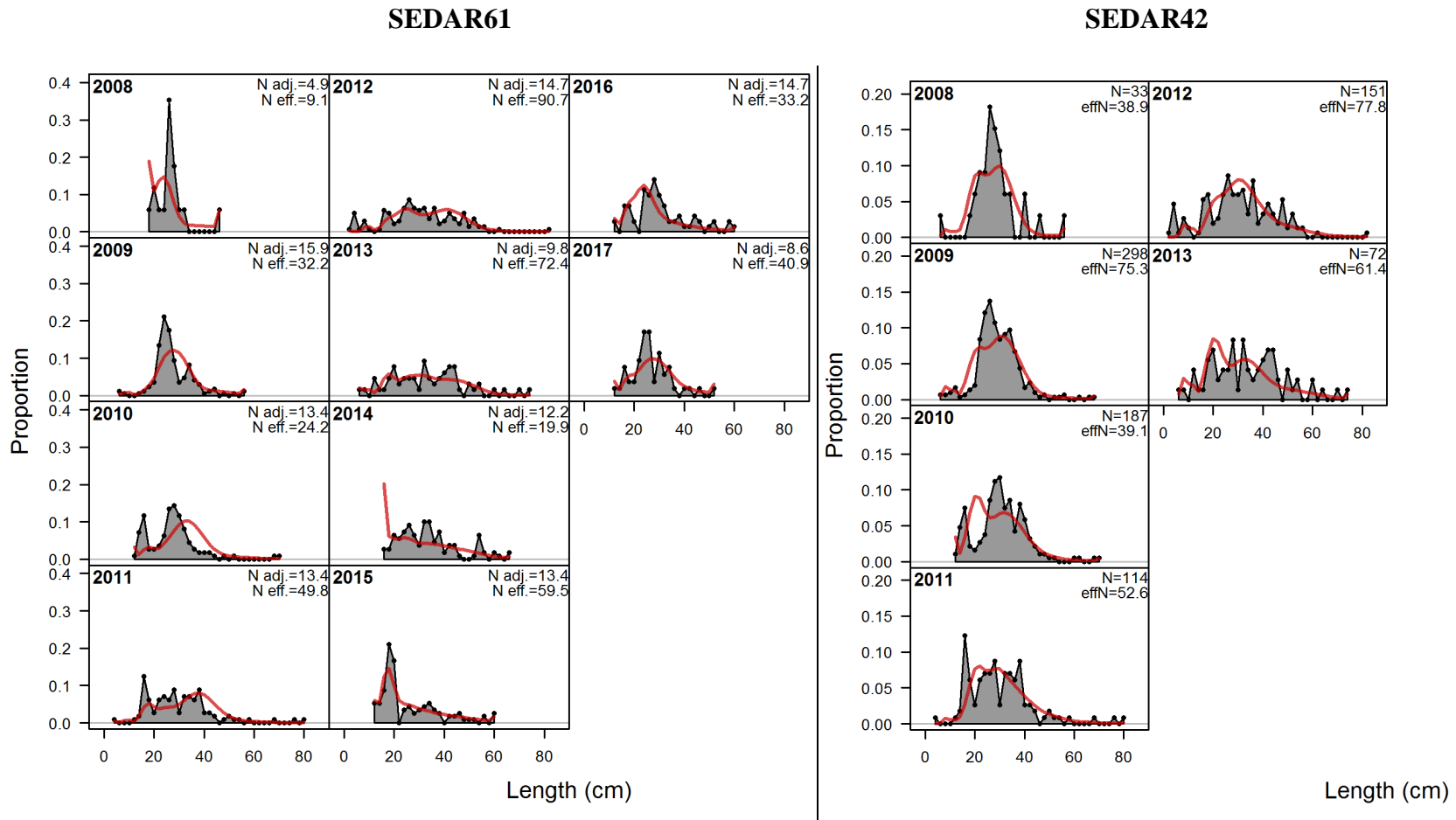
Figure 4.18. Model fits to the length composition of survey catch by the SEAMAP Summer Groundfish Survey for Gulf of Mexico Red Grouper. Red lines represent predicted length compositions, while grey shaded regions represent observed length compositions. The effective sample size used to weight the yearly length composition data is provided by N adj for SEDAR61 (left panel) and effN for SEDAR42 (right panel) and shown in the upper right corner of each panel.
