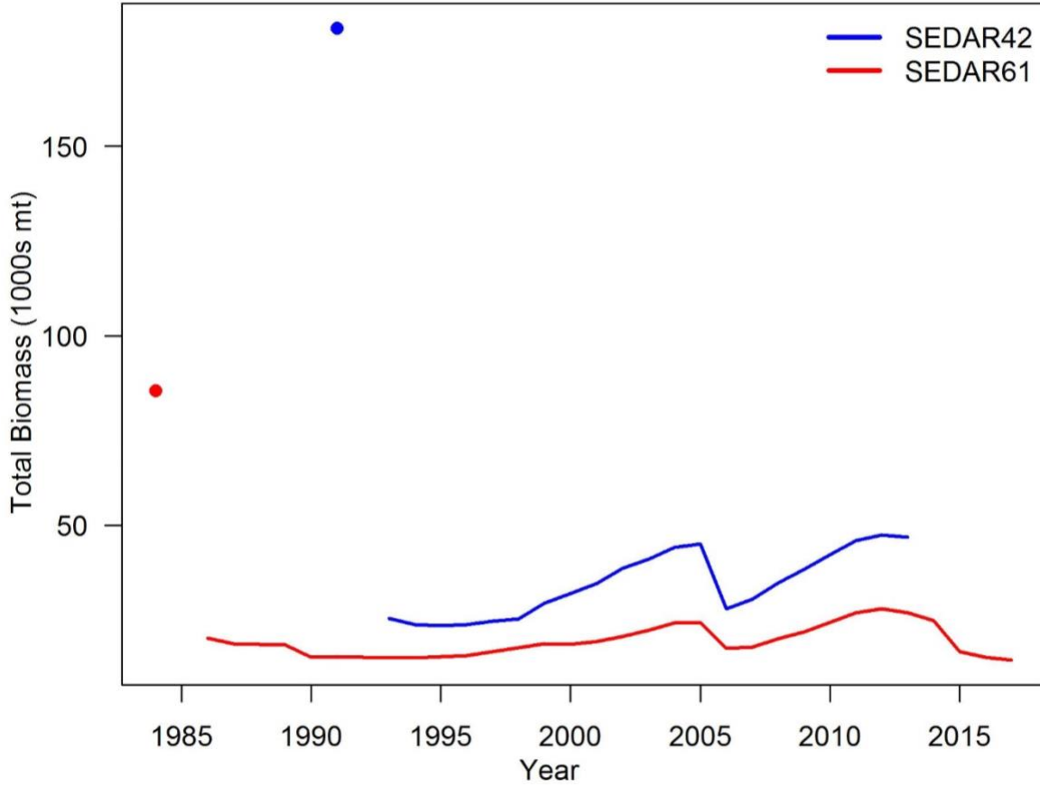
Figure 4.41. Estimates of total biomass (in 1000s of metric tons) of Gulf of Mexico Red Grouper. The solid circle is the estimated unfished equilibrium biomass.
