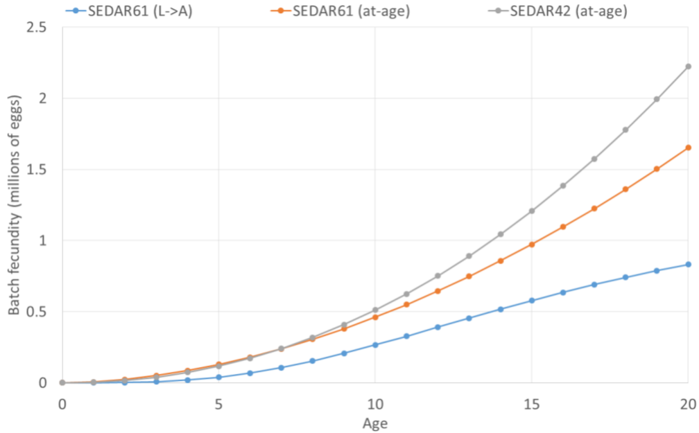
Figure 2.11. Comparison of batch fecundity-at-age for Red Grouper. The blue line reflects the recommended conversion of fecundity-at-length to fecundity-at-age using the growth curve for SEDAR61.
