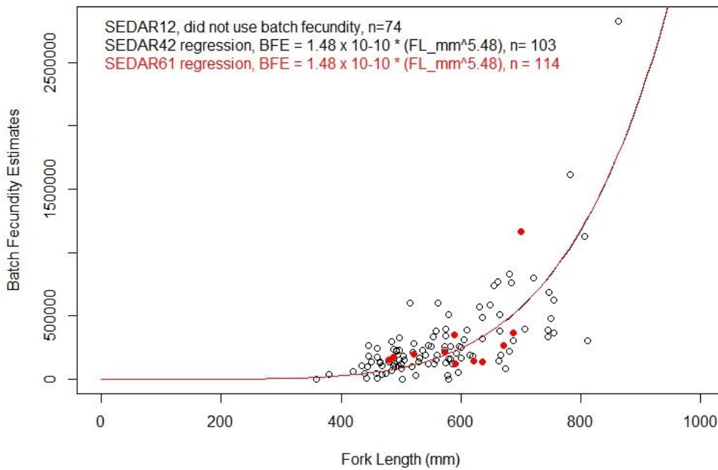
Figure 2.10. Batch fecundity by fork length for Red Grouper. Eleven new samples were obtained for SEDAR61 between 2014 and 2017 by NMFS Panama City.
