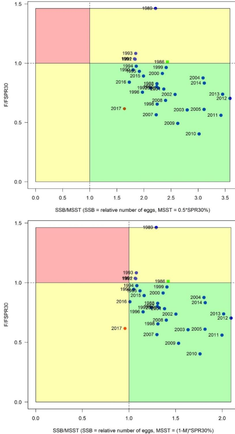
Figure 5.3. Kobe plot illustrating the time series of stock status of Gulf of Mexico Red Grouper in 2017 for the the SEDAR61 Base Model using the new definition of MSST ( 0.5 \cdot SSB_{SPR30\%} ; Upper Panel) and the old definition of MSST ( [1 - M] \cdot SSB_{SPR30\%} .) Lower Panel).
