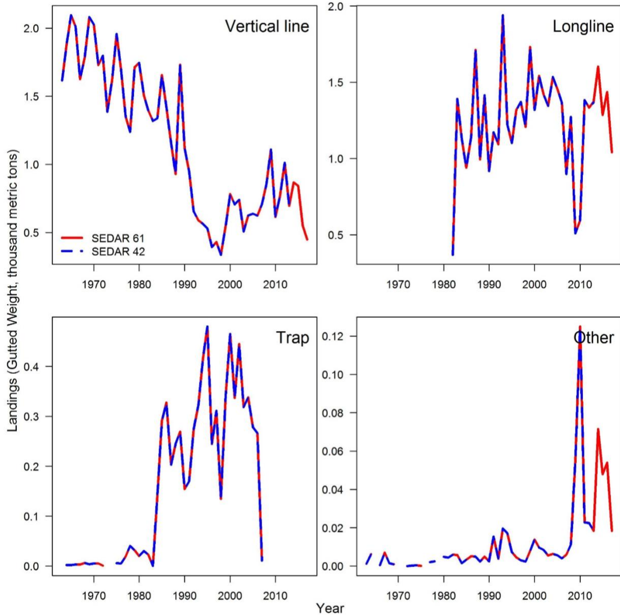
Figure 2.13. Commercial landings (guttled weight in thousands of metric tons) for the vertical line, longline, trap, and other fleets in the U.S. Gulf of Mexico. Note that the start year of the SEDAR61 Base Model is 1986.
