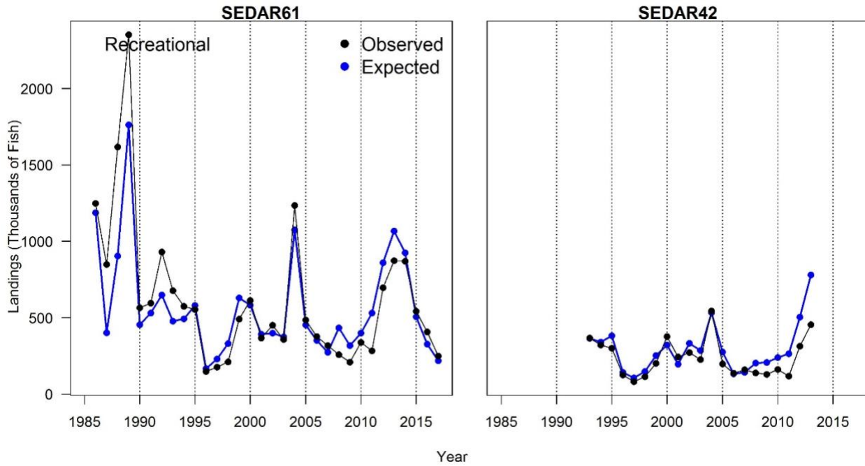
Figure 4.7. Gulf of Mexico Red Grouper observed and expected recreational landings for the recreational fleet in thousands of fish for SEDAR61 (left panel) and SEDAR42 (right panel). Dashed vertical lines identify five year intervals starting in 1990.
