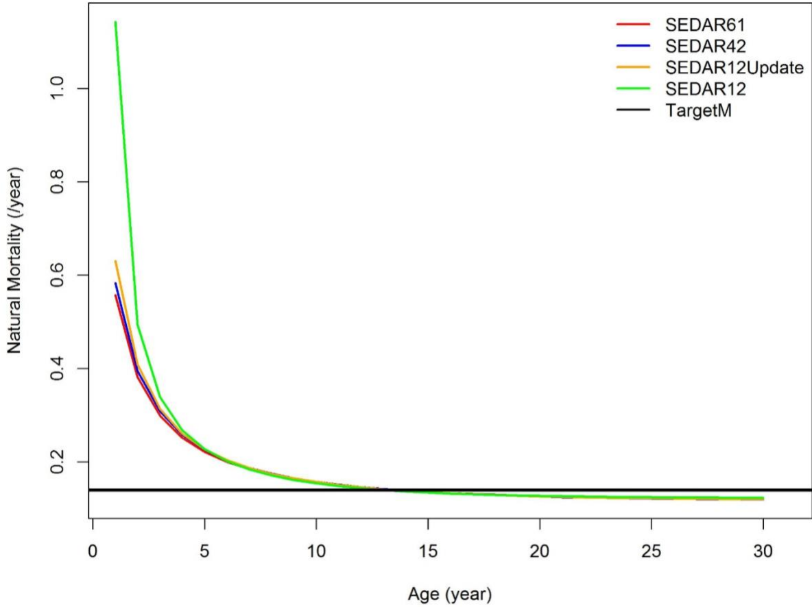
Figure 2.4. Comparison of age-specific natural mortality (M) vectors for Red Grouper from the northeastern Gulf of Mexico. Each vector was calculated using the same regression (Lorenzen 2005), age 5 as the first age at vulnerability, and a target M of 0.14 (Hoenig teleost , maximum age of 29 years; thick black line). The only difference among the age-specific natural mortality vectors was the predicted von Bertalanffy growth parameters used in the estimations.
