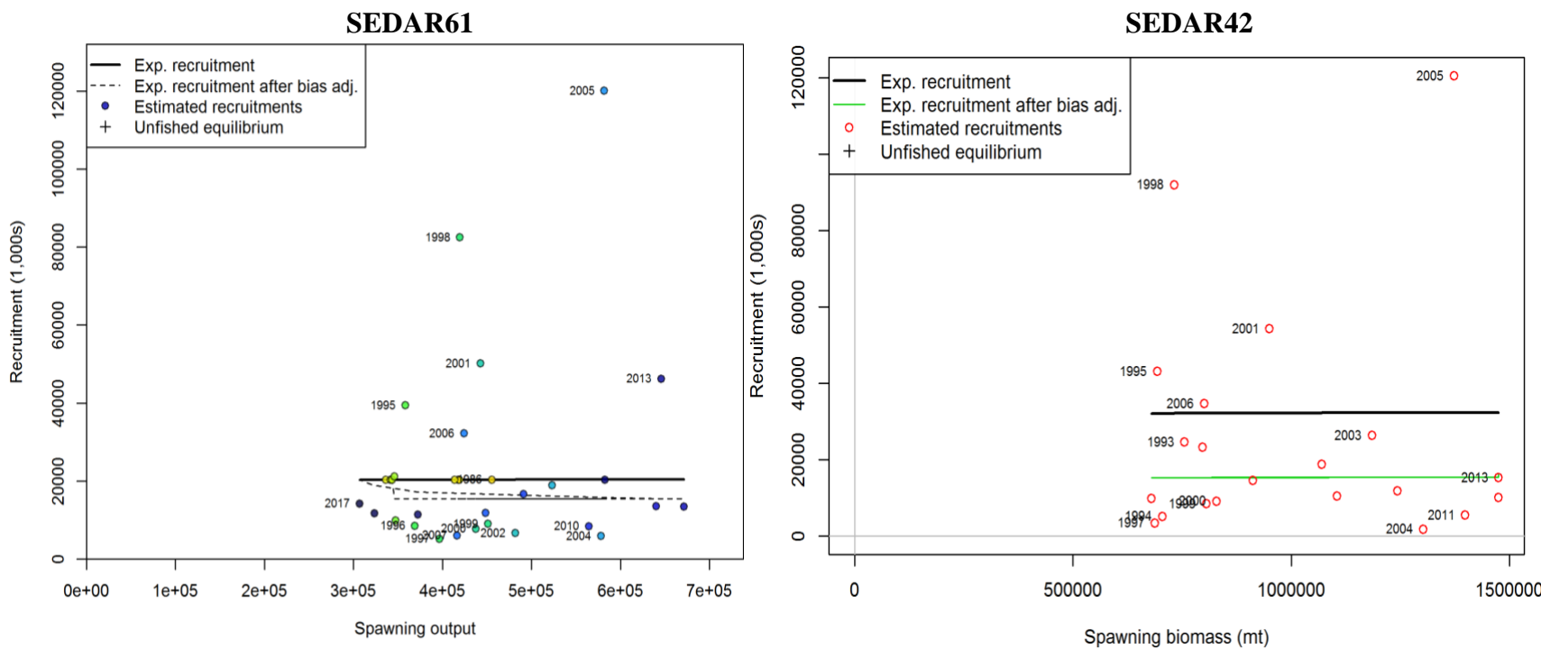
Figure 4.39. Predicted stock-recruitment relationship for Gulf of Mexico Red Grouper (steepness = 0.99, SigmaR estimated at 0.815). Plotted are predicted annual recruitments from Stock Synthesis (circles) and expected recruitment from the stock recruit relationship (black line). Labels are included on the first year, last year, and years with natural log deviations > 0.5. Results from SEDAR61 are presented in the left panel and those from SEDAR42 are presented in the right panel.
