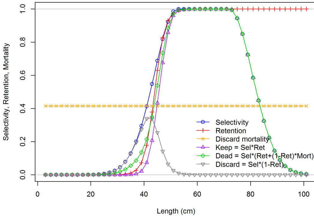
Figure 4.32. Terminal-year commercial longline fleet selectivity, retention, and discard mortality pattern.
