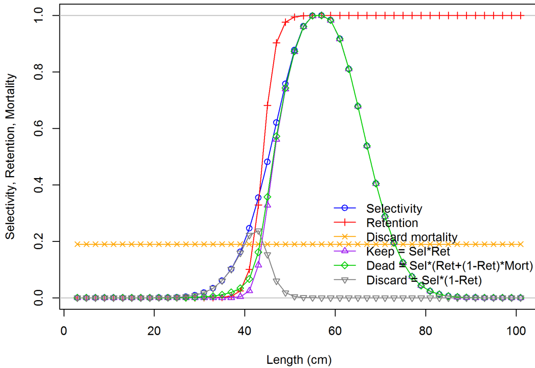
Figure 4.31. Terminal-year commercial vertical line fleet selectivity, retention, and discard mortality pattern.
