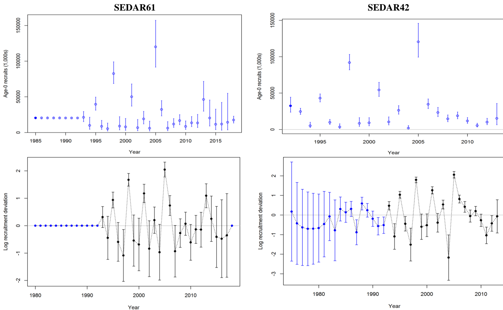
Figure 4.40. Estimated Age-0 recruitment with 95% confidence intervals and log recruitment deviations (1993-2017) for Gulf of Mexico Red Grouper (steepness = 0.99, \sigma_R estimated at 0.815). Results from SEDAR61 are presented in the left panels and those from SEDAR42 are presented in the right panels.
