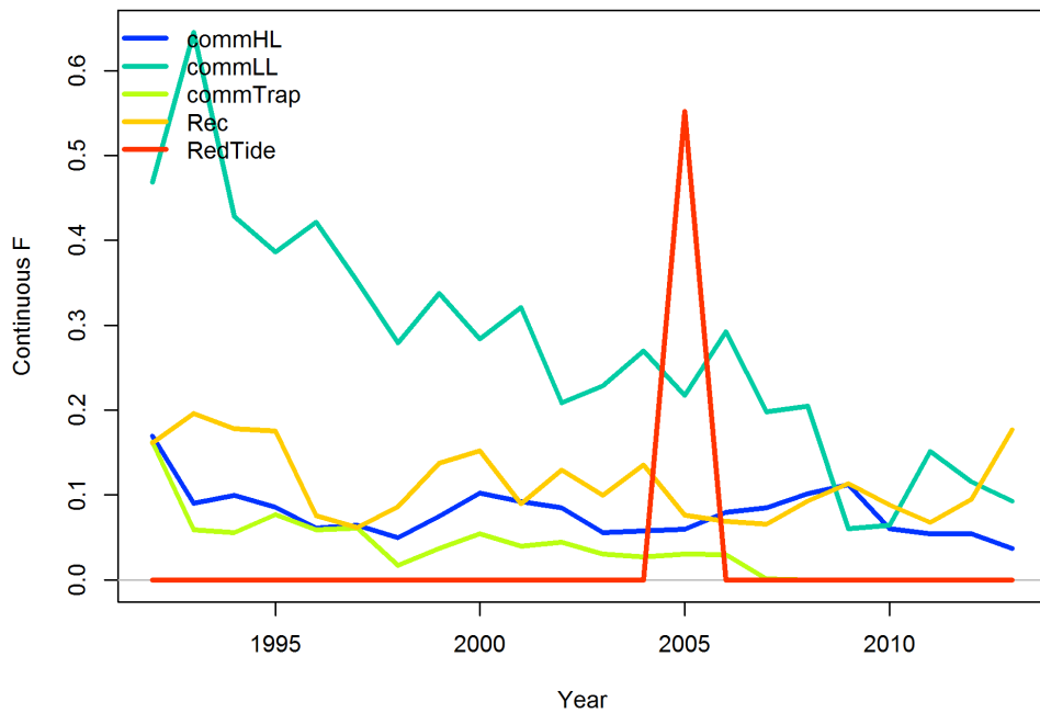
Figure 4.45. Fleet-specific apical fishing mortality rates for Gulf of Mexico Red Grouper for SEDAR61 (Upper Panel) and SEDAR42 (Lower Panel). This represents the instantaneous fishing mortality level on the most vulnerable age class for each fleet.
