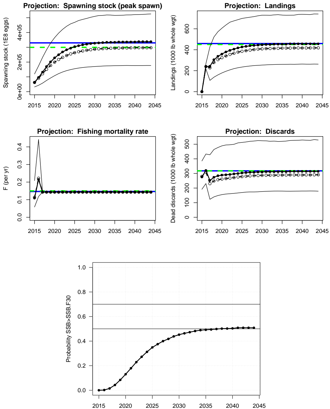
Figure 60. Projection results under scenario 5—fishing mortality rate at F = F_{rebuild} , with rebuilding probability of 0.5 in 2044. In top four panels, expected values (base run) represented by solid lines with solid circles, medians represented by dashed lines with open circles, and uncertainty represented by thin lines corresponding to 5 th and 95 th percentiles of replicate projections. Solid horizontal lines mark F_{30\%} -related quantities; dashed horizontal lines represent corresponding medians. Spawning stock (SSB) is at time of peak spawning. In bottom panel, the curve represents the proportion of projection replicates for which SSB has reached the replicate-specific SSB_{F30\%} .
