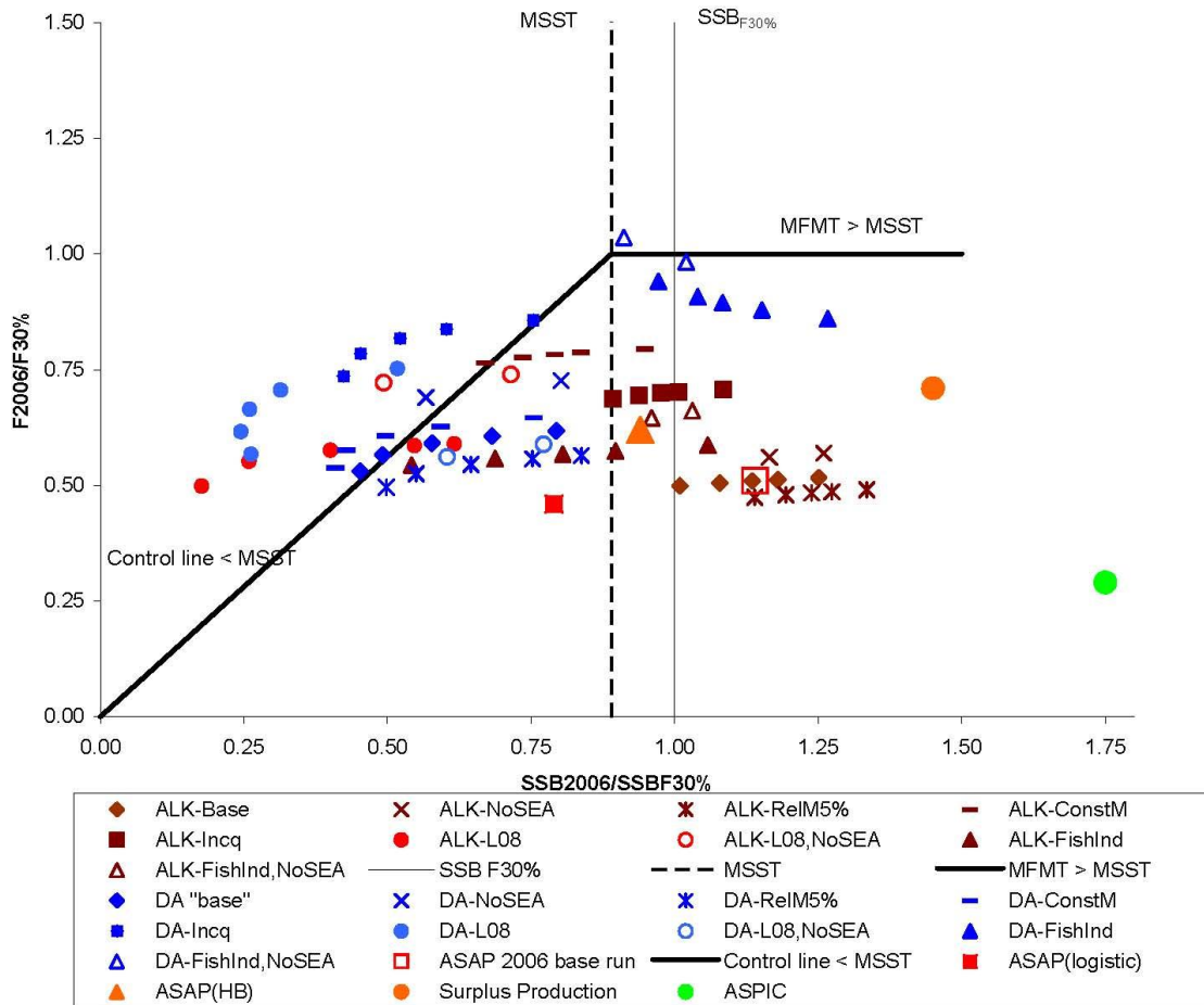
Figure 1. Comparison of ASAP model run configurations and results against fishery benchmarks. Results from additional sensitivity runs requested by the Review Panel using an asymptotic selectivity pattern for the different fisheries, a configuration using a new index for the Headboat Survey for the 1981-2006 time period (rather than a split time series for this index), and benchmark values from the Surplus Production and ASPIC models are plotted along with the ASAP benchmarks from the mutton snapper stock assessment.
