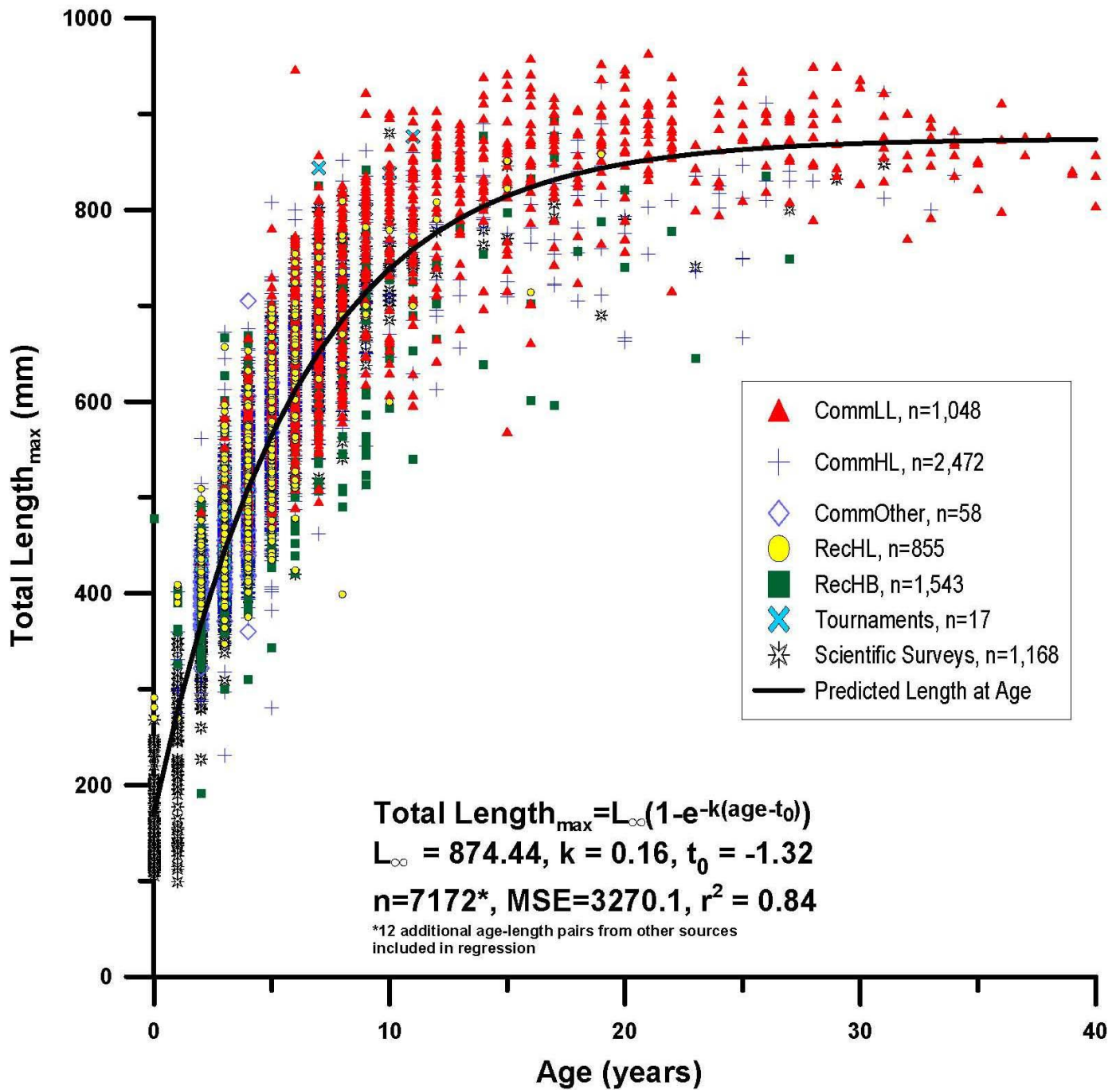
Figure 2.10. Total length ( TL_{max} , mm) at age and estimated size at age from von Bertalanffy (1938) growth function of the current study.
