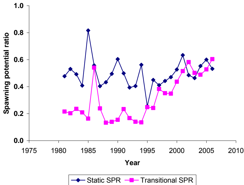
Figure 2.5.1. a) Yield-per-recruit, spawning potential ratio, and the SPR = 30% limit from the base run that had a steepness of 0.75 and age-specific natural mortality averaging 0.11 per year for ages 3-40. F_{MAX} was at 0.52 per year and F_{30\%} was 0.34 per year. b) Static and transitional spawning potential ratios by year from the base run.
