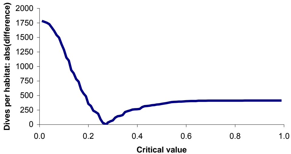
Figure 5.13. The absolute differences between false positive and false negative dives per habitat for juvenile mutton snapper for each critical value from the Stephens and MACAll method.
