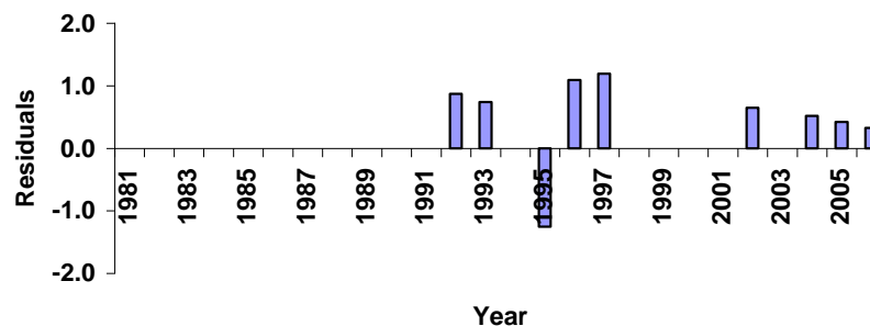
Figure 2.3.1.3.3 continued. Fit of ASAP model to the 11 relative indices of abundance. Each index is scaled to its mean such that a value of 1.0 is equal to the mean of the index. The indices included in this model were: FWC Visual survey for exploited ages, FWC Visual survey of pre-exploited ages, FWC Fishery Independent Monitoring haul seine sets, NMFS-UM Reef visual census, NMFS Riley's Hump visual survey, SEAMAP Video survey, NMFS MRFSS total catch index, NMFS Logbook hook-and-line, NMFS Logbook longline, NMFS Headboat survey 1981-1991, and NMFS Headboat 1995-2006.
